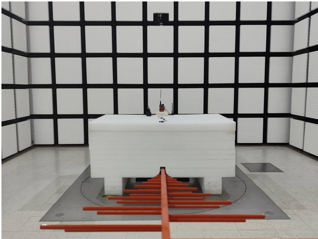
Radiated Emission Below 1GHz Rear View M2&M3
