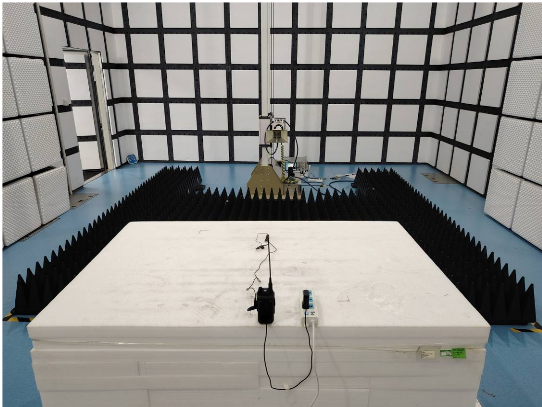
Radiation Emission_ Above 1GHz - Rear View (Mode 1)
