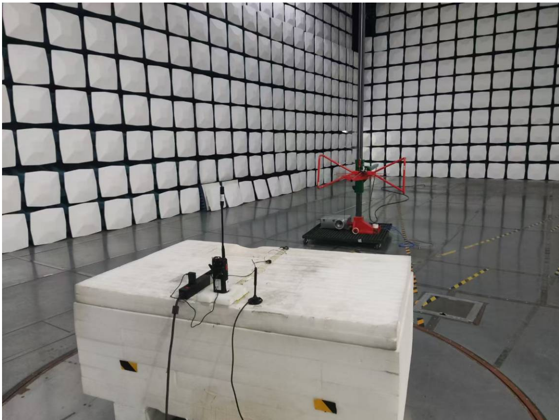
Radiated Emission 30M-1GHz Rear View
