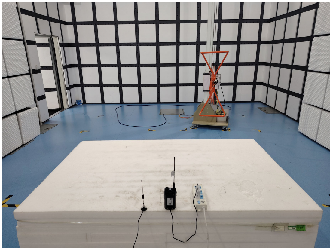
Radiated Emission - Back View (Below 1GHz)
