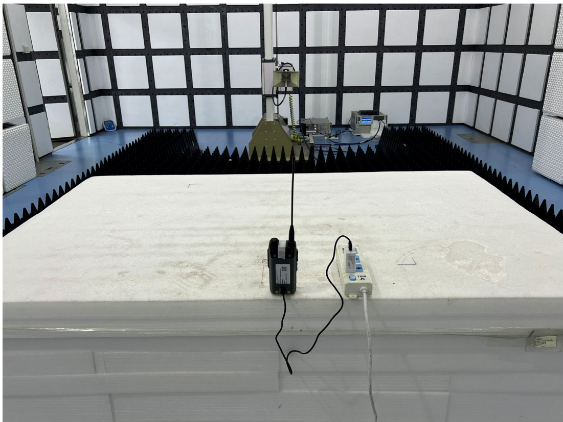
Radiated Emission - Back View (Above 1GHz)
