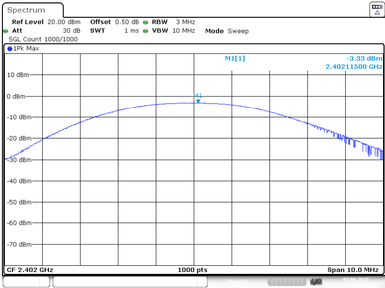
1Mbps_Lowest
