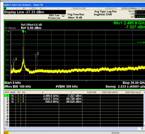
802.11g-High channel
