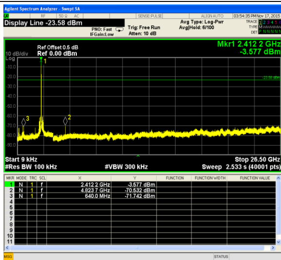
802.11b-Low channel
