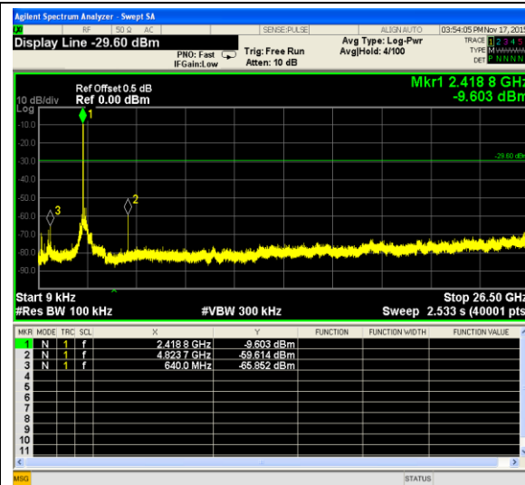
802.11g-Low channel
