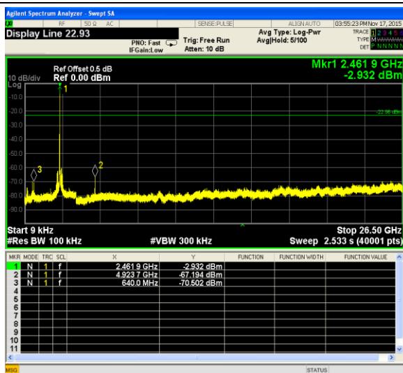
802.11b-High channel
