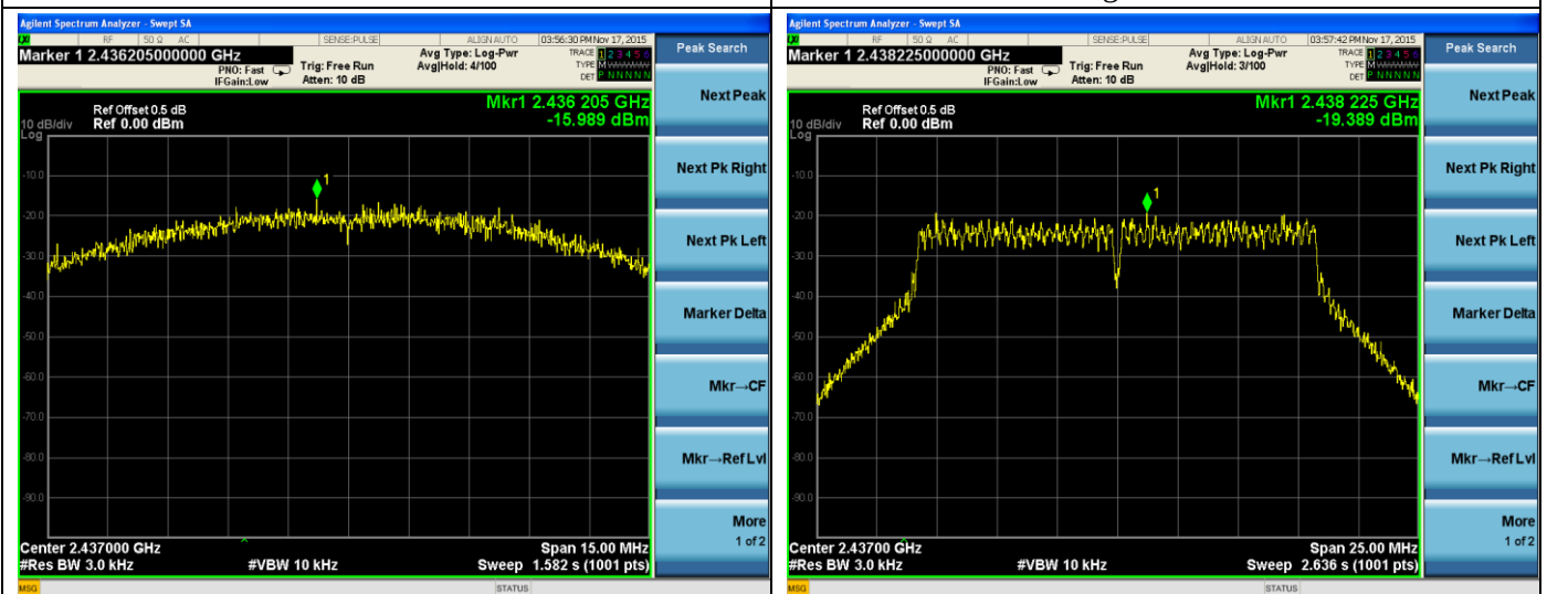
802.11b-Middle channel
