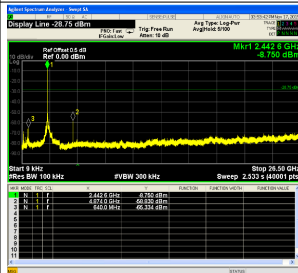
802.11g-Middle channel
