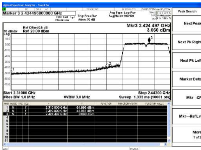
802.11n(HT40)-Low channel(Peak)
