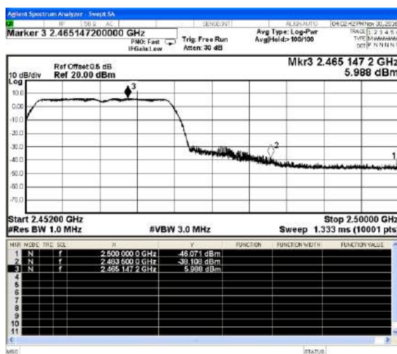
802.11n(HT20)-High channel(Peak)
