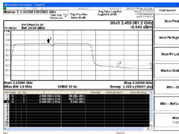
802.11n(HT40)-High channel(Average)
