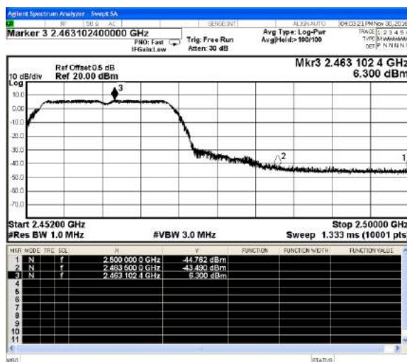
802.11g-High channel(Peak)
