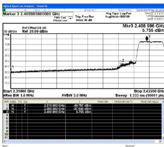
802.11n(HT20)-Low channel(Peak)
