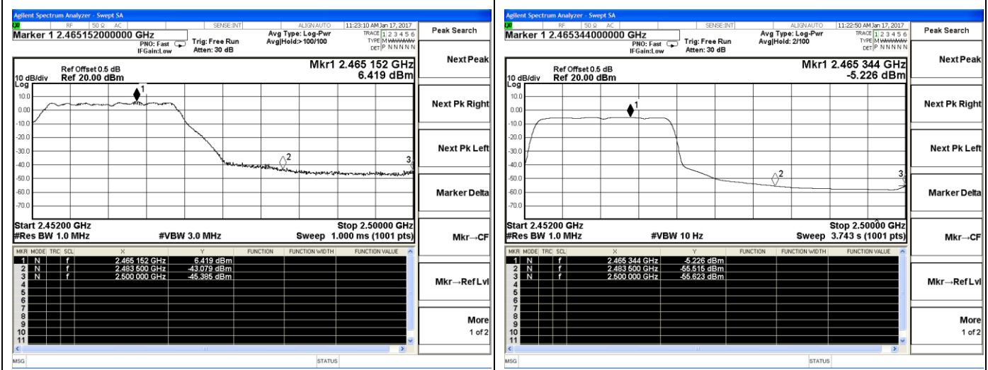
802.11g Chain 0-High channel(Peak)
