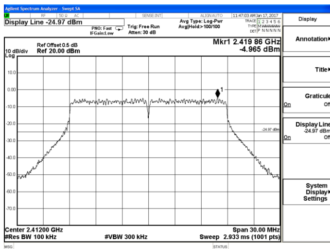
802.11n-HT20 Chain 1-Low channel Reference
