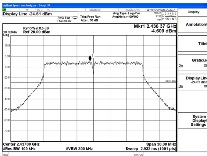
802.11n-HT20 Chain 1-Middle channel Reference
