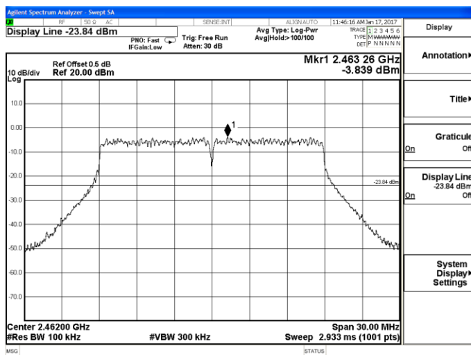
802.11n-HT20 Chain 1-High channel Reference
