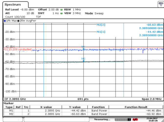
Figure 8.3-6: Conducted spurious emission at band edge of restricted band, low channel
