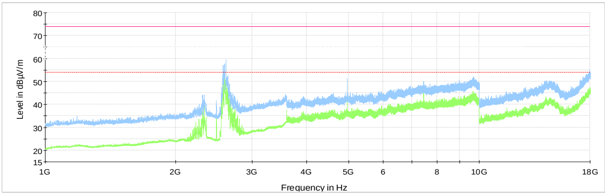
Figure 8.3-10: Radiated spurious emissions 1 to 18 GHz, High channel
