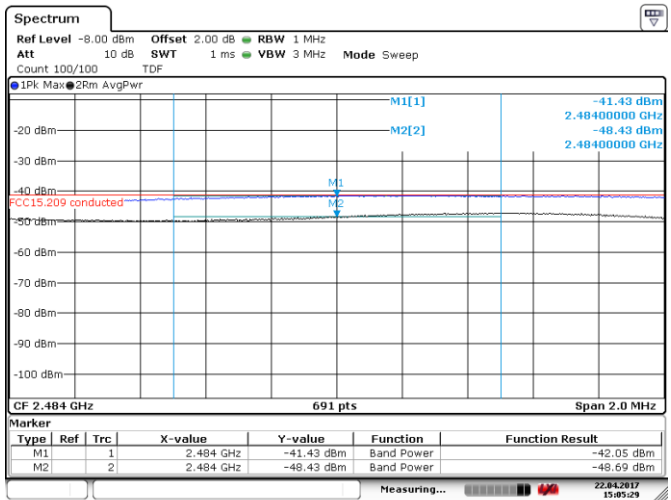
Figure 8.3-7: Conducted spurious emissions at band edge of restricted band, High channel
