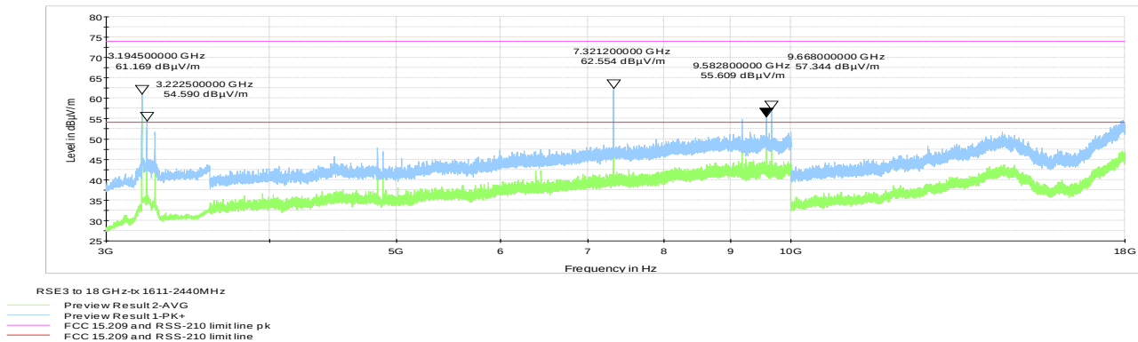
Figure 8.3-18: Radiated spurious emissions 3 to 18 GHz, Tx on mid channel, Globalstar Radio at 1611 MHz
