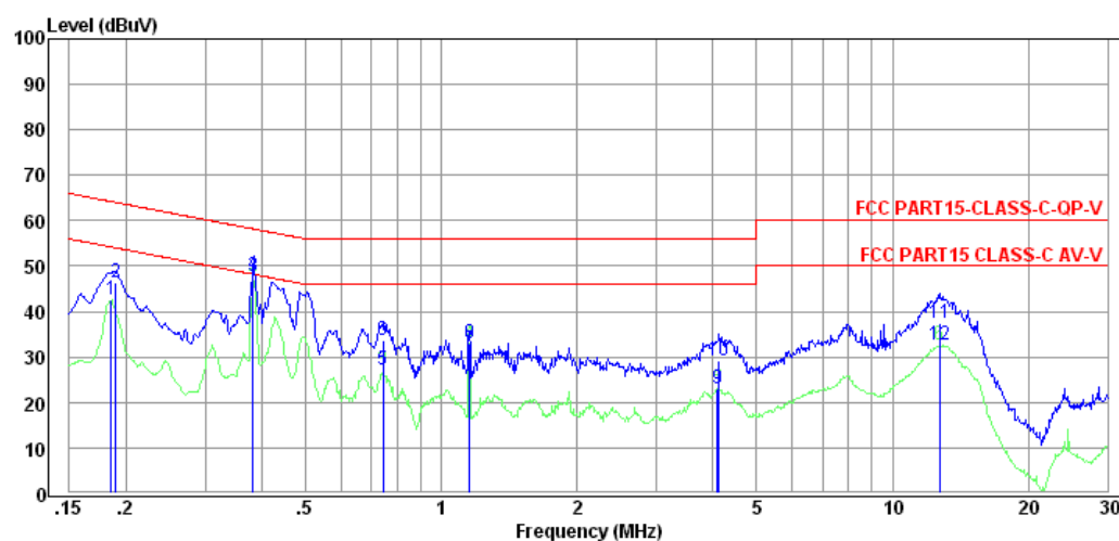
ANT1-L Line
