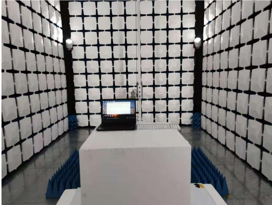
Model: DF22 Above 1GHz for radiated emission test setup
