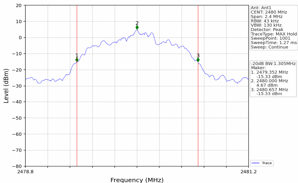
Pi/4DQPSK_2DH5_HCH_2480MHz_Ant1_NTNV
