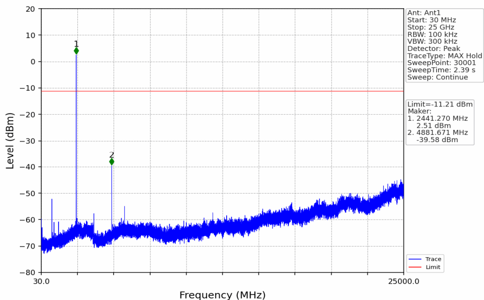
Pi/4DQPSK_2DH5_MCH_2441MHz_Ant1_NTNV
