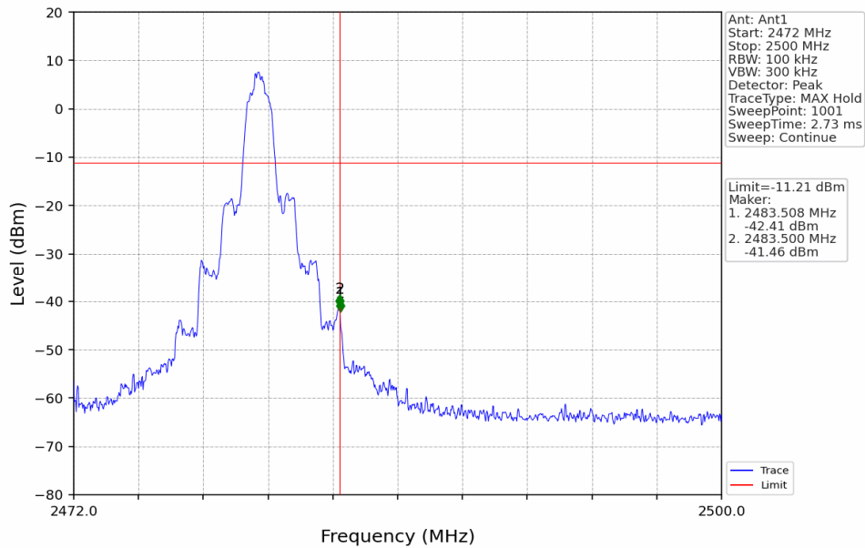
Pi/4DQPSK_2DH5_HCH_2480MHz_Ant1_NTNV
