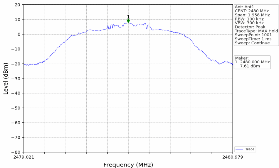
Pi/4DQPSK_2DH5_HCH_2480MHz_Ant1_NTNV
