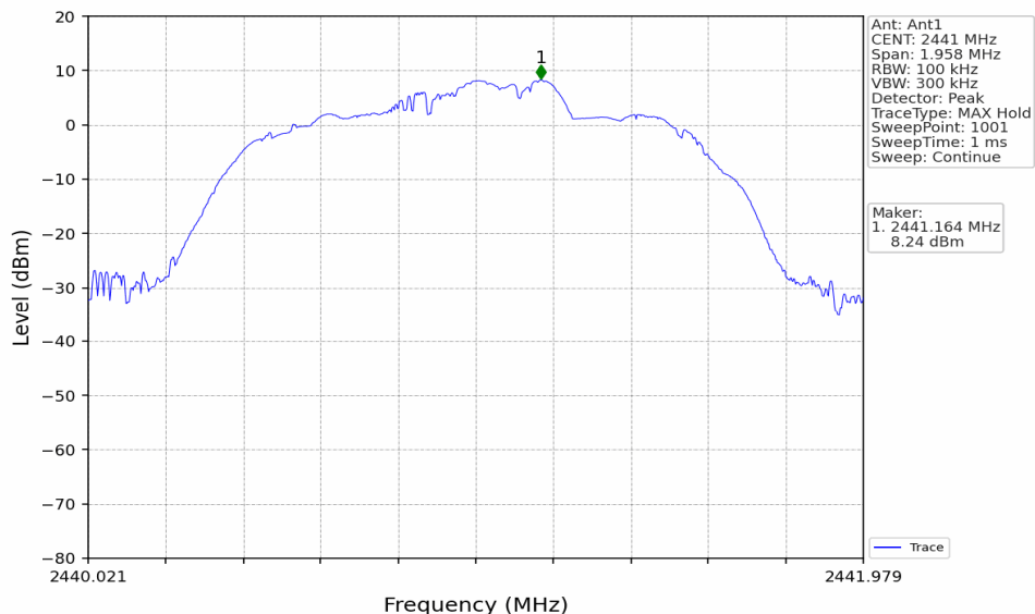
8DPSK_3DH5_MCH_2441MHz_Ant1_NTNV
