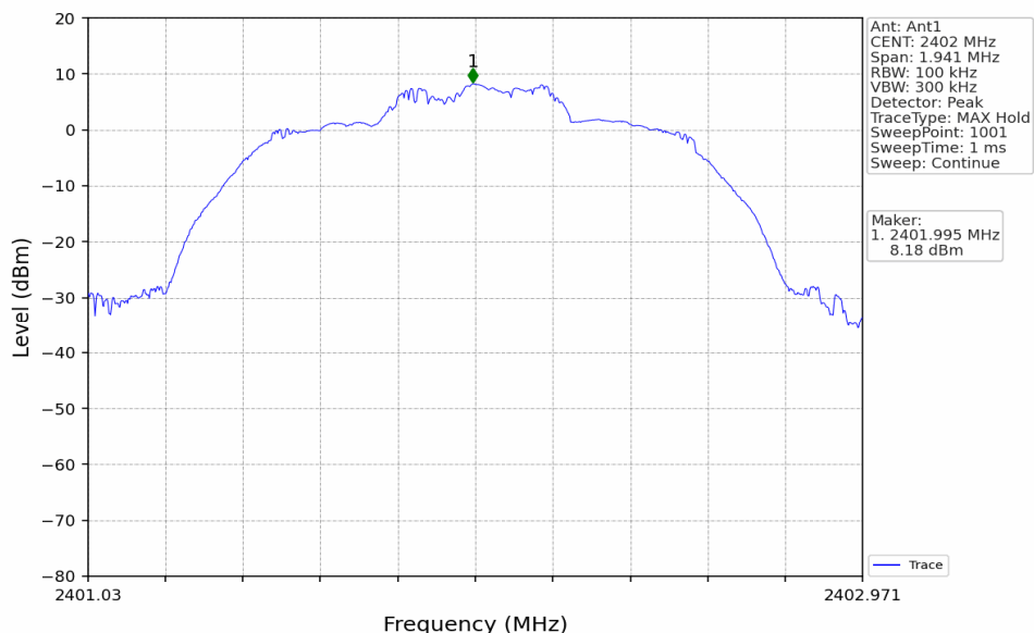
Pi/4DQPSK_2DH5_LCH_2402MHz_Ant1_NTNV
