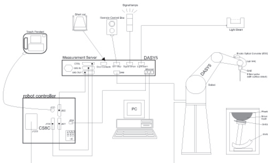
F-1. SAR Measurement System Configuration
