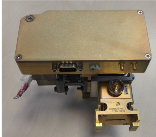
RF Detector
