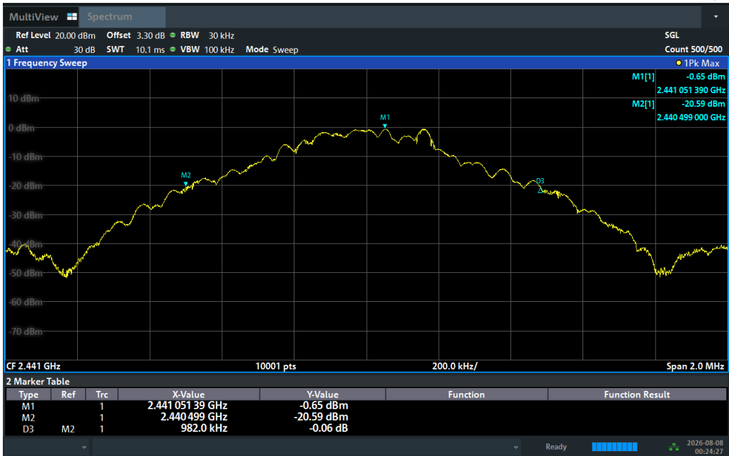
TX CH39
