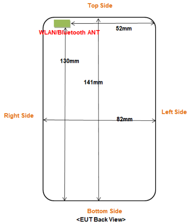
Fig 7.2 Block Diagram for EUT Antenna Position
