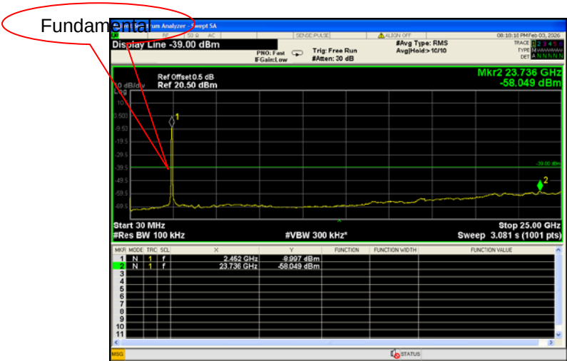
Mode: TX 11 n HT40 channel 9
