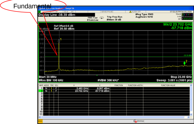
Mode: TX 11g channel 11
