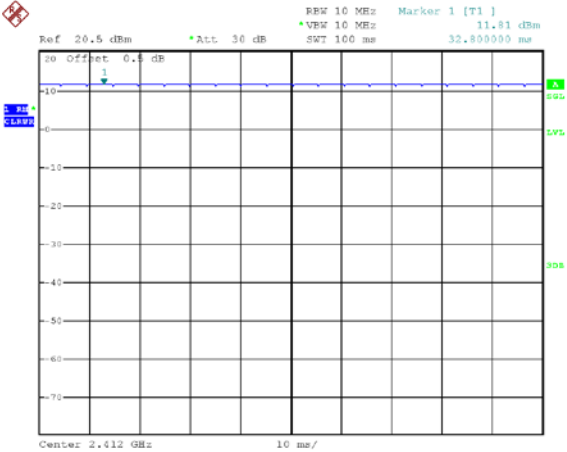
Wi-Fi 802.11n-HT20
