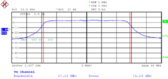
Mode: TX 11g channel 6
