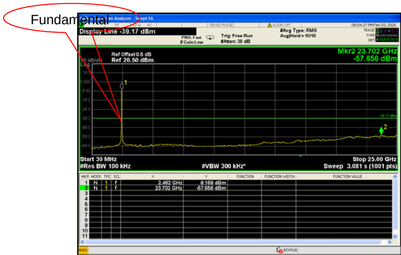
Mode: TX 11 n HT20 channel 11
