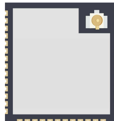
ESP32-S3-WROOM-1U
