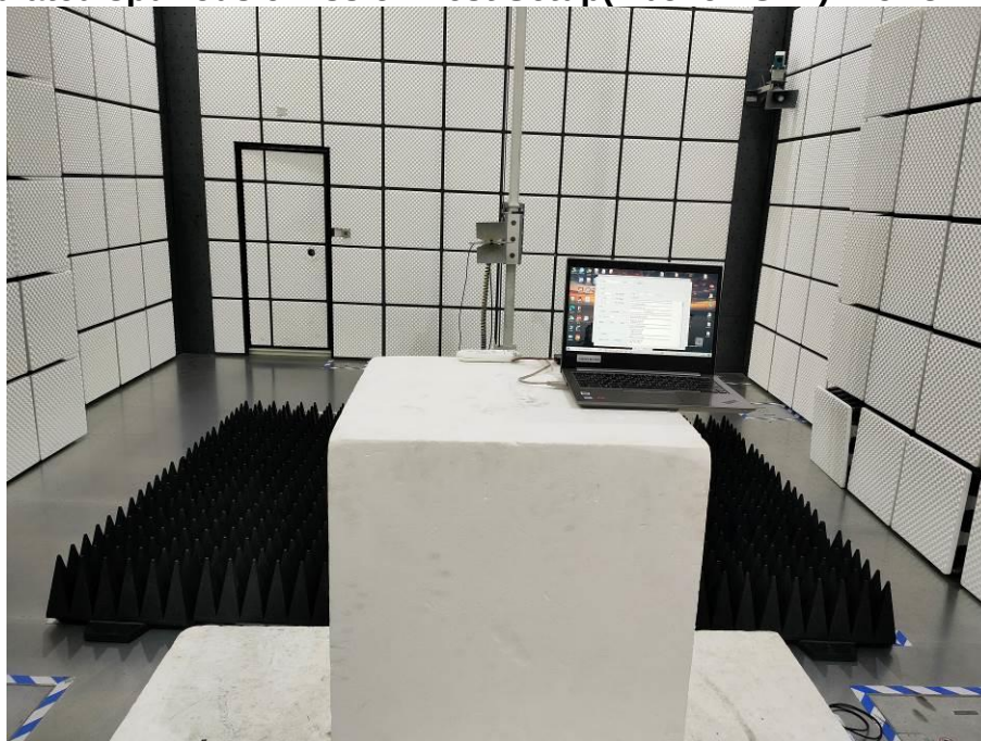
Radiated spurious emission Test Setup(Above 1GHz)- HJH82B Ble
