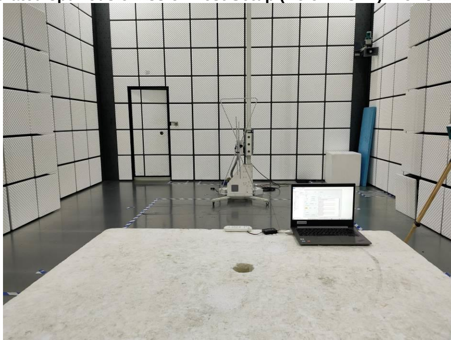
Radiated spurious emission Test Setup (Below 1GHz)- HJH82B Ble
