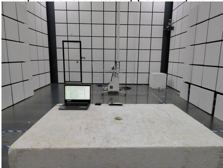
Radiated spurious emission Test Setup (Below 1GHz)-- HJH92B Ble
