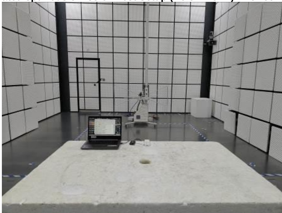
Radiated spurious emission Test Setup (Below 1GHz)-- HJH55BA Ble
