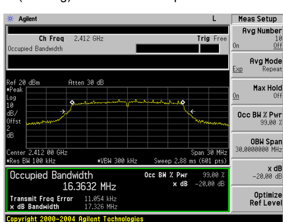
(802.11g) -20dB Bandwidth plot on channel 1
