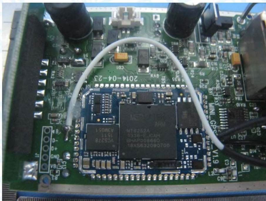
Photo 10 Appearance of Antenna
