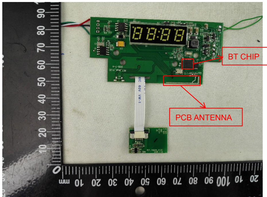
EUT UNCOVER VIEW 3
