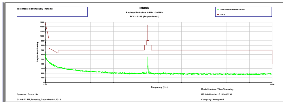
Radiated Emissions 9 kHz - 30 MHz, Antenna: Perpendicular (Worst case)
