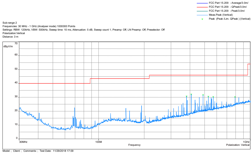
Radiated Emissions 30 MHz – 1GHz, Antenna: Vertical
