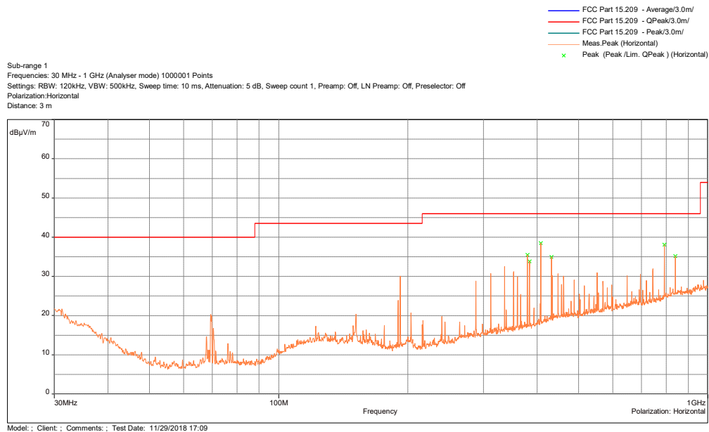
Radiated Emissions 30 MHz – 1GHz, Antenna: Horizontal
