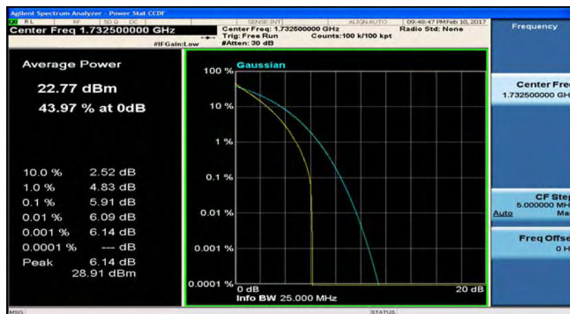
(LTE band 4_Channel Bandwidth:15 MHz)_MCH_QPSK_37RB#38
