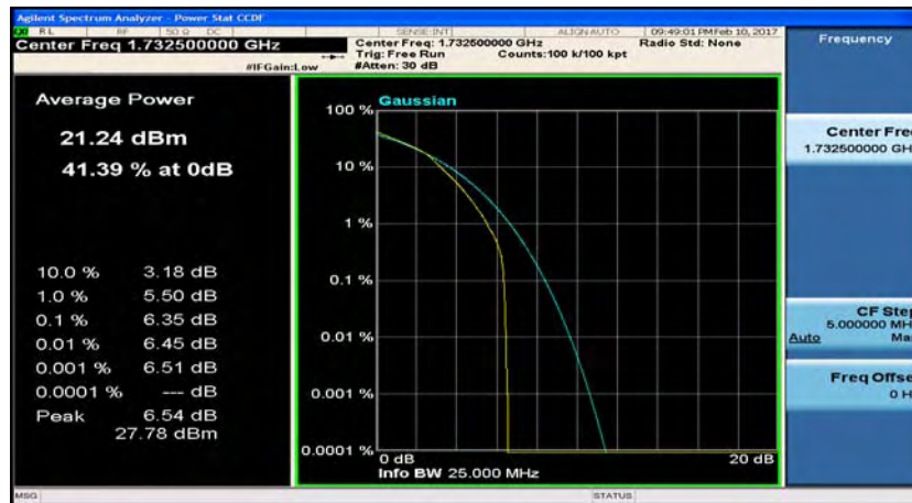
(LTE band 4_Channel Bandwidth:15 MHz)_MCH_16QAM_37RB#18
