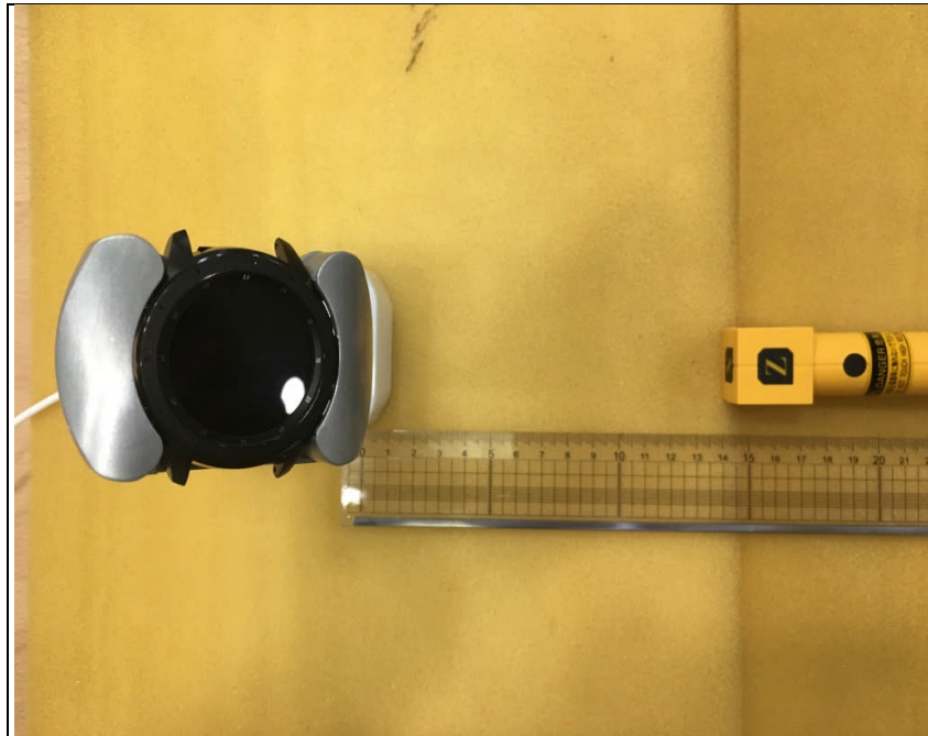
Photo of MPE Test Set up (E-field)
