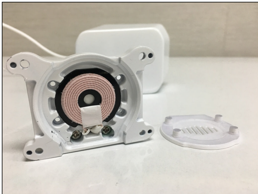
Internal Bottom view of EUT
