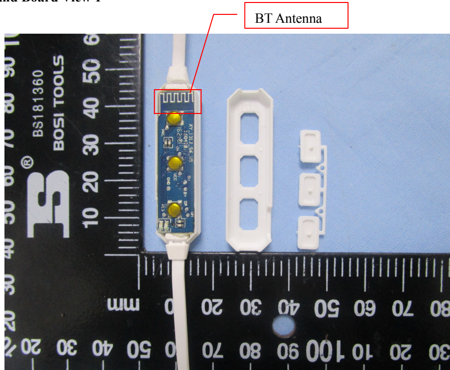
EUT Housing and Board View 1
