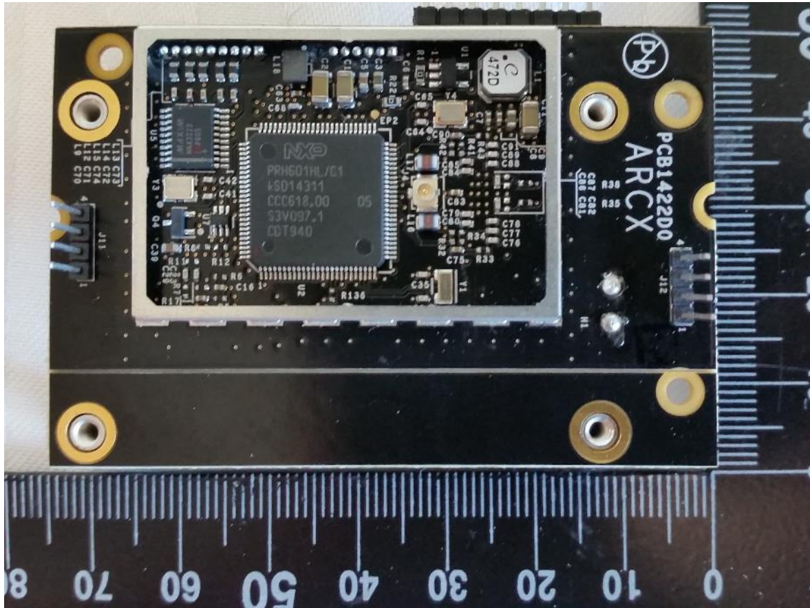
Figure 2 – EUT Internal Photo Top (Without the Shield)
