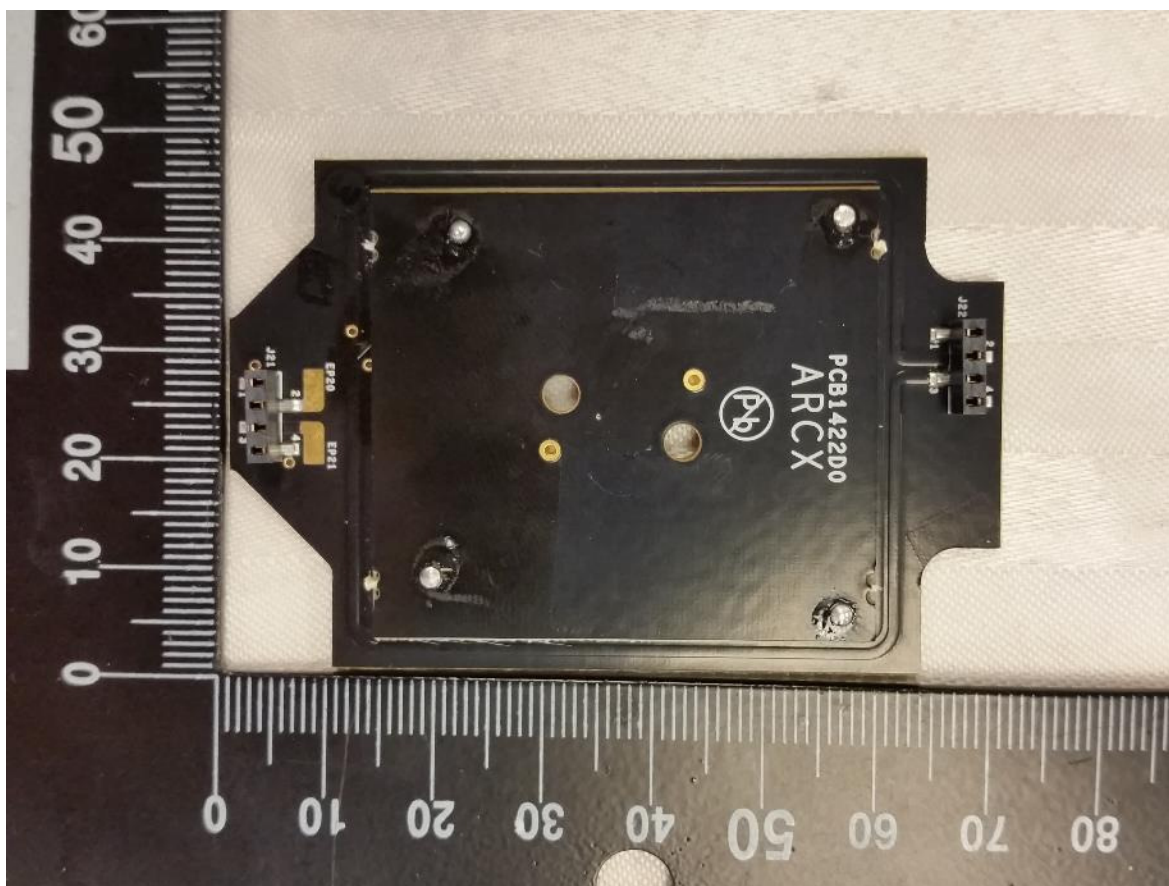
Figure 5 – EUT's Custom Loop Antenna - Top
