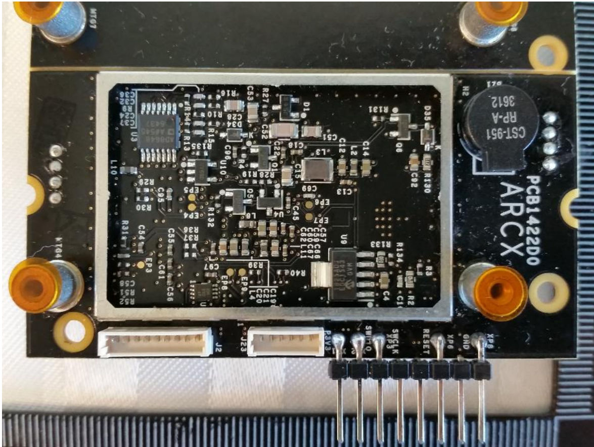
Figure 4 – EUT Internal Photo Bottom (Without the Shield)
