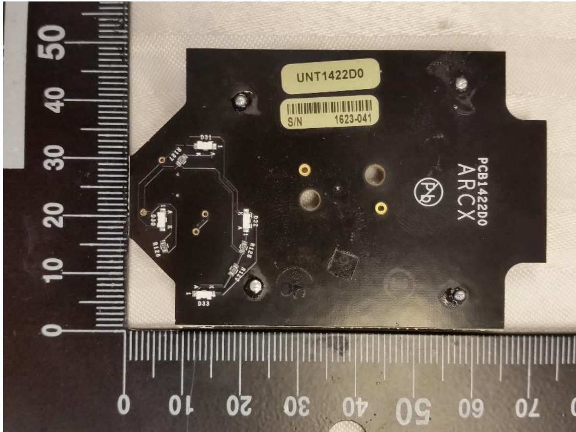
Figure 6 – EUT's Custom Loop Antenna - Bottom
