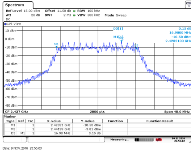
Figure 8.1-17: 6 dB bandwidth, 20MHz BW OFDM/QAM16 MCS4
