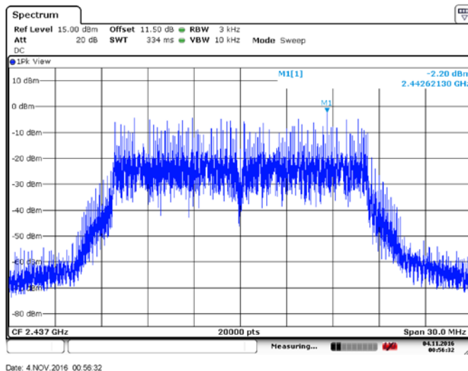
Figure 8.4.5: Conducted spurious emissions, 2437MHz, 20MHz BW, OFDM/Mbps48
