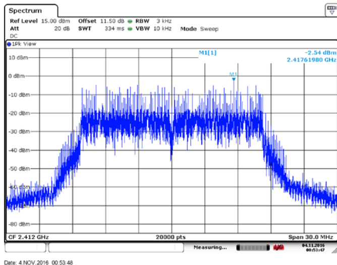
Figure 8.4.4: Power Spectrum Density, 2412MHz, 20MHz BW, OFDM/Mbps48
