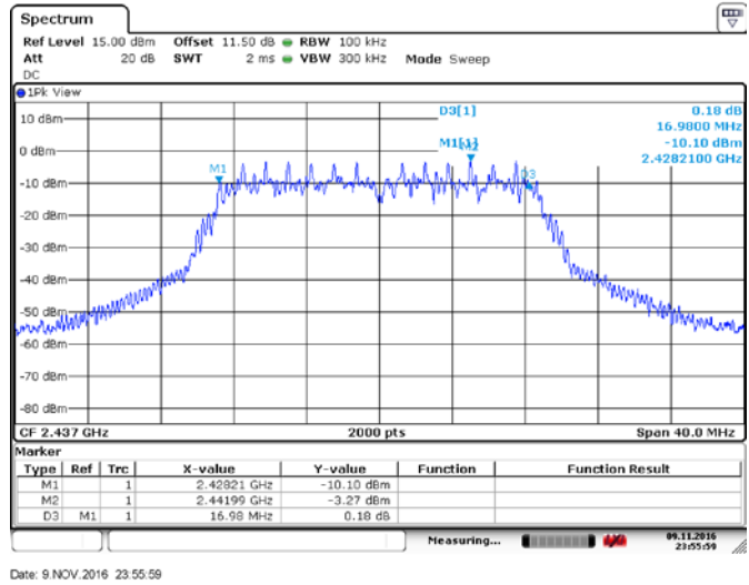
Figure 8.1-18: 6 dB bandwidth, 20MHz BW OFDM/QAM64 MCS5
