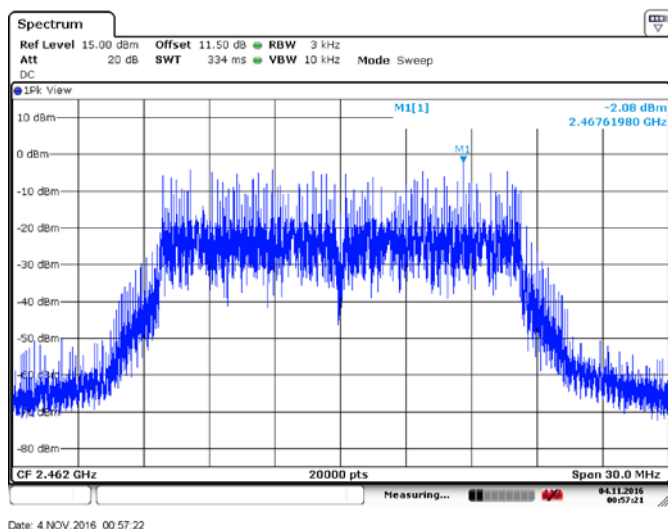
Figure 8.4.6: Power Spectrum Density, 2462MHz, 20MHz BW, OFDM/Mbps48
