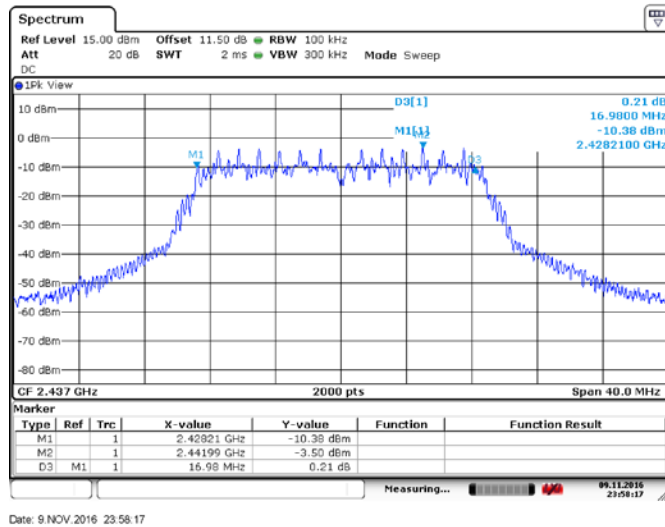
Figure 8.1-19: 6 dB bandwidth, 20MHz BW OFDM/QAM64 MCS6
