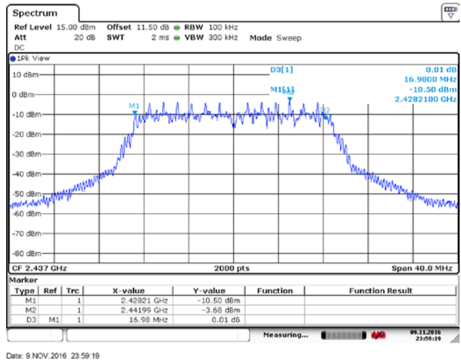
Figure 8.1-20: 6 dB bandwidth, 20MHz BW OFDM/QAM64 MCS7
