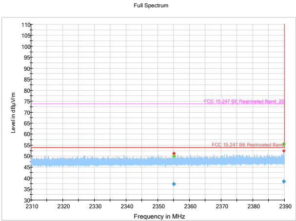
Figure 8.3.47: Radiated Band Edge, 2412MHz, 20MHz BW, DSSS/Mbps5.5
