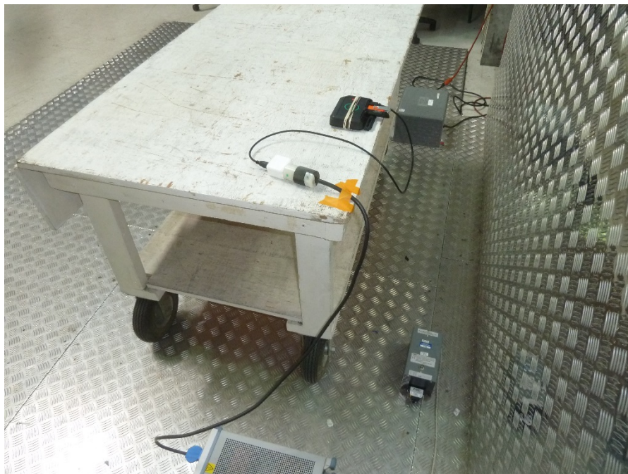
Figure 8.1-3: Clause 8.4 – AC mains power input/output ports setup photo
