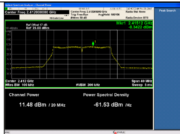
11g-PSD-Low-TX2
