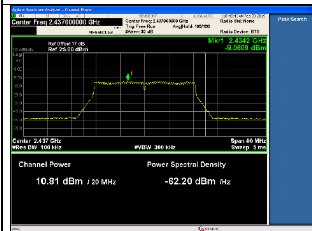
11g-PSD-Mid-TX1
