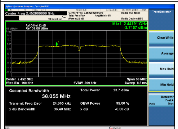
11n-40MHz-6dB BW-High
