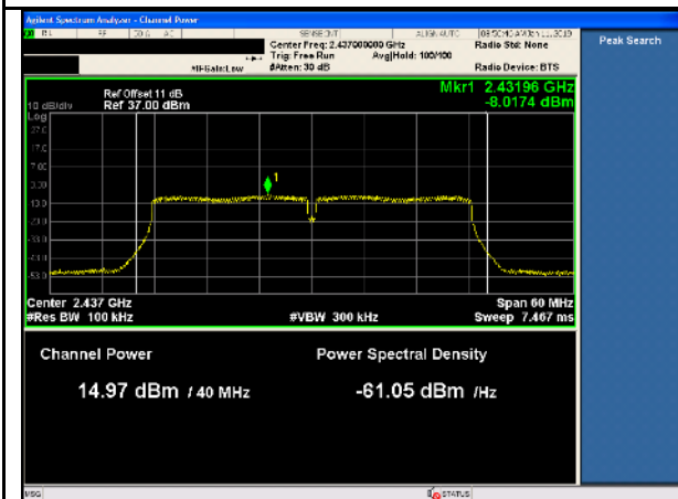
11n-40MHz-PSD-Mid-TX1
