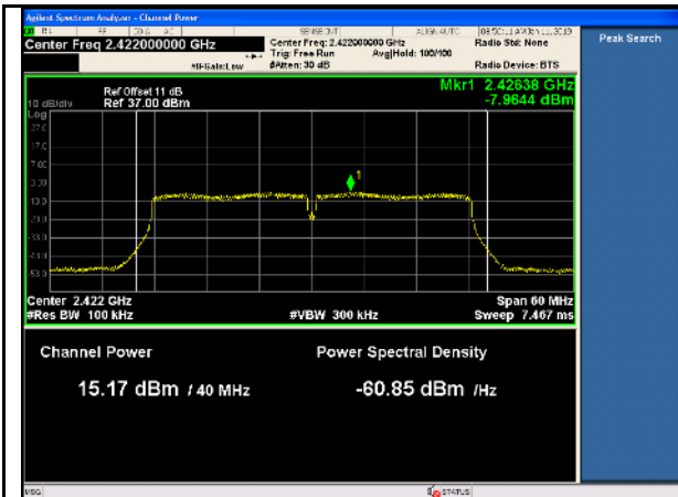
11n-40MHz-PSD-Low-TX1
