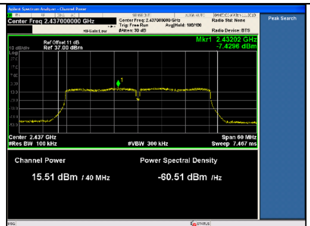
11n-40MHz-PSD-Mid-TX2
