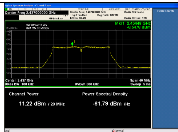
11g-PSD-Mid-TX2
