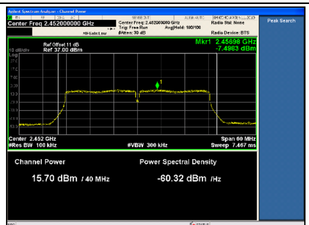
11n-40MHz-PSD-High-TX2
