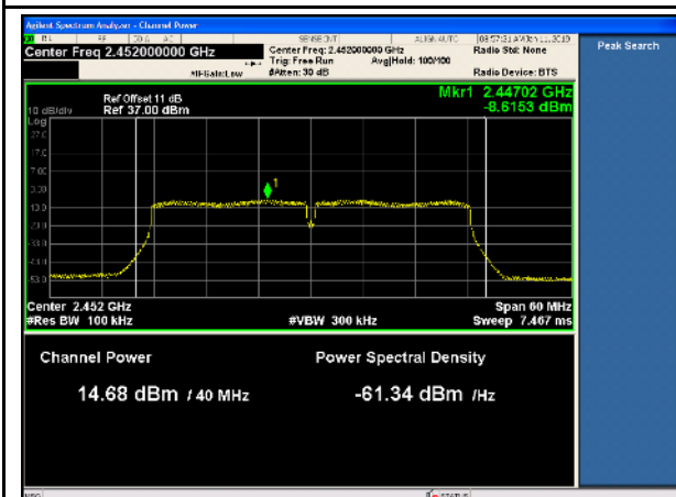
11n-40MHz-PSD-High-TX1
