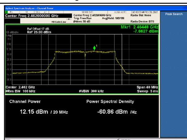
11g-PSD-High-TX2
