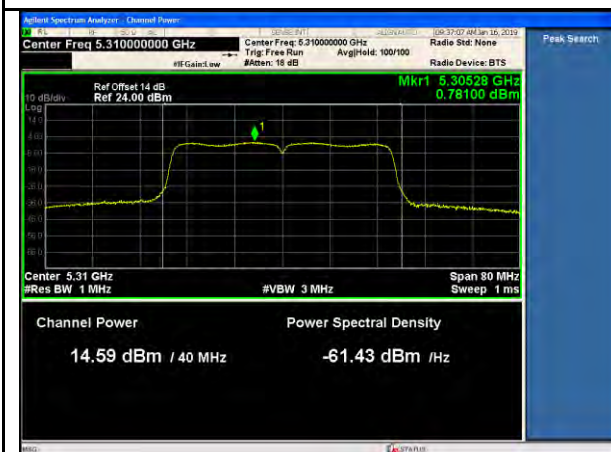
802.11n-40MHz- 5310MHz-PWR-TX1
