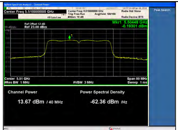
802.11n-40MHz- 5510MHz-PWR-TX2
