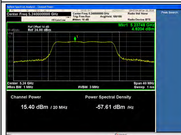
802.11a 5240MHz-PWR-TX1
