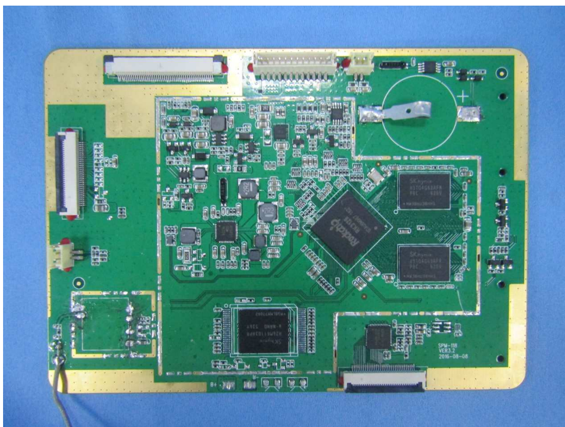
Control PCB view(Remove WIFI and BT module)
