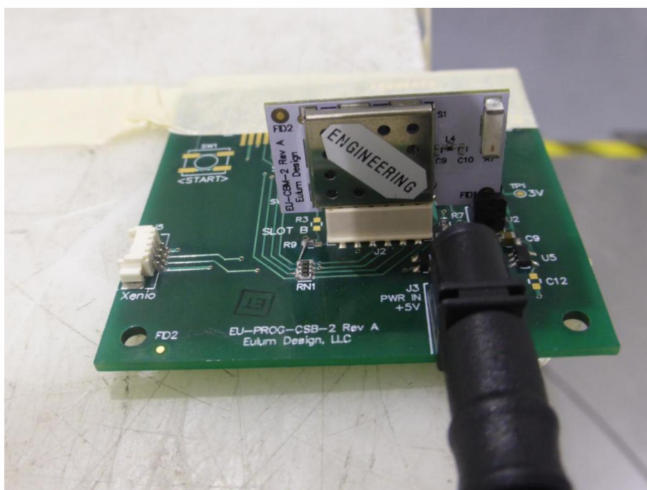
Radiated spurious emission Test Setup for close-up-4
