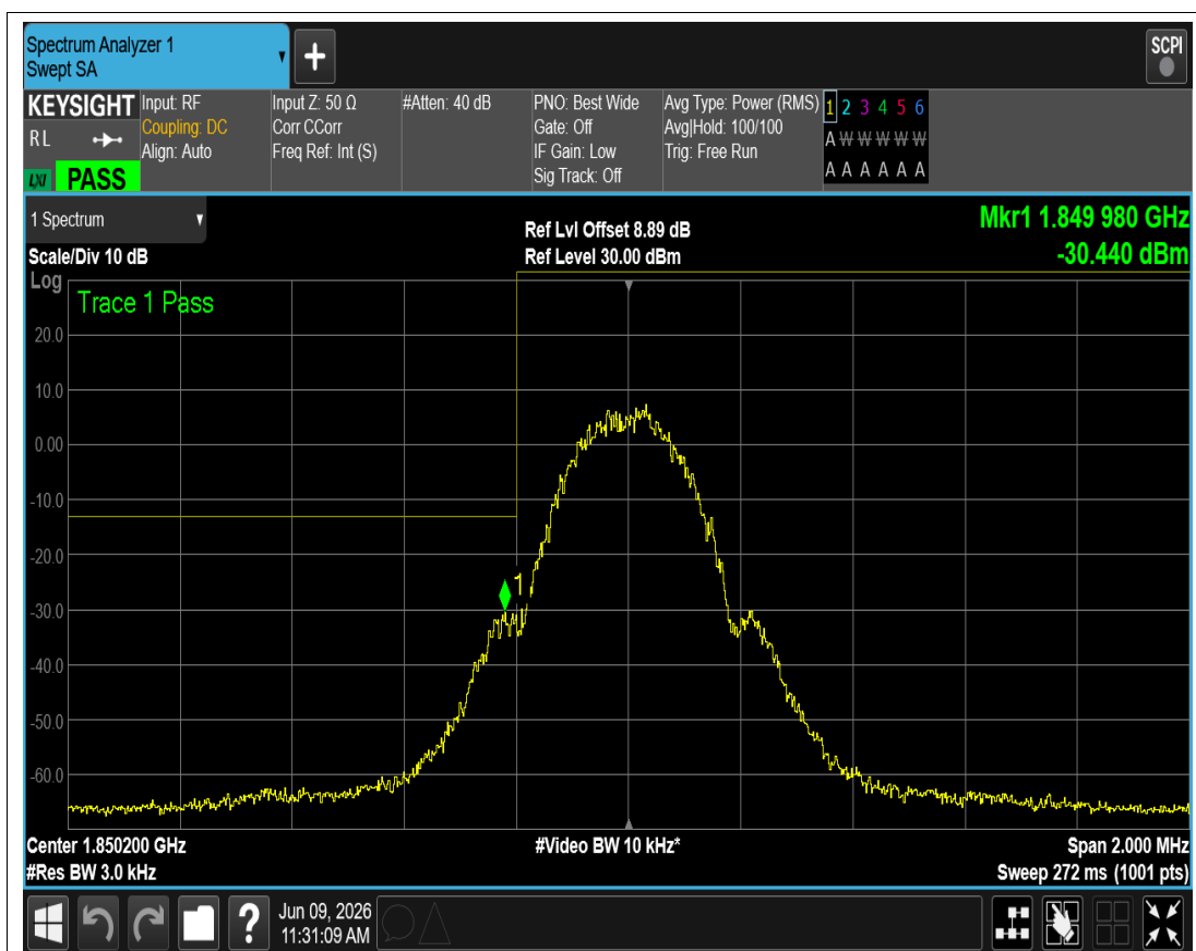
GSM1900 Channel=512
