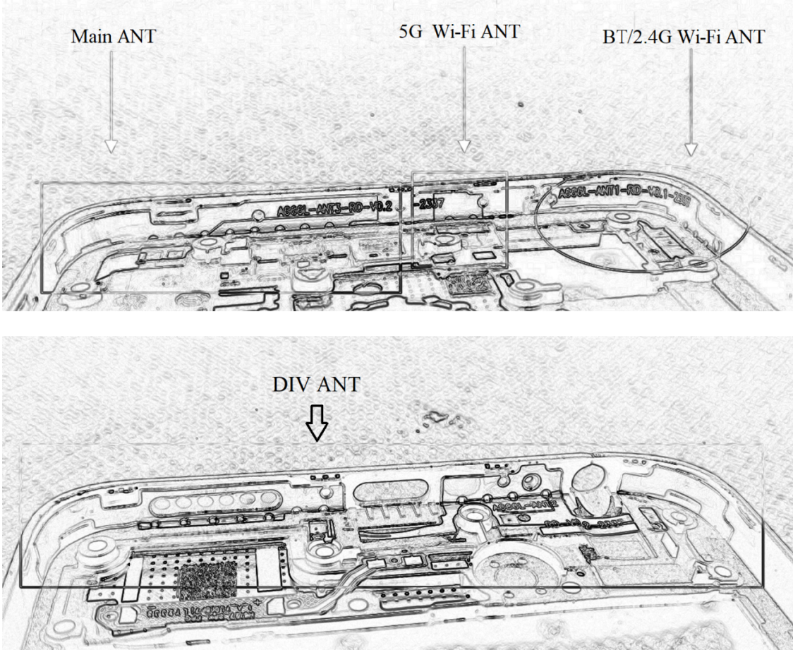
Antenna Photo
