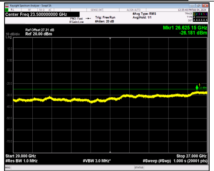
Band7_5MHz_QPSK_21100_1RB#0_20000~27000_20000~27000 0
