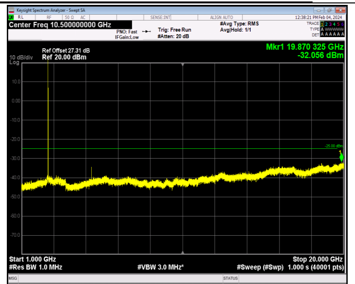
Band7_5MHz_64QAM_21425_1RB#0_1000~20000_1000~20000
