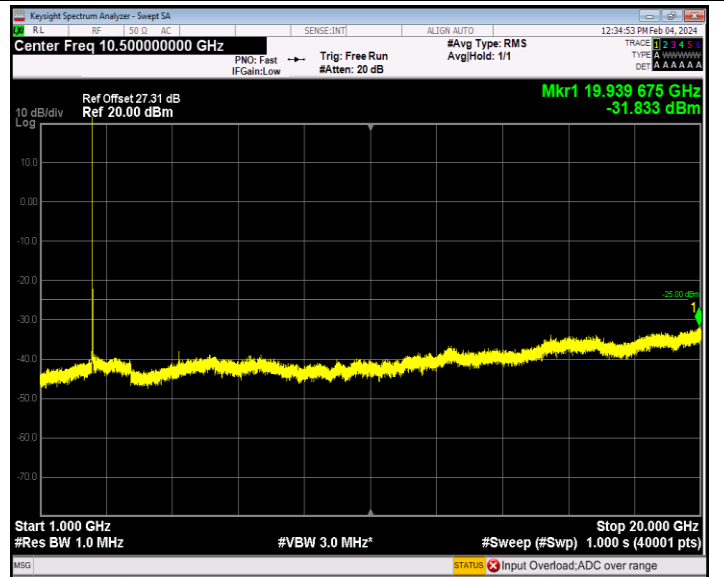
Band7_5MHz_64QAM_20775_1RB#0_1000~20000_1000~20000
