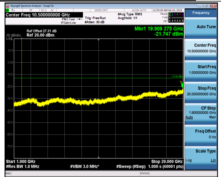
Band2_1.4MHz_16QAM_18900_1RB#0_1000~20000_1000~20000
