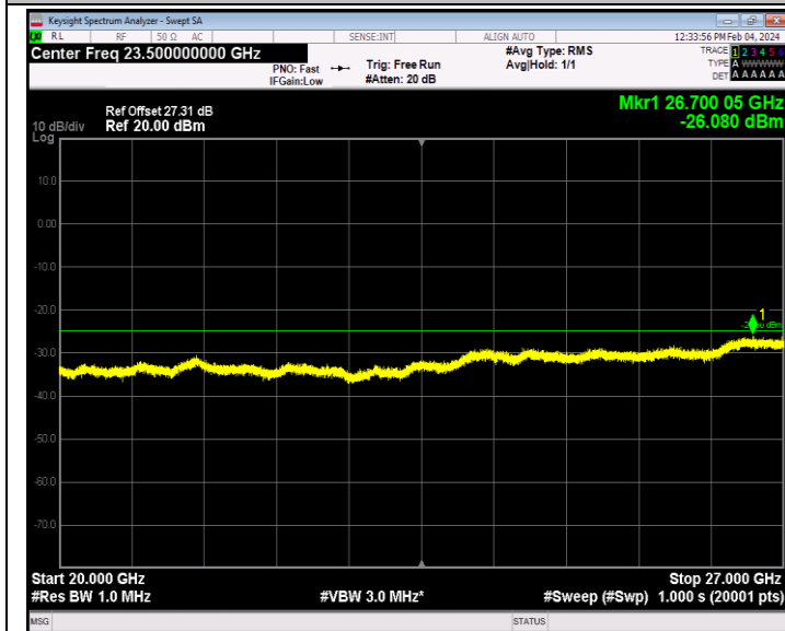
Band7_5MHz_QPSK_20775_1RB#0_20000~27000_20000~2700
