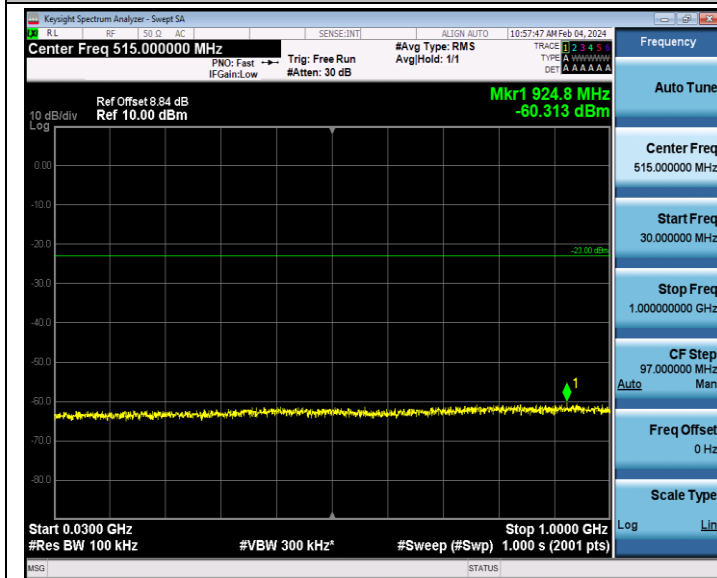
Band2_1.4MHz_16QAM_18607_1RB#0_30~1000_30~1000
