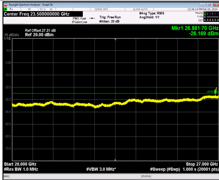
Band7_5MHz_16QAM_21100_1RB#0_20000~27000_20000~27000
