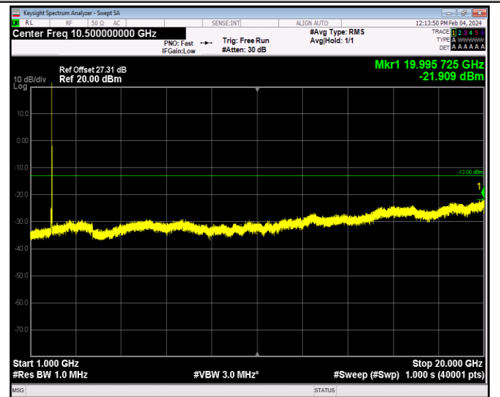
Band2_20MHz_64QAM_19100_1RB#0_1000~20000_1000~2000 0
