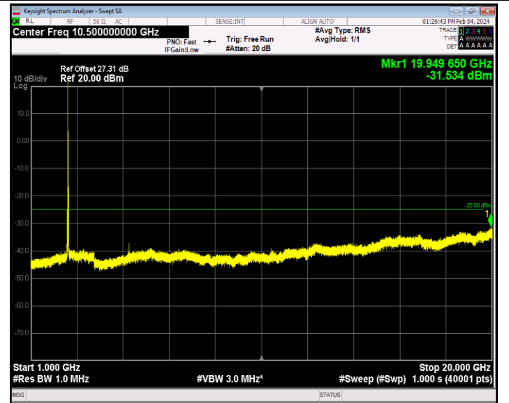
Band7_20MHz_QPSK_21100_1RB#0_1000~20000_1000~20000
