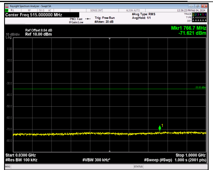
Band7_5MHz_64QAM_21100_1RB#0_30~1000_30~1000
