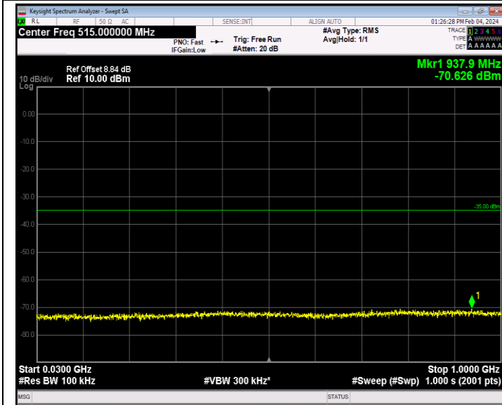
Band7_20MHz_QPSK_21100_1RB#0_30~1000_30~1000
