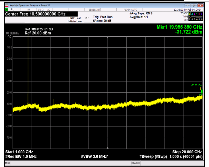
Band7_5MHz_16QAM_21100_1RB#0_1000~20000_1000~20000
