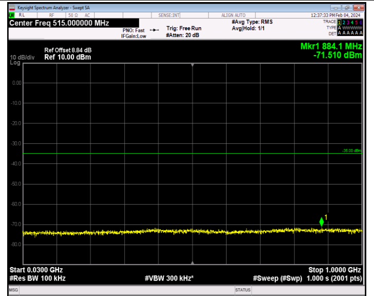
Band7_5MHz_16QAM_21425_1RB#0_30~1000_30~1000
