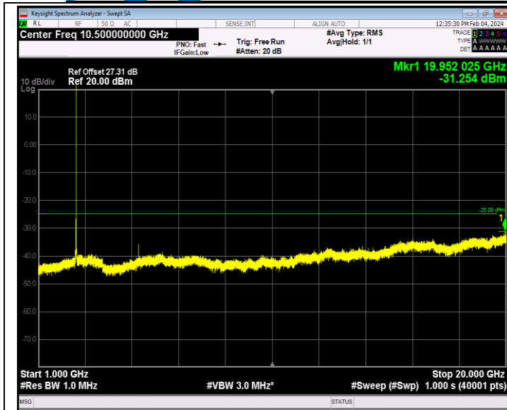
Band7_5MHz_QPSK_21100_1RB#0_1000~20000_1000~20000
