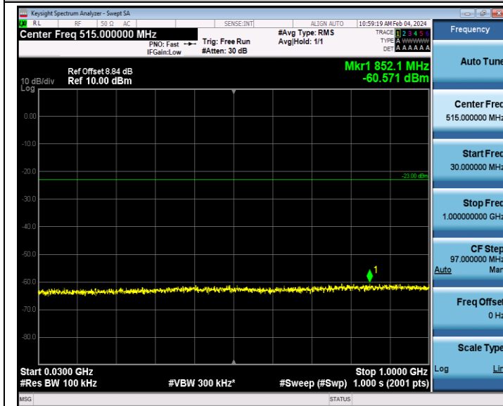
Band2_1.4MHz_64QAM_18900_1RB#0_30~1000_30~1000
