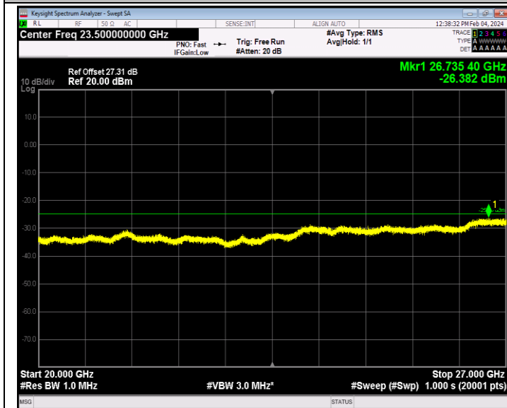
Band7_5MHz_64QAM_21425_1RB#0_20000~27000_20000~270 00
