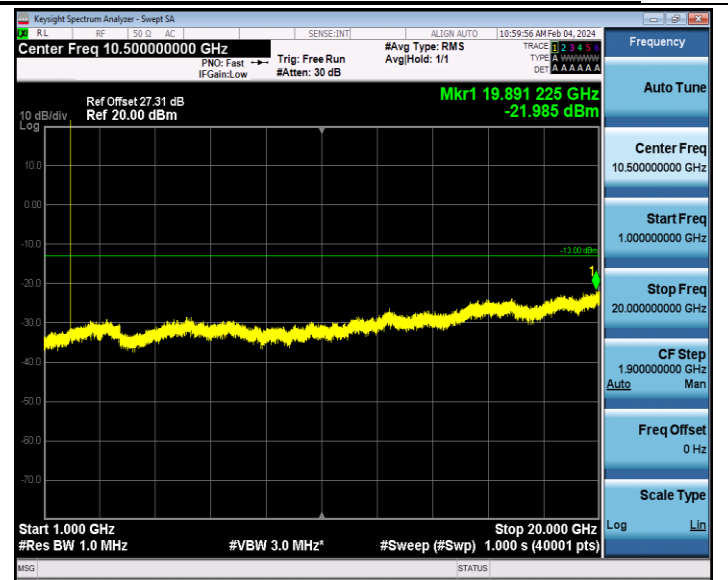
Band2_1.4MHz_QPSK_19193_1RB#0_1000~20000_1000~2000 0
