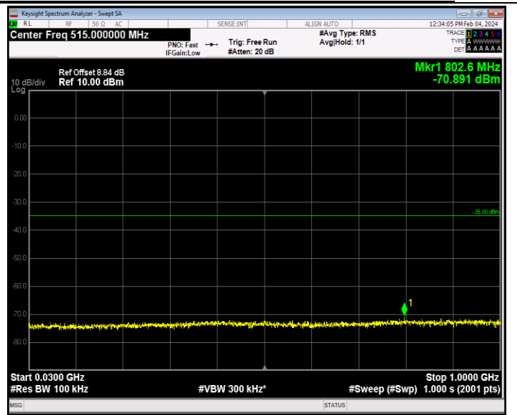
Band7_5MHz_16QAM_20775_1RB#0_30~1000_30~1000
