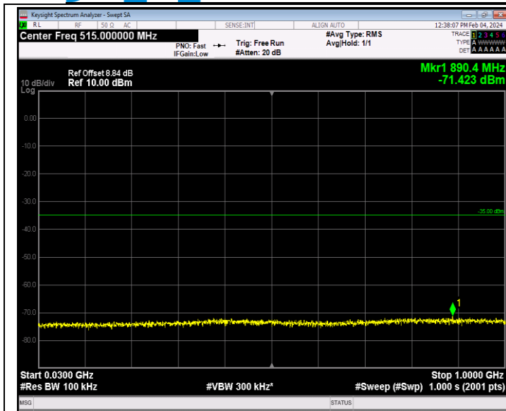
Band7_5MHz_64QAM_21425_1RB#0_30~1000_30~1000
