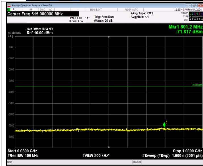
Band7_5MHz_16QAM_21100_1RB#0_30~1000_30~1000
