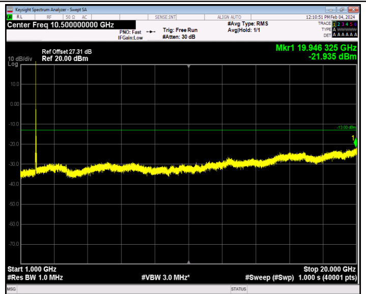
Band2_20MHz_QPSK_18700_1RB#0_1000~20000_1000~20000
