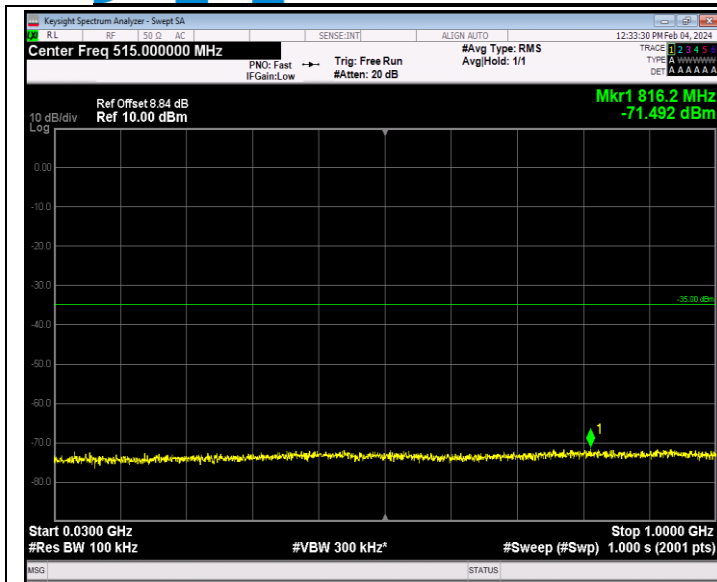
Band7_5MHz_QPSK_20775_1RB#0_30~1000_30~1000
