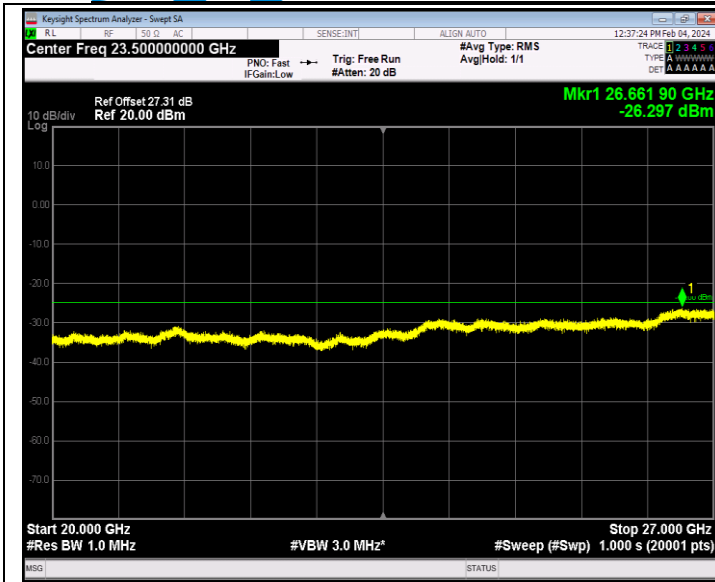
Band7_5MHz_QPSK_21425_1RB#0_20000~27000_20000~27000 0
