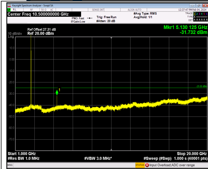
Band7_5MHz_16QAM_21425_1RB#0_1000~20000_1000~20000
