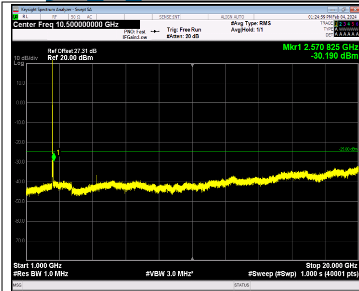
Band7_20MHz_QPSK_20850_1RB#0_1000~20000_1000~20000
