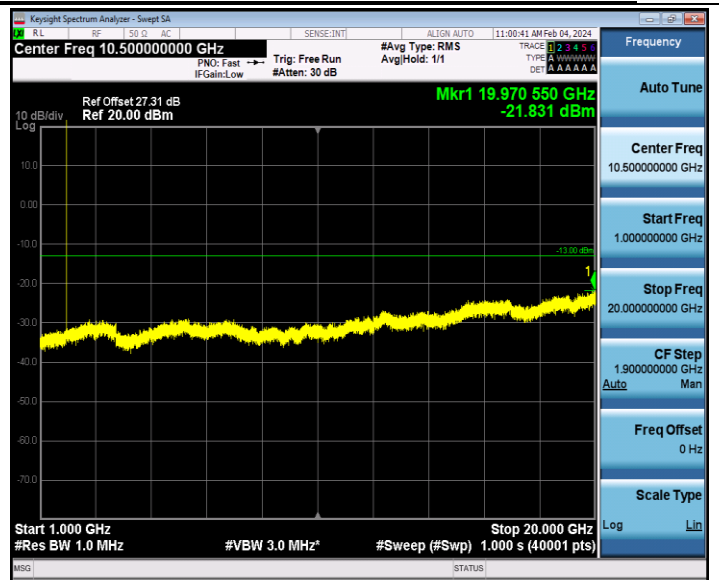
Band2_1.4MHz_64QAM_19193_1RB#0_1000~20000_1000~20000
