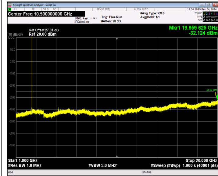
Band7_5MHz_16QAM_20775_1RB#0_1000~20000_1000~20000
