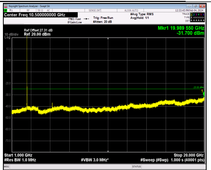
Band7_5MHz_QPSK_20775_1RB#0_1000~20000_1000~20000
