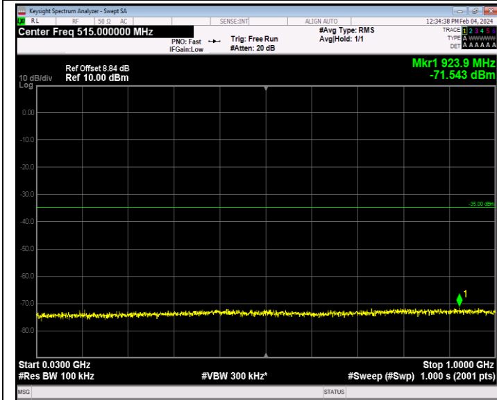
Band7_5MHz_64QAM_20775_1RB#0_30~1000_30~1000
