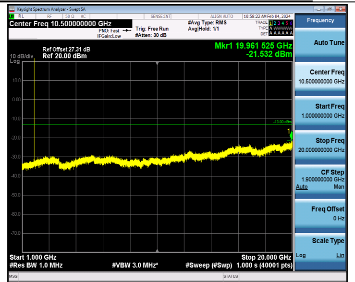
Band2_1.4MHz_64QAM_18607_1RB#0_1000~20000_1000~2000
