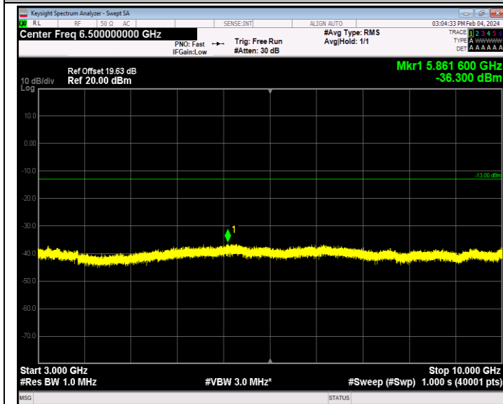
Band26_1.4MHz_QPSK_26783_1RB#0_3000~10000_3000~10000
