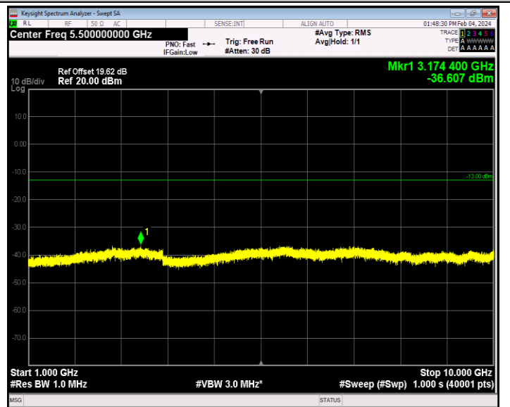
Band12_1.4MHz_64QAM_23017_1RB#0_1000~10000_1000~10000
