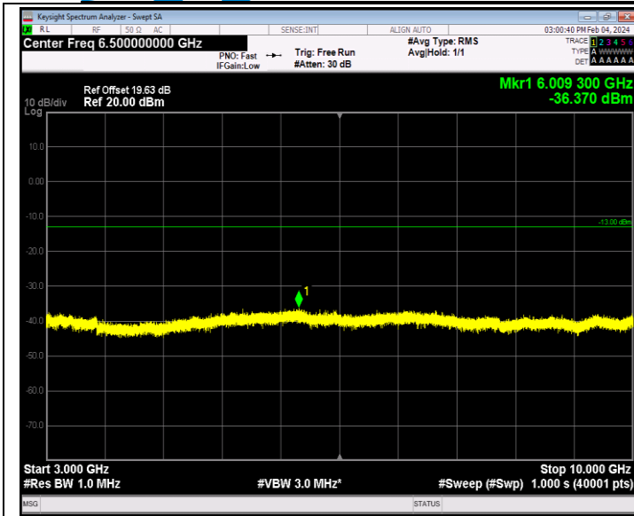
Band26_1.4MHz_QPSK_26697_1RB#0_3000~10000_3000~10000
