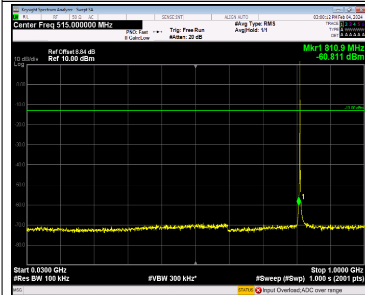
Band26_1.4MHz_QPSK_26697_1RB#0_30~1000_30~1000
