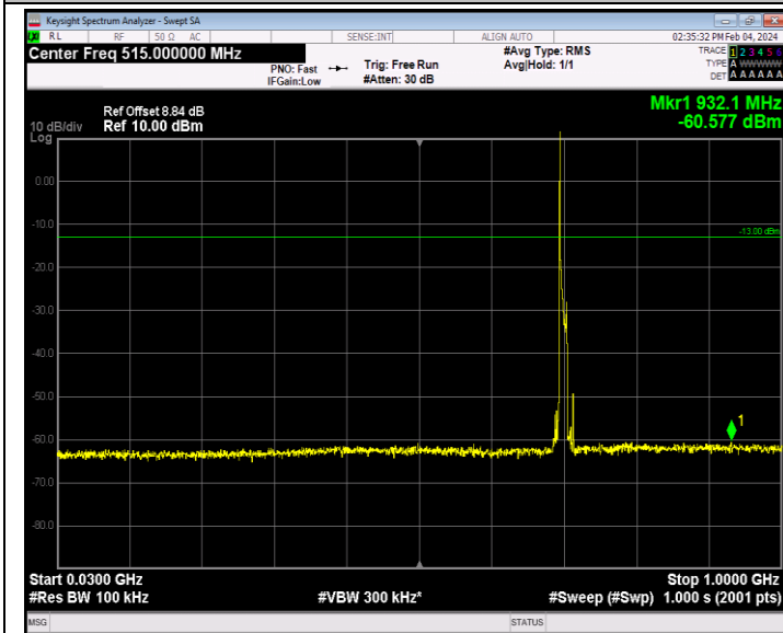
Band12_10MHz_64QAM_23095_1RB#0_30~1000_30~1000
