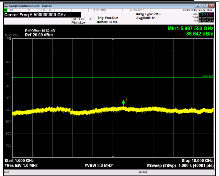
Band12_1.4MHz_64QAM_23095_1RB#0_1000~10000_1000~10000
