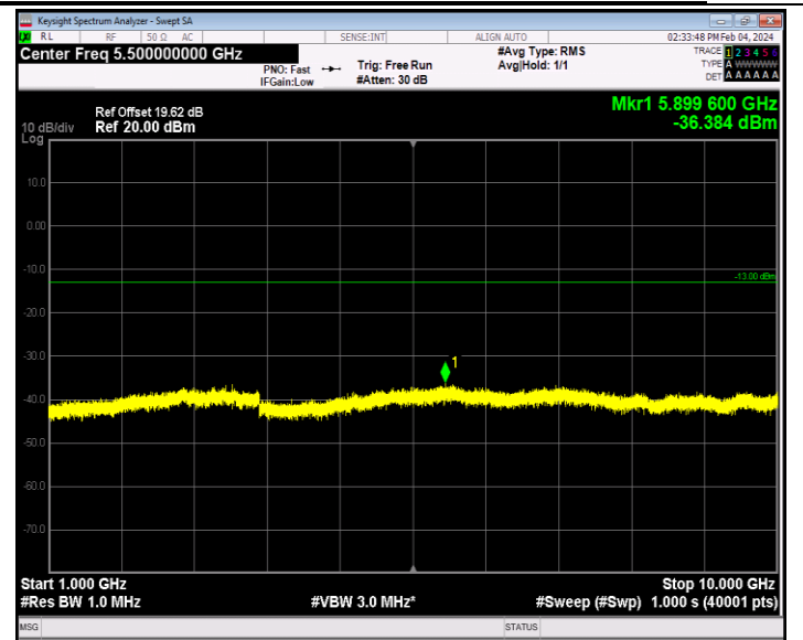
Band12_10MHz_QPSK_23060_1RB#0_1000~10000_1000~1000 0
