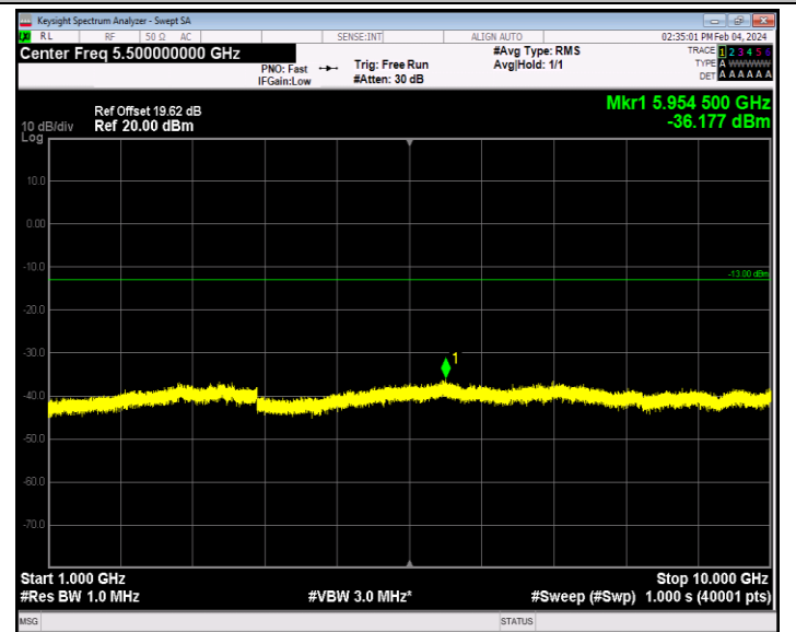
Band12_10MHz_QPSK_23095_1RB#0_1000~10000_1000~1000 0
