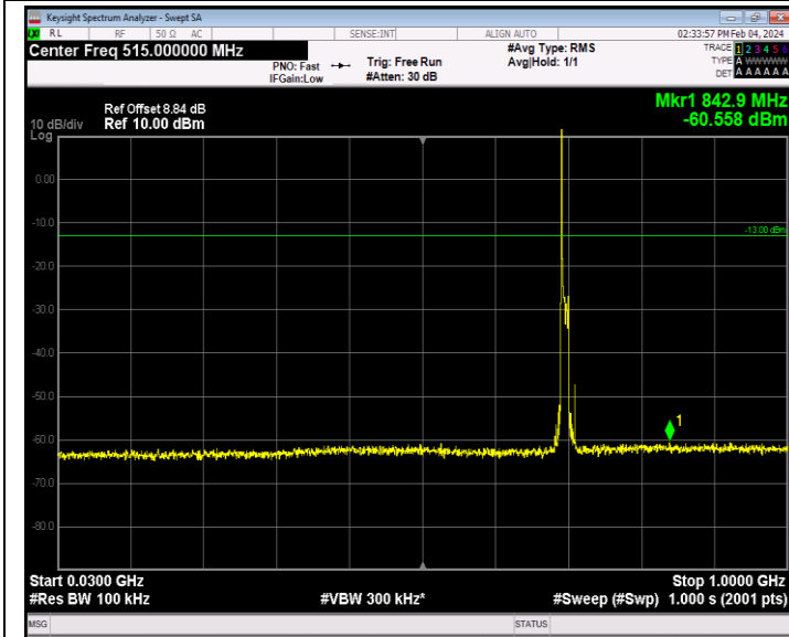
Band12_10MHz_16QAM_23060_1RB#0_30~1000_30~1000
