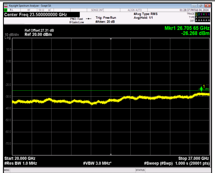
Band7_20MHz_QPSK_21350_1RB#0_20000~27000_20000~27000
