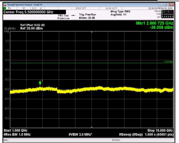
Band12_10MHz_64QAM_23060_1RB#0_1000~10000_1000~10000
