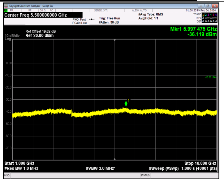
Band12_1.4MHz_16QAM_23173_1RB#0_1000~10000_1000~10000
