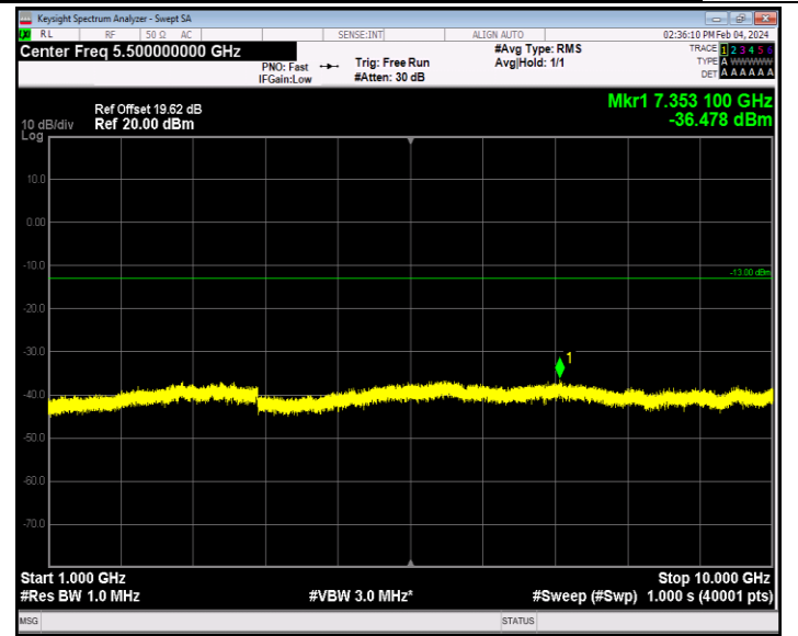
Band12_10MHz_QPSK_23130_1RB#0_1000~10000_1000~1000 0
