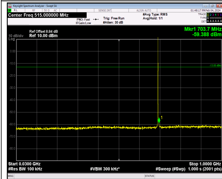
Band12_1.4MHz_64QAM_23017_1RB#0_30~1000_30~1000
