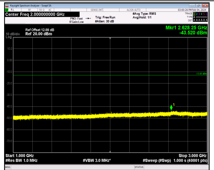
Band26_1.4MHz_QPSK_26697_1RB#0_1000~3000_1000~3000
