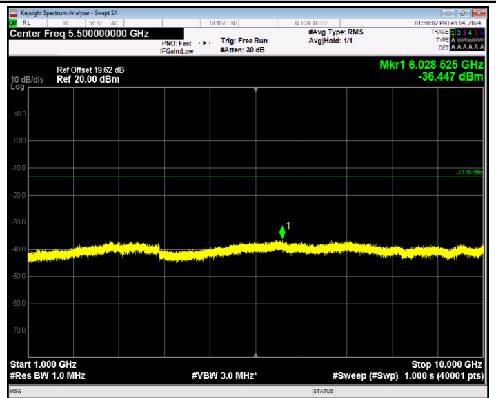
Band12_1.4MHz_QPSK_23173_1RB#0_1000~10000_1000~10000
