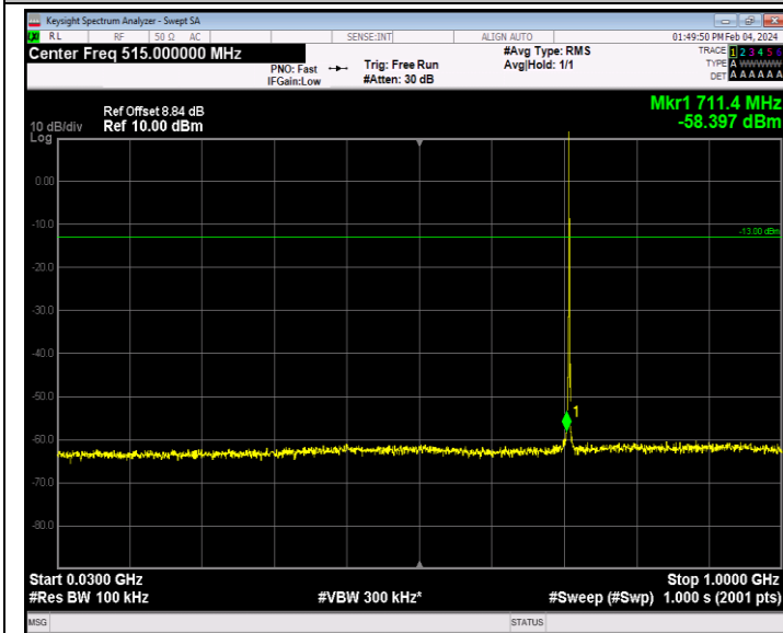
Band12_1.4MHz_QPSK_23173_1RB#0_30~1000_30~1000
