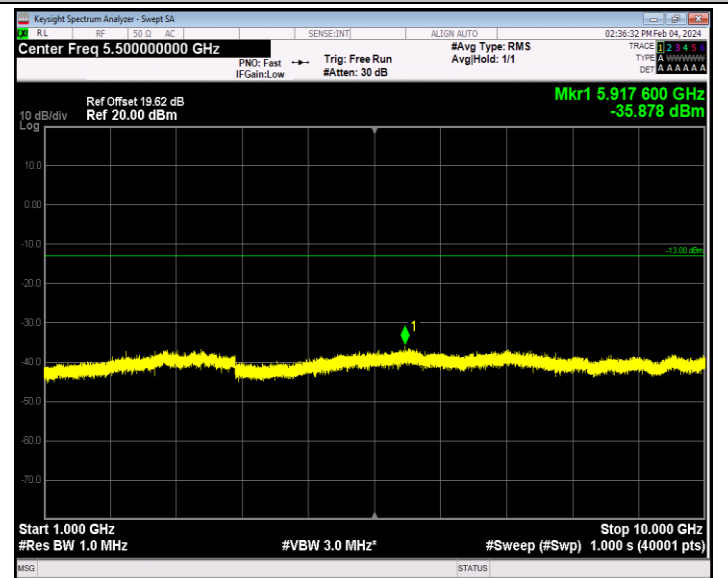
Band12_10MHz_16QAM_23130_1RB#0_1000~10000_1000~10000
