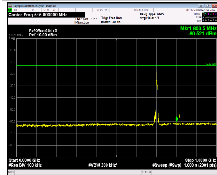
Band12_10MHz_16QAM_23130_1RB#0_30~1000_30~1000
