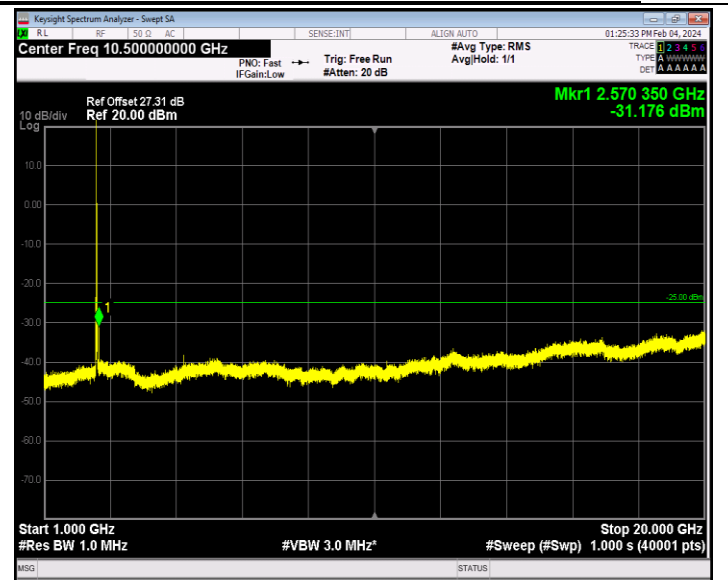
Band7_20MHz_16QAM_20850_1RB#0_1000~20000_1000~2000 0
