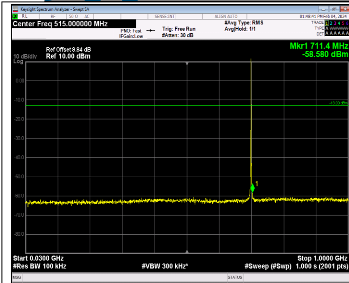
Band12_1.4MHz_QPSK_23095_1RB#0_30~1000_30~1000
