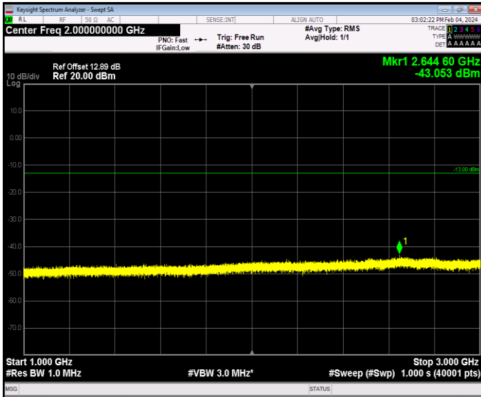
Band26_1.4MHz_QPSK_26740_1RB#0_1000~3000_1000~3000
