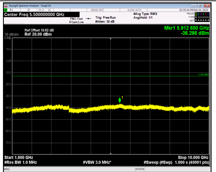
Band12_10MHz_64QAM_23095_1RB#0_1000~10000_1000~10000
