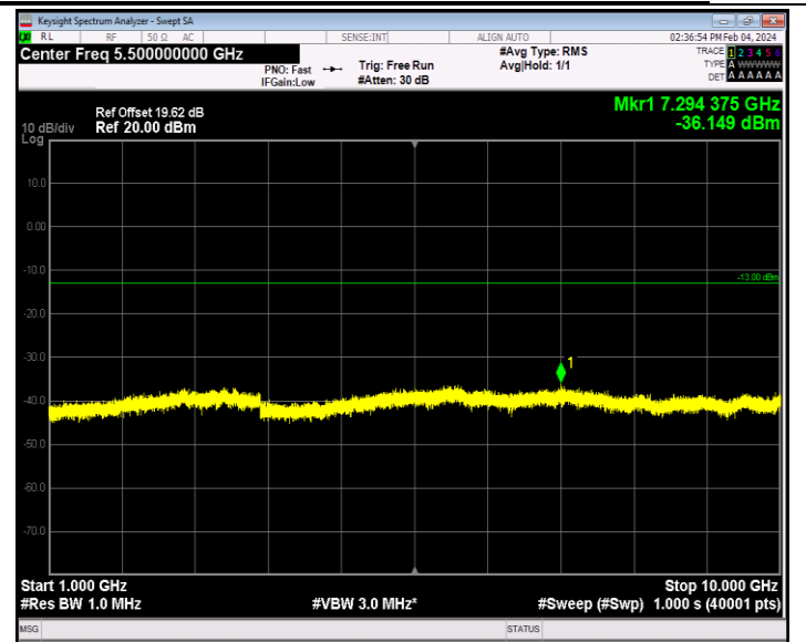
Band12_10MHz_64QAM_23130_1RB#0_1000~10000_1000~10000
