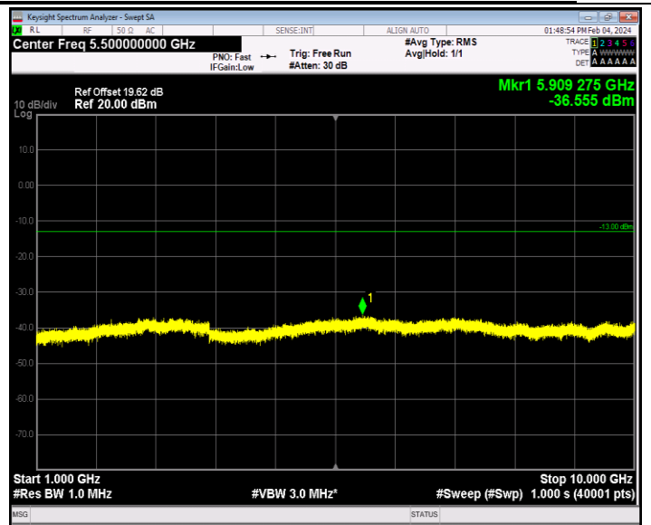
Band12_1.4MHz_QPSK_23095_1RB#0_1000~10000_1000~10000
