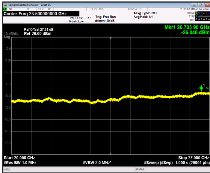
Band7_20MHz_64QAM_21100_1RB#0_20000~27000_20000~27 000
