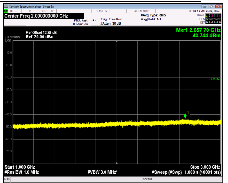
Band26_1.4MHz_QPSK_26783_1RB#0_1000~3000_1000~3000
