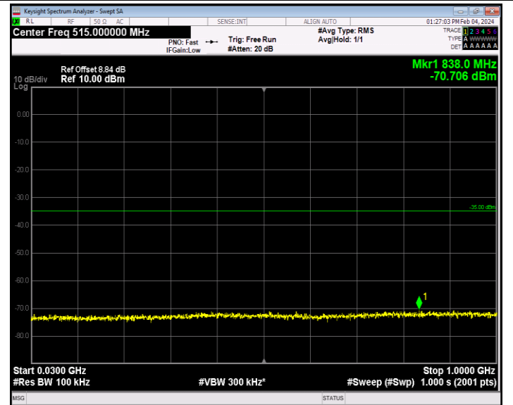
Band7_20MHz_16QAM_21100_1RB#0_30~1000_30~1000
