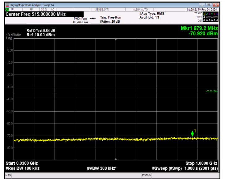
Band7_20MHz_64QAM_21350_1RB#0_30~1000_30~1000
