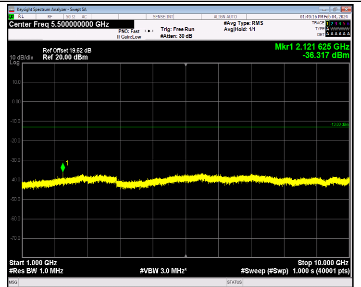
Band12_1.4MHz_16QAM_23095_1RB#0_1000~10000_1000~10000
