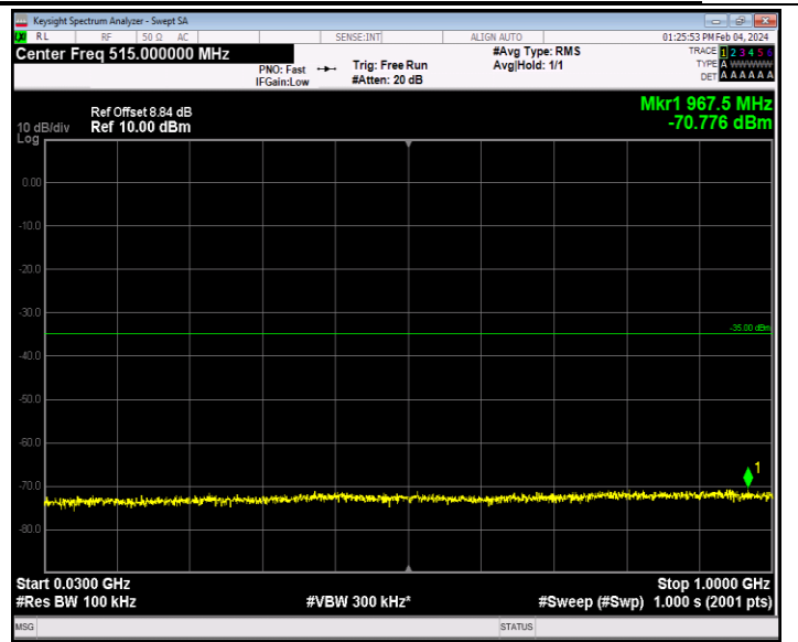
Band7_20MHz_64QAM_20850_1RB#0_30~1000_30~1000
