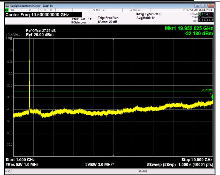
Band7_20MHz_64QAM_21100_1RB#0_1000~20000_1000~2000 0
