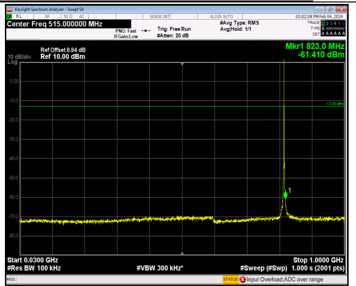
Band26_1.4MHz_QPSK_26740_1RB#0_30~1000_30~1000
