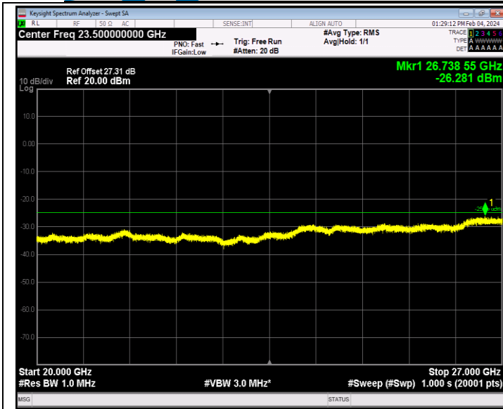
Band7_20MHz_16QAM_21350_1RB#0_20000~27000_20000~27000
