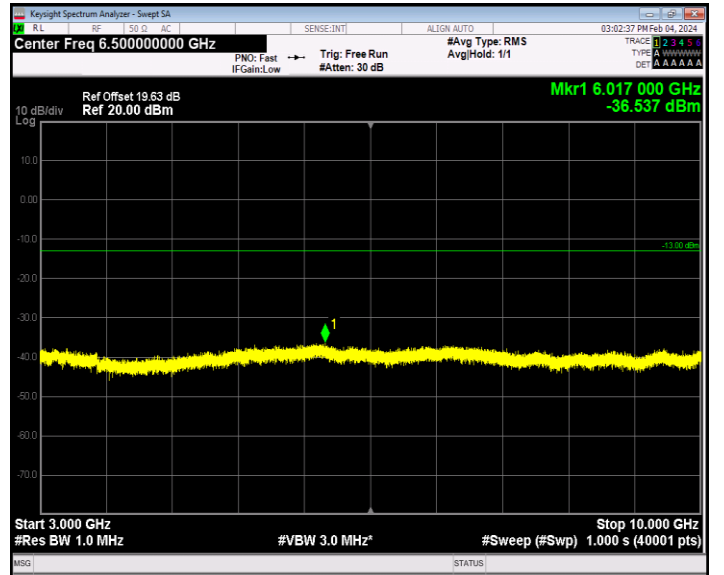
Band26_1.4MHz_QPSK_26740_1RB#0_3000~10000_3000~10000
