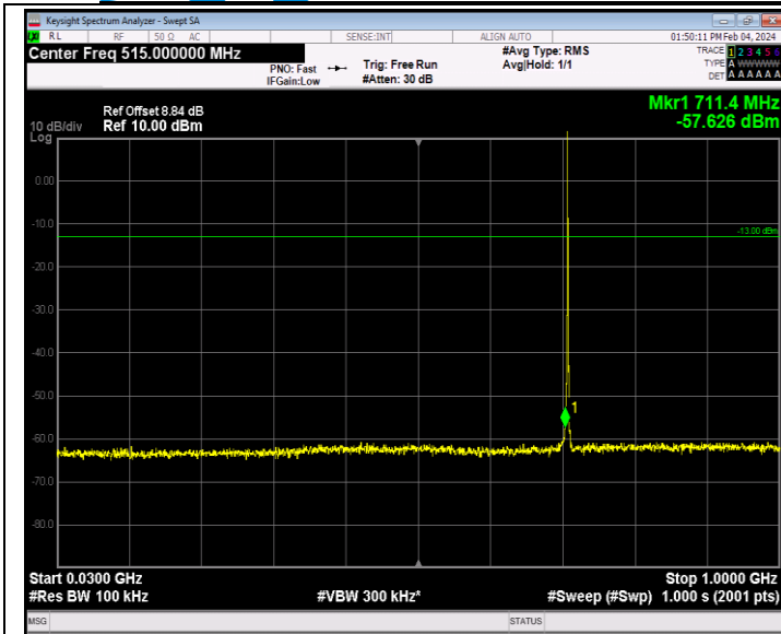
Band12_1.4MHz_16QAM_23173_1RB#0_30~1000_30~1000
