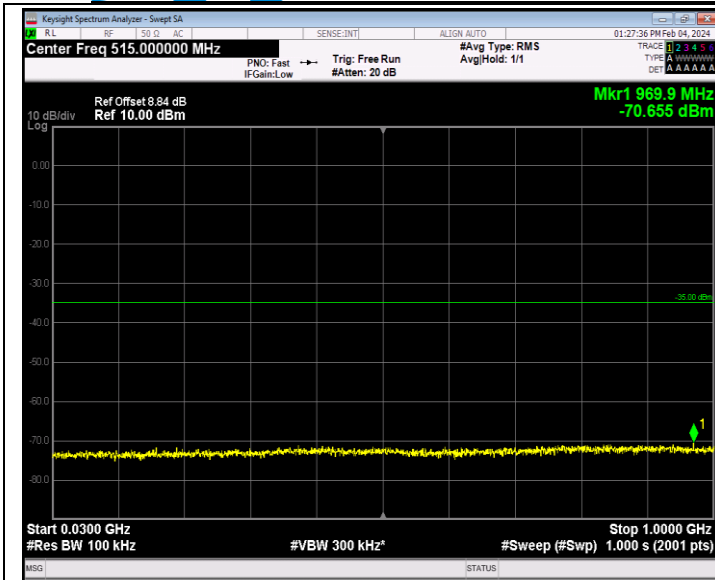
Band7_20MHz_64QAM_21100_1RB#0_30~1000_30~1000
