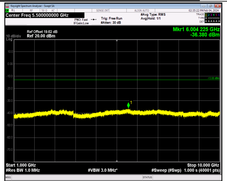
Band12_10MHz_16QAM_23095_1RB#0_1000~10000_1000~10000
