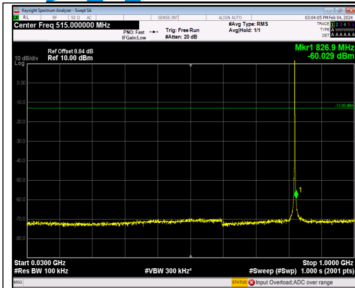
Band26_1.4MHz_QPSK_26783_1RB#0_30~1000_30~1000
