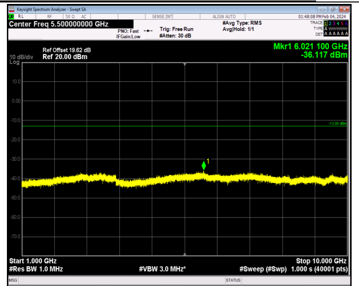
Band12_1.4MHz_16QAM_23017_1RB#0_1000~10000_1000~10000
