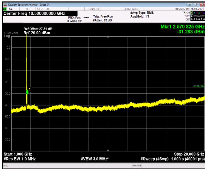
Band7_20MHz_64QAM_20850_1RB#0_1000~20000_1000~20000
