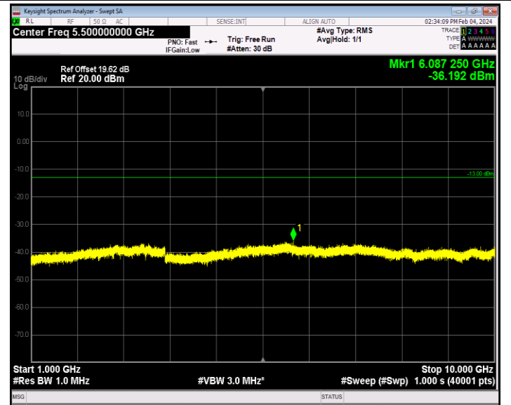
Band12_10MHz_16QAM_23060_1RB#0_1000~10000_1000~1000 00
