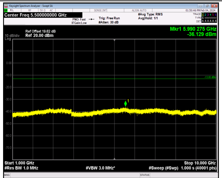
Band12_1.4MHz_64QAM_23173_1RB#0_1000~10000_1000~10000
