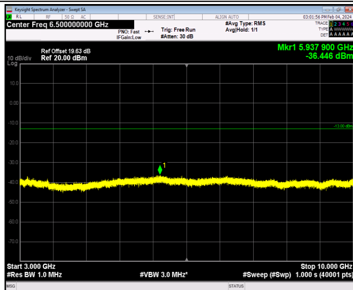
Band26_1.4MHz_64QAM_26697_1RB#0_3000~10000_3000~10000 000
