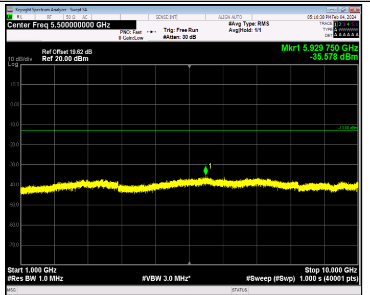
Band26_15MHz_16QAM_26865_1RB#0_1000~10000_1000~1000 00
