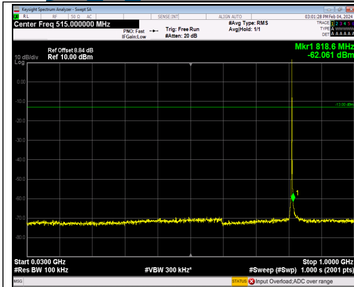
Band26_1.4MHz_64QAM_26697_1RB#0_30~1000_30~1000
