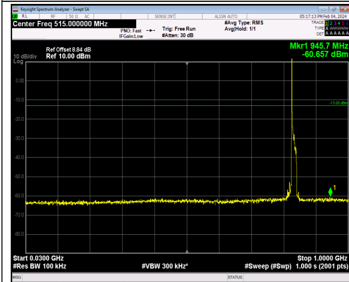
Band26_15MHz_QPSK_26915_1RB#0_30~1000_30~1000
