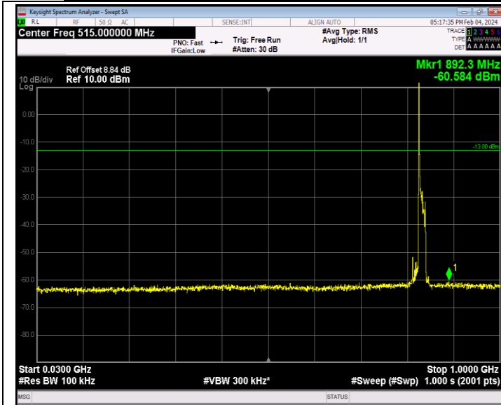
Band26_15MHz_16QAM_26915_1RB#0_30~1000_30~1000
