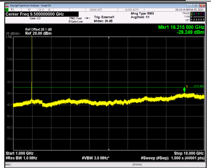
Band41_5MHz_QPSK_41215_1RB#0_1000~18000_1000~18000
