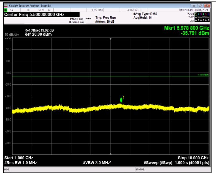
Band26_1.4MHz_16QAM_26797_1RB#0_1000~10000_1000~10000
