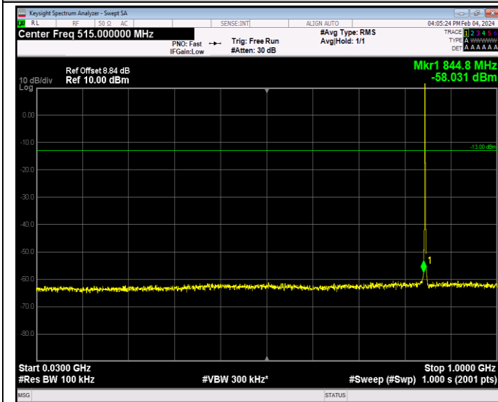
Band26_1.4MHz_64QAM_27033_1RB#0_30~1000_30~1000
