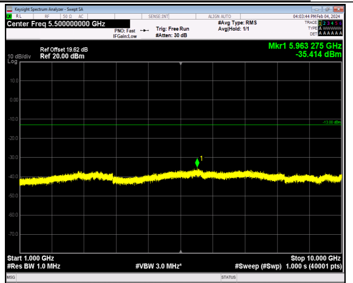
Band26_1.4MHz_QPSK_26915_1RB#0_1000~10000_1000~10000
