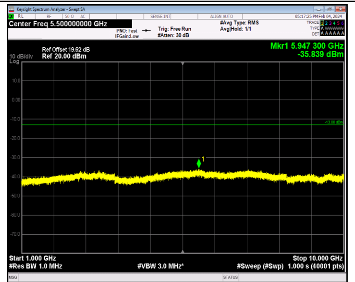
Band26_15MHz_QPSK_26915_1RB#0_1000~10000_1000~1000 0
