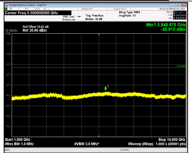
Band26_15MHz_QPSK_26865_1RB#0_1000~10000_1000~1000 0
