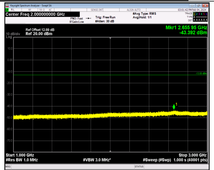
Band26_1.4MHz_64QAM_26697_1RB#0_1000~3000_1000~3000 0
