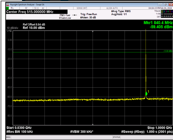
Band26_1.4MHz_64QAM_26915_1RB#0_30~1000_30~1000
