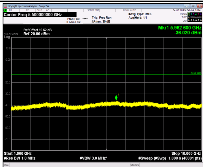
Band26_1.4MHz_64QAM_26797_1RB#0_1000~10000_1000~10000
