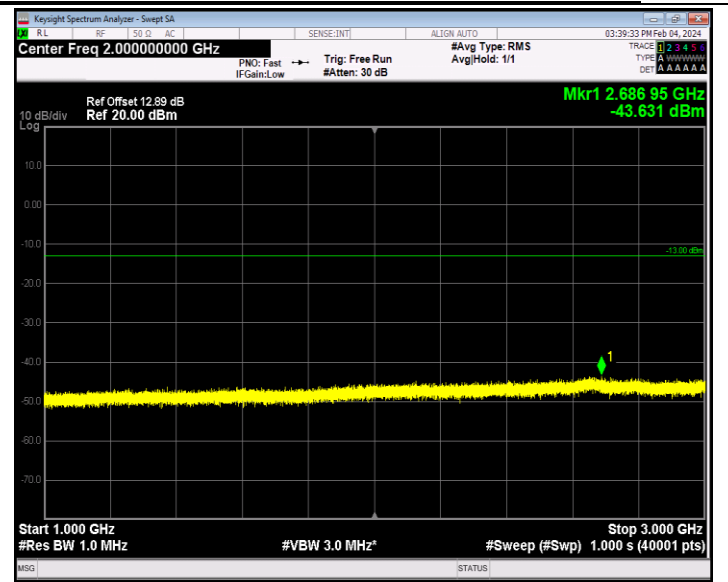
Band26_10MHz_16QAM_26740_1RB#0_1000~3000_1000~3000
