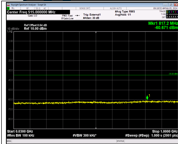
Band41_5MHz_QPSK_41215_1RB#0_30~1000_30~1000
