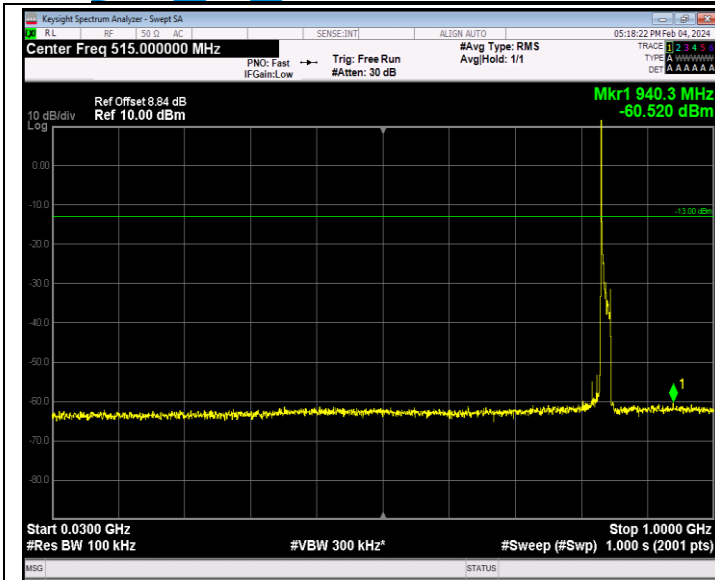
Band26_15MHz_QPSK_26965_1RB#0_30~1000_30~1000
