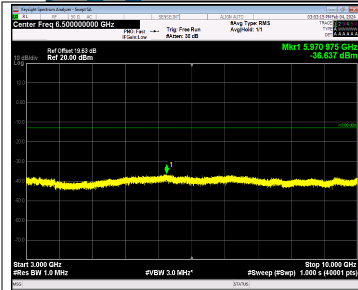
Band26_1.4MHz_16QAM_26740_1RB#0_3000~10000_3000~10000
