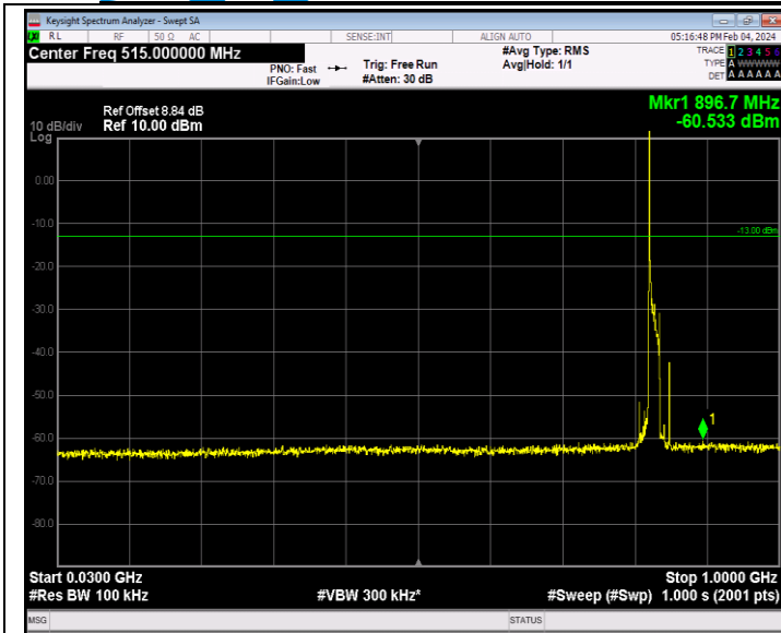
Band26_15MHz_64QAM_26865_1RB#0_30~1000_30~1000
