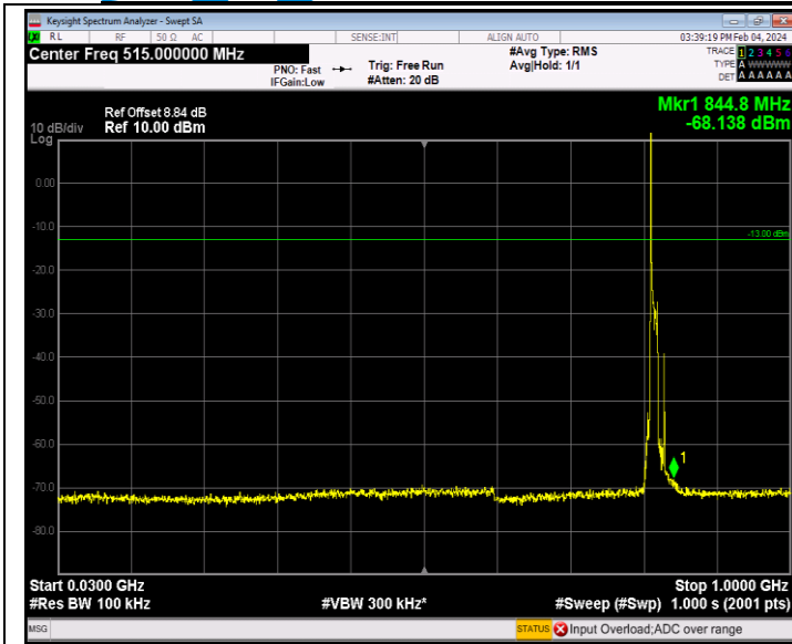
Band26_10MHz_16QAM_26740_1RB#0_30~1000_30~1000
