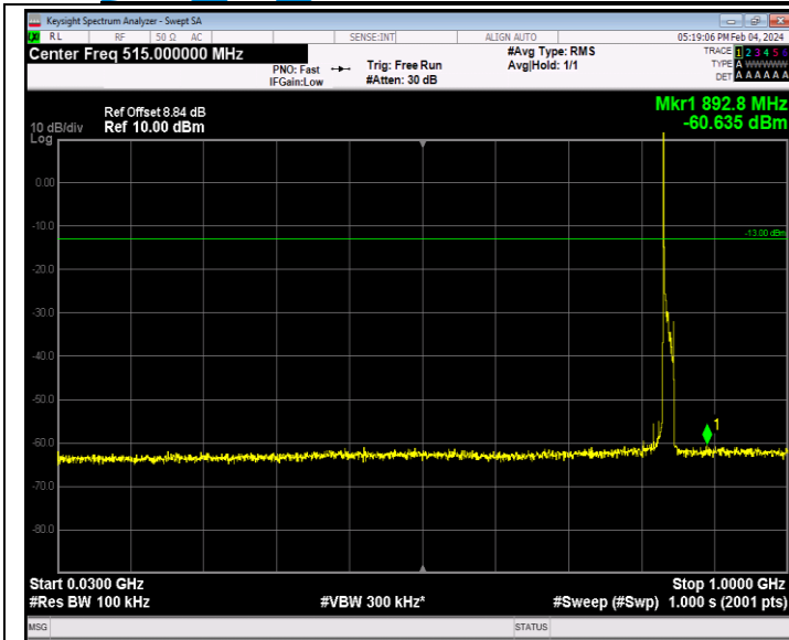
Band26_15MHz_64QAM_26965_1RB#0_30~1000_30~1000
