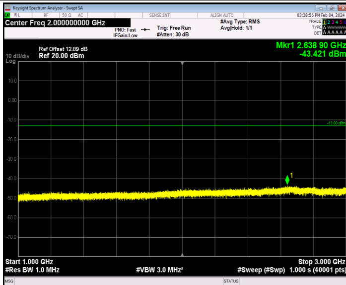
Band26_10MHz_QPSK_26740_1RB#0_1000~3000_1000~3000
