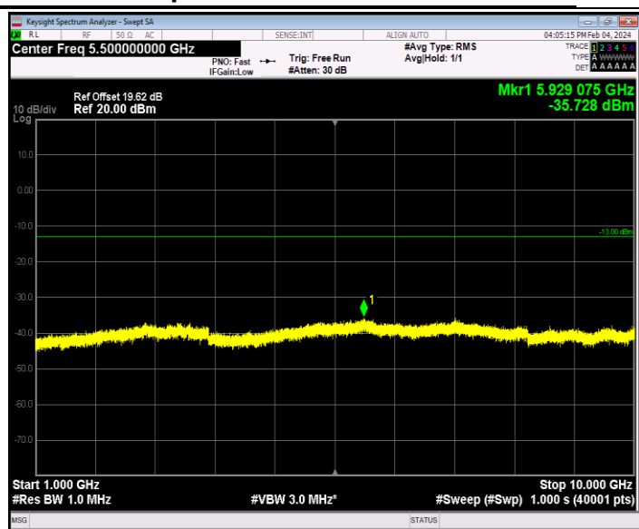
Band26_1.4MHz_16QAM_27033_1RB#0_1000~10000_1000~10000
