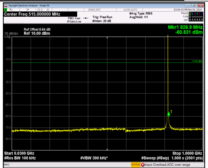
Band26_1.4MHz_16QAM_26783_1RB#0_30~1000_30~1000
