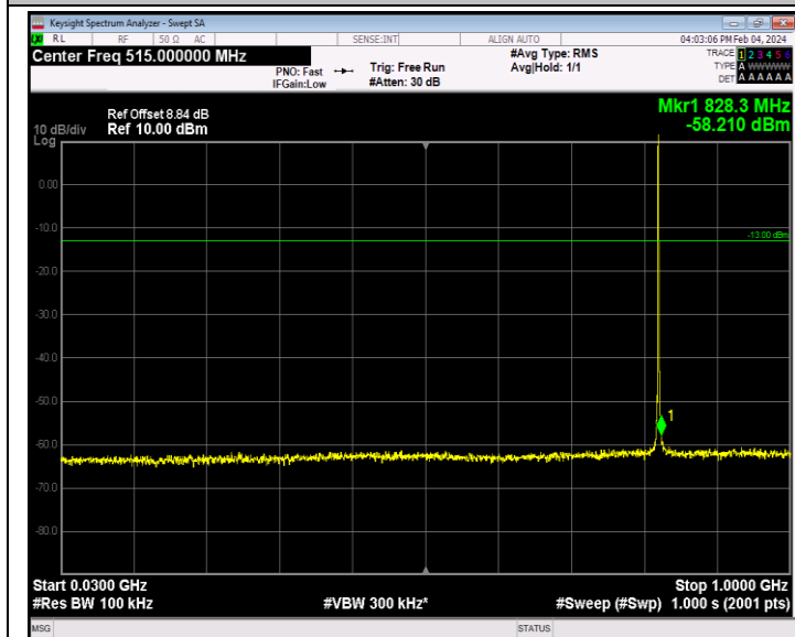
Band26_1.4MHz_64QAM_26797_1RB#0_30~1000_30~1000
