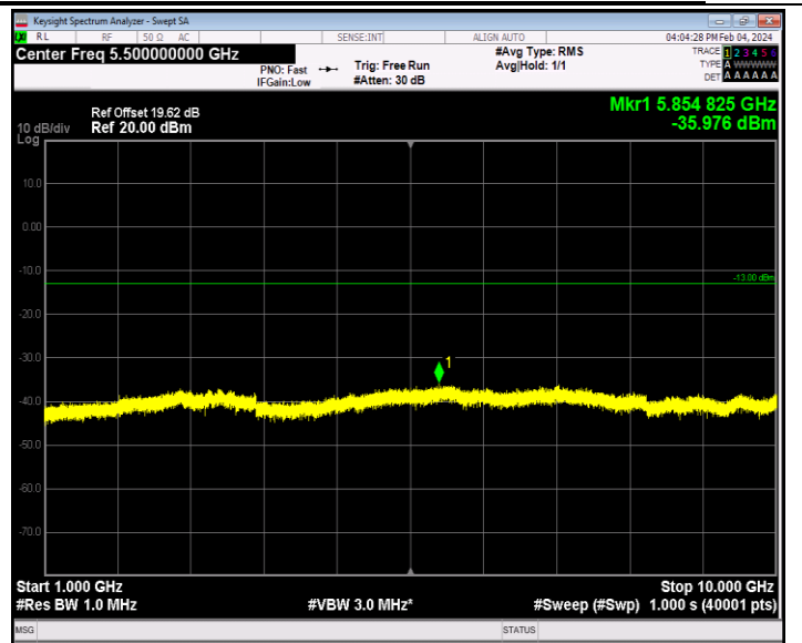
Band26_1.4MHz_64QAM_26915_1RB#0_1000~10000_1000~10000
