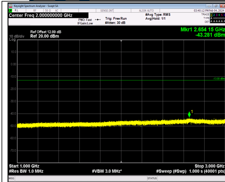
Band26_10MHz_64QAM_26740_1RB#0_1000~3000_1000~3000
