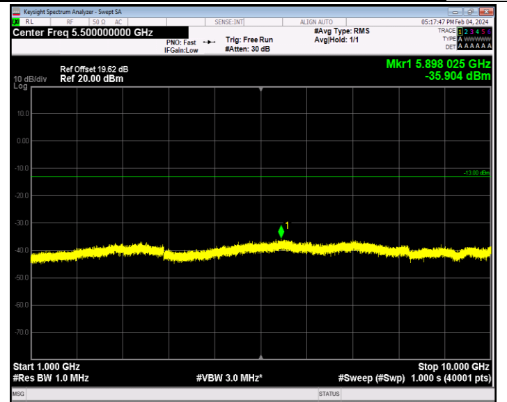
Band26_15MHz_16QAM_26915_1RB#0_1000~10000_1000~10000
