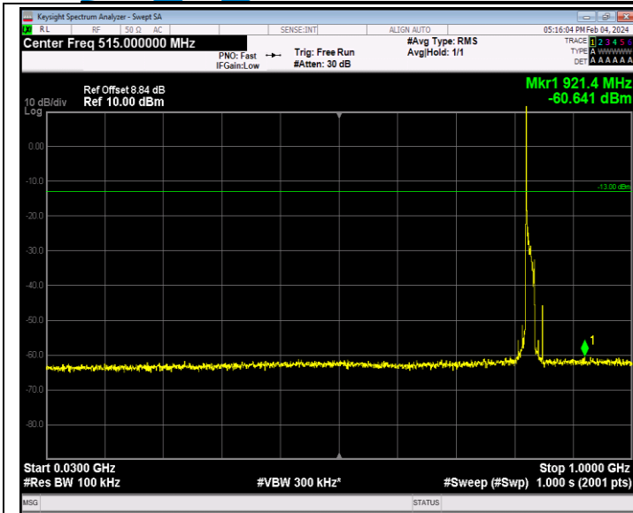
Band26_15MHz_QPSK_26865_1RB#0_30~1000_30~1000
