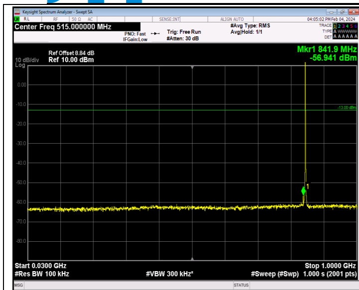
Band26_1.4MHz_16QAM_27033_1RB#0_30~1000_30~1000
