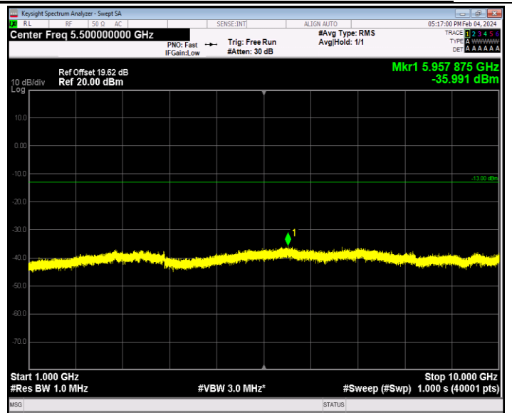
Band26_15MHz_64QAM_26865_1RB#0_1000~10000_1000~10000
