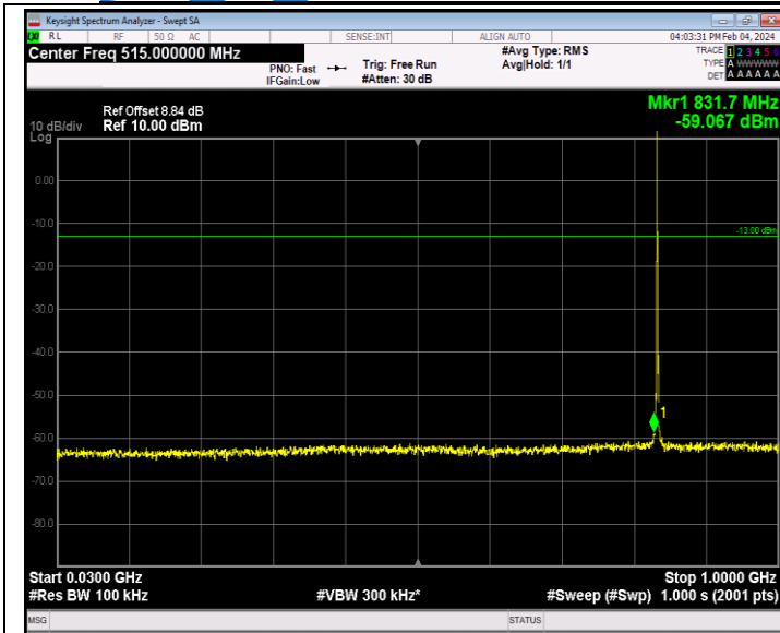
Band26_1.4MHz_QPSK_26915_1RB#0_30~1000_30~1000
