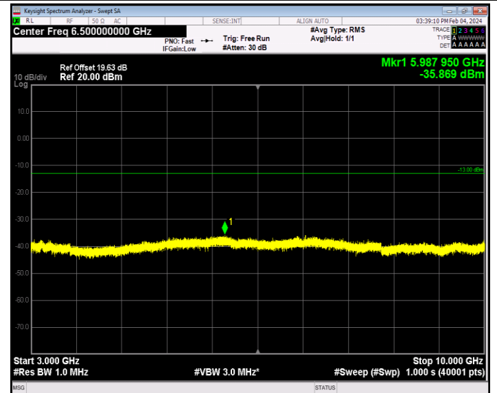
Band26_10MHz_QPSK_26740_1RB#0_3000~10000_3000~10000
