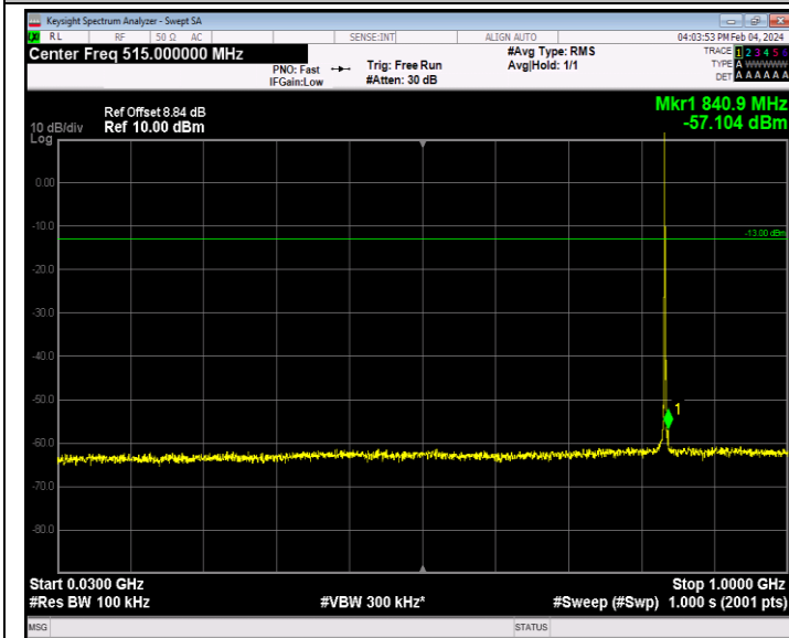
Band26_1.4MHz_16QAM_26915_1RB#0_30~1000_30~1000
