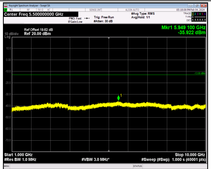
Band26_15MHz_64QAM_26915_1RB#0_1000~10000_1000~10000
