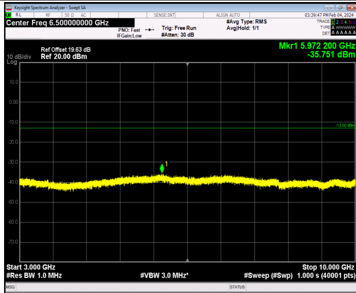
Band26_10MHz_16QAM_26740_1RB#0_3000~10000_3000~10000
