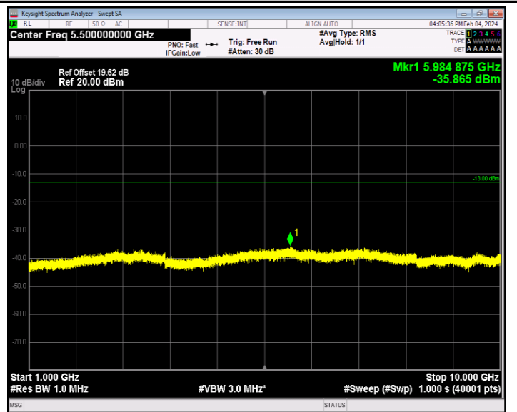
Band26_1.4MHz_64QAM_27033_1RB#0_1000~10000_1000~10000
