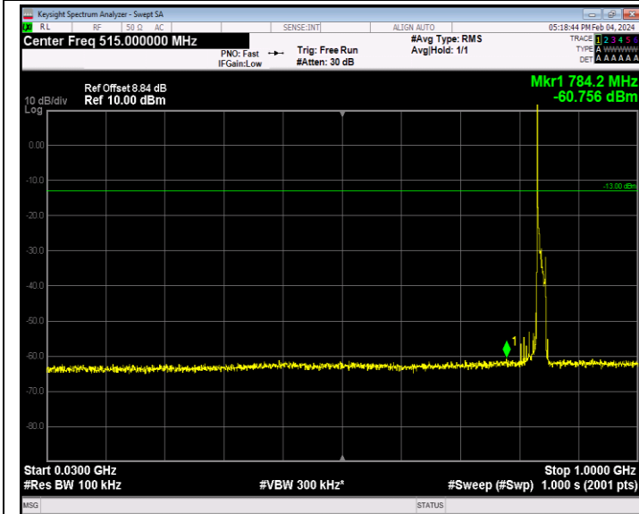
Band26_15MHz_16QAM_26965_1RB#0_30~1000_30~1000
