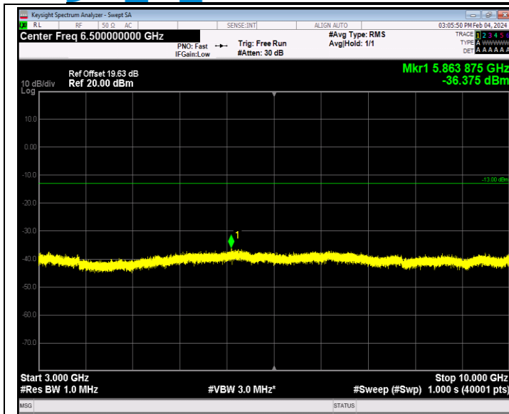
Band26_1.4MHz_64QAM_26783_1RB#0_3000~10000_3000~10000
