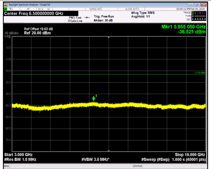
Band26_1.4MHz_16QAM_26783_1RB#0_3000~10000_3000~10000
