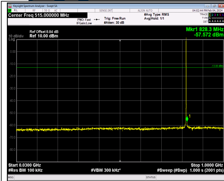
Band26_1.4MHz_16QAM_26797_1RB#0_30~1000_30~1000
