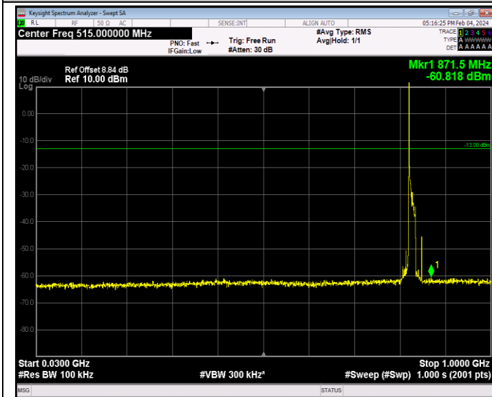
Band26_15MHz_16QAM_26865_1RB#0_30~1000_30~1000
