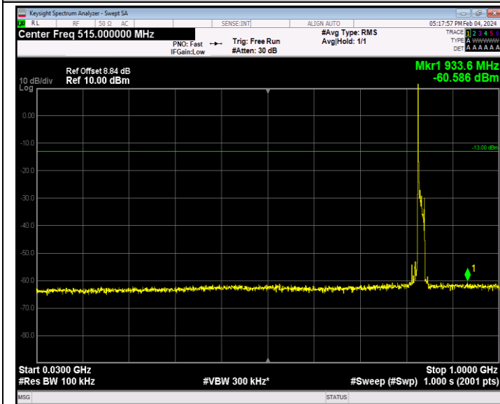
Band26_15MHz_64QAM_26915_1RB#0_30~1000_30~1000
