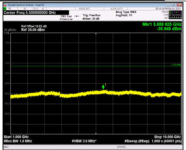
Band26_15MHz_64QAM_26965_1RB#0_1000~10000_1000~1000 00
