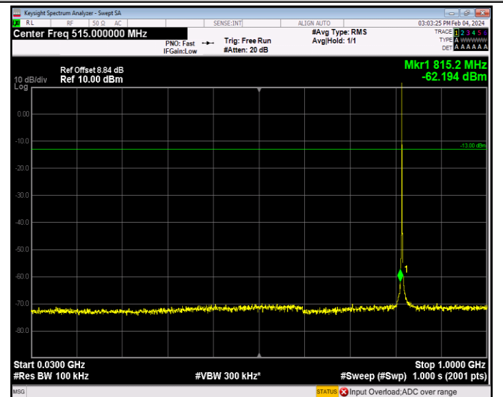
Band26_1.4MHz_64QAM_26740_1RB#0_30~1000_30~1000
