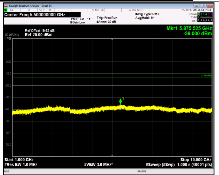
Band26_15MHz_QPSK_26965_1RB#0_1000~10000_1000~1000 0
