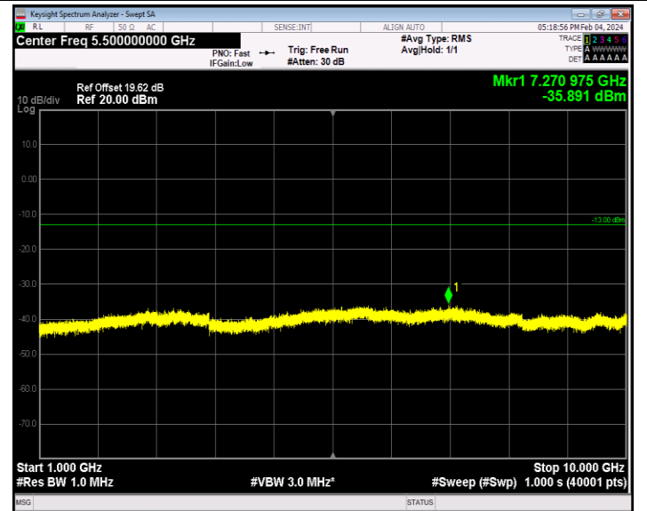
Band26_15MHz_16QAM_26965_1RB#0_1000~10000_1000~10000
