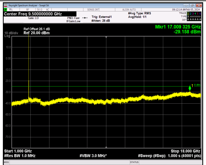
Band41_5MHz_QPSK_40065_1RB#0_1000~18000_1000~18000
