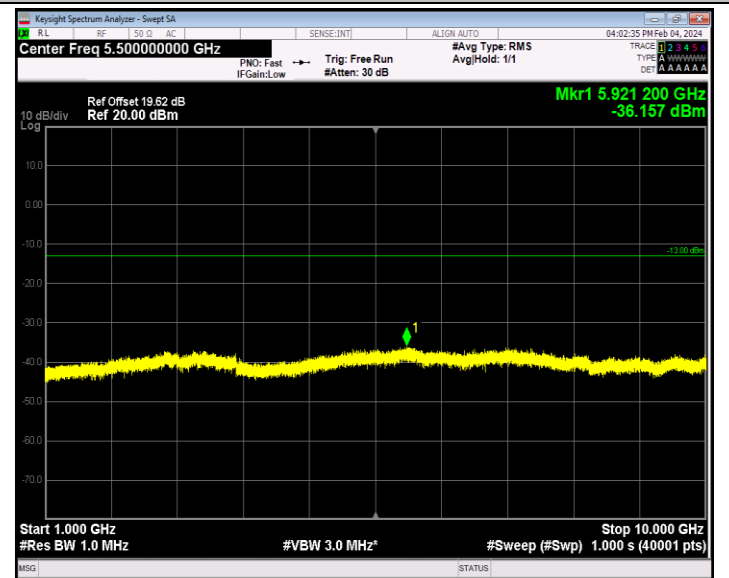
Band26_1.4MHz_QPSK_26797_1RB#0_1000~10000_1000~10000
