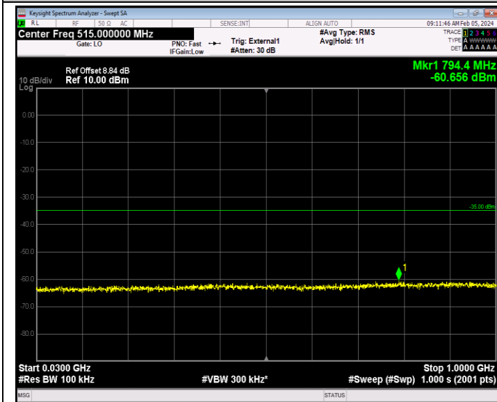
Band41_5MHz_QPSK_40065_1RB#0_30~1000_30~1000
