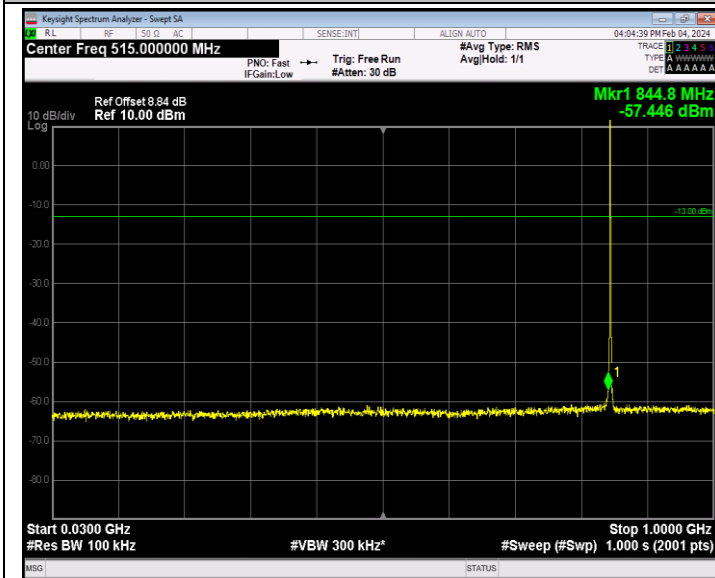
Band26_1.4MHz_QPSK_27033_1RB#0_30~1000_30~1000
