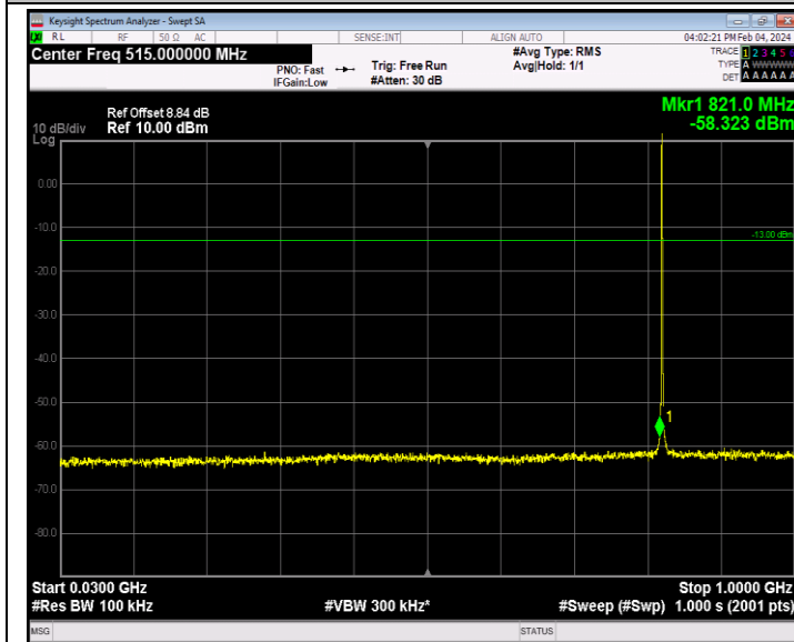
Band26_1.4MHz_QPSK_26797_1RB#0_30~1000_30~1000
