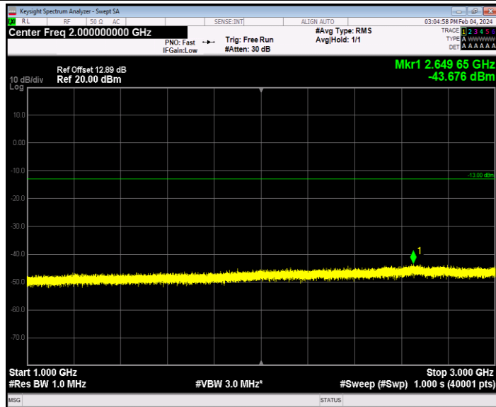
Band26_1.4MHz_16QAM_26783_1RB#0_1000~3000_1000~3000
