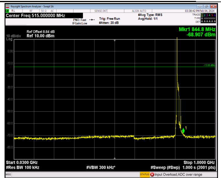
Band26_10MHz_QPSK_26740_1RB#0_30~1000_30~1000
