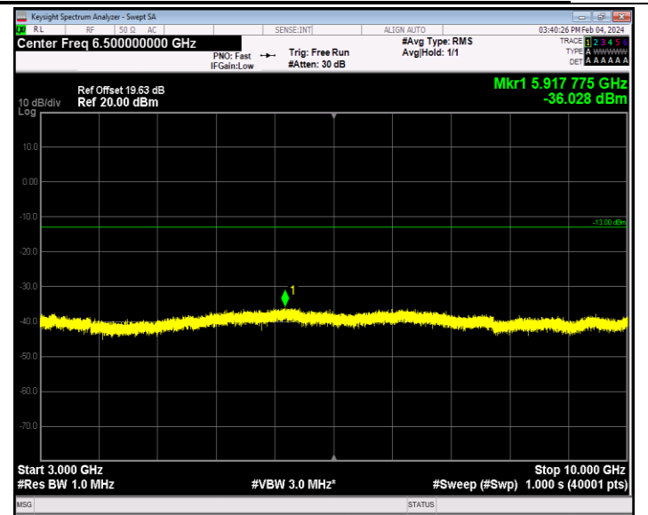
Band26_10MHz_64QAM_26740_1RB#0_3000~10000_3000~10000
