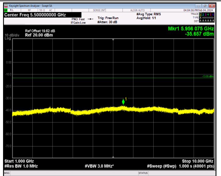
Band26_1.4MHz_16QAM_26915_1RB#0_1000~10000_1000~10000
