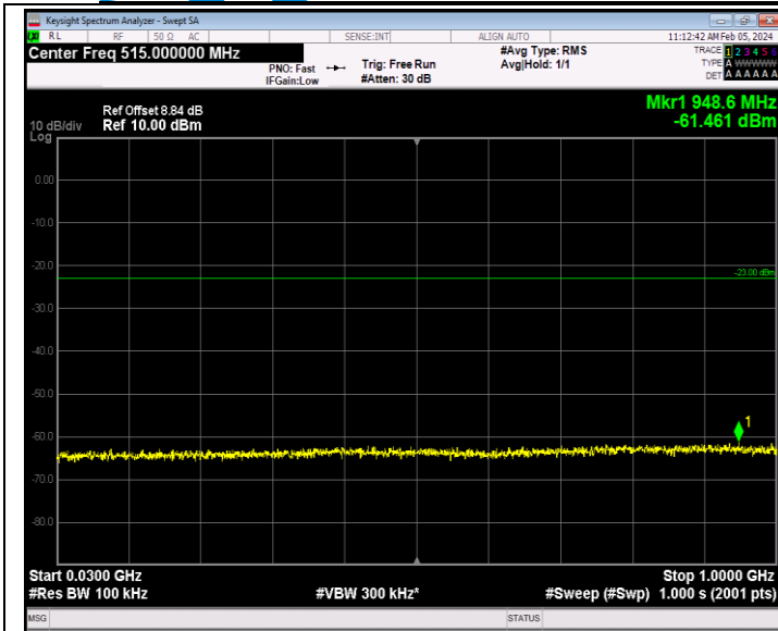
Band66_1.4MHz_64QAM_131979_1RB#0_30~1000_30~1000
