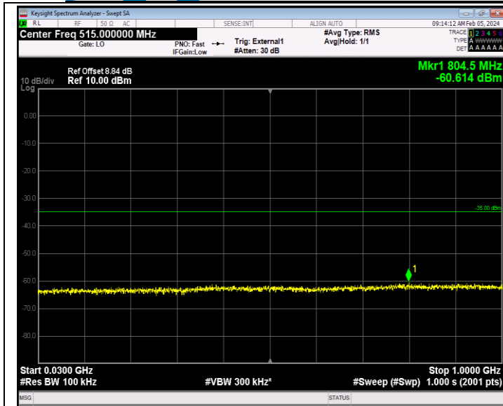
Band41_5MHz_64QAM_40065_1RB#0_30~1000_30~1000
