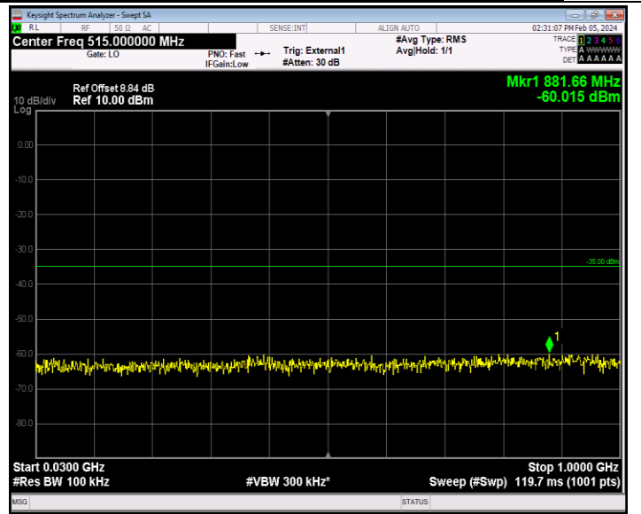
Band41_20MHz_16QAM_40640_1RB#0_30~1000_30~1000
