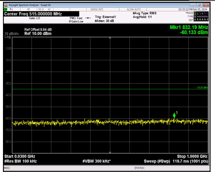
Band41_20MHz_64QAM_41140_1RB#0_30~1000_30~1000
