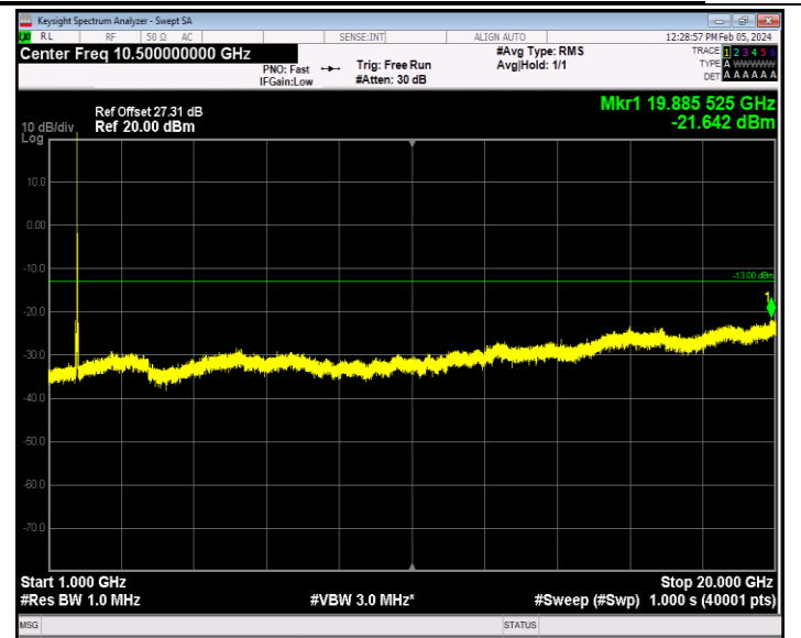
Band66_20MHz_QPSK_132322_1RB#0_1000~20000_1000~20000
