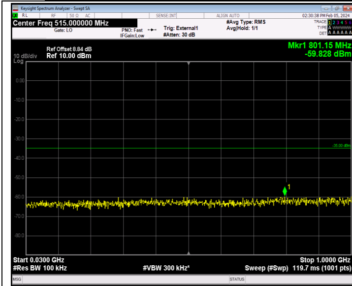
Band41_20MHz_QPSK_40640_1RB#0_30~1000_30~1000
