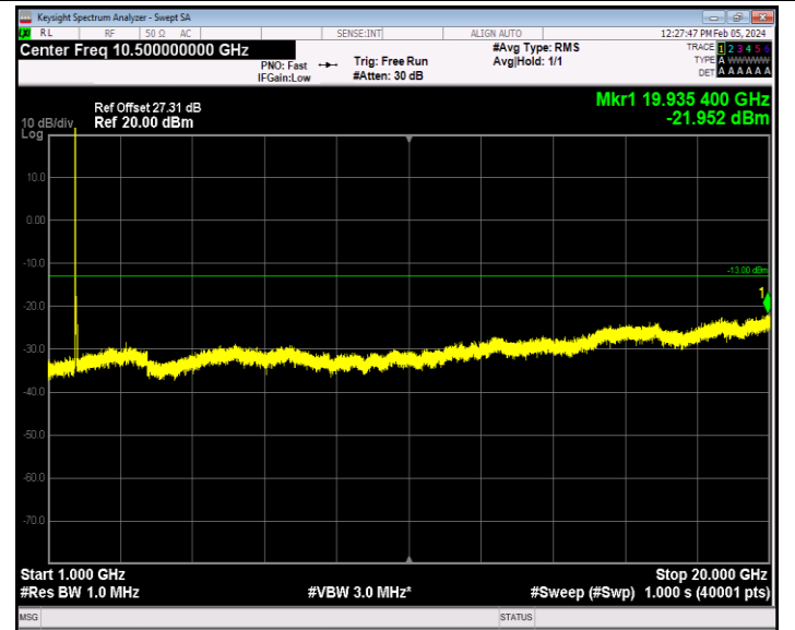
Band66_20MHz_QPSK_132072_1RB#0_1000~20000_1000~20000
