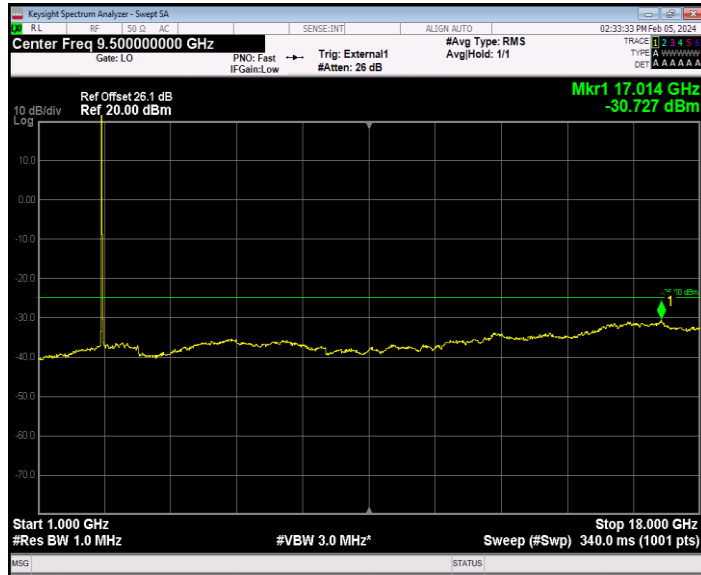
Band41_20MHz_64QAM_41140_1RB#0_1000~18000_1000~18000
