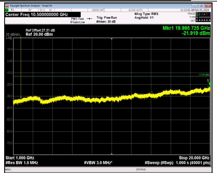
Band66_1.4MHz_16QAM_132322_1RB#0_1000~20000_1000~20000
