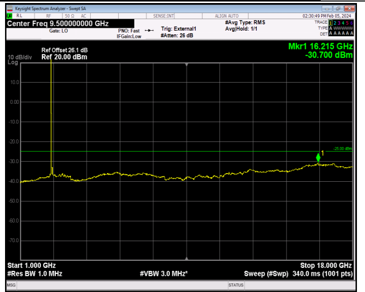
Band41_20MHz_QPSK_40640_1RB#0_1000~18000_1000~18000
