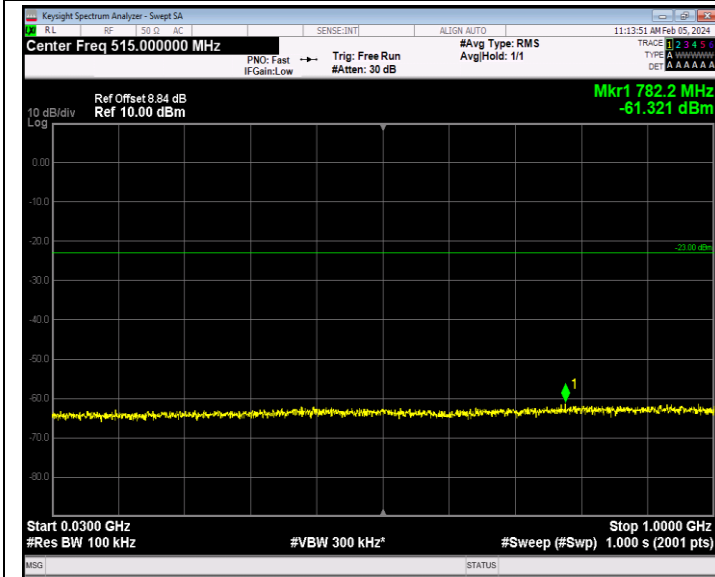
Band66_1.4MHz_64QAM_132322_1RB#0_30~1000_30~1000
