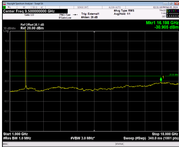
Band41_20MHz_16QAM_40640_1RB#0_1000~18000_1000~18000
