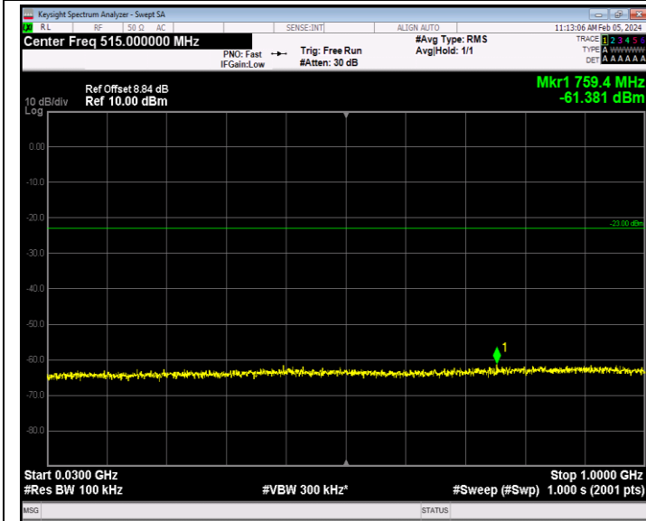
Band66_1.4MHz_QPSK_132322_1RB#0_30~1000_30~1000
