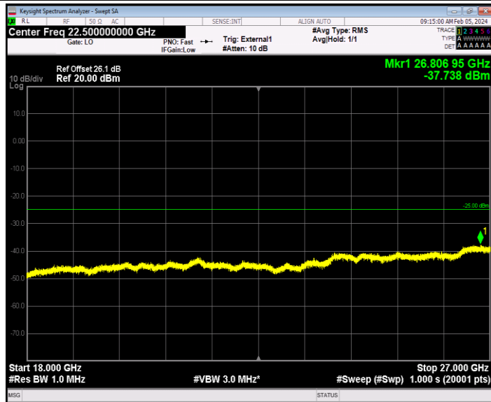
Band41_5MHz_64QAM_40065_1RB#0_18000~27000_18000~27000
