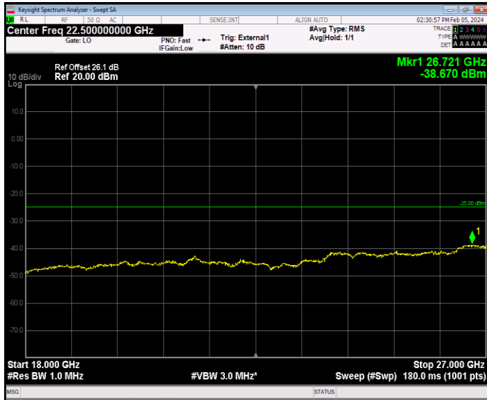
Band41_20MHz_QPSK_40640_1RB#0_18000~27000_18000~27000
