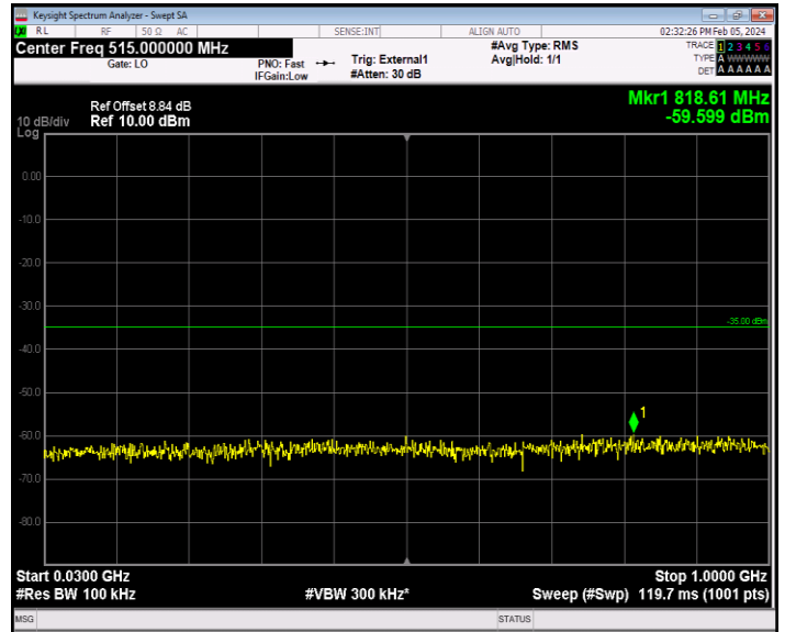
Band41_20MHz_QPSK_41140_1RB#0_30~1000_30~1000
