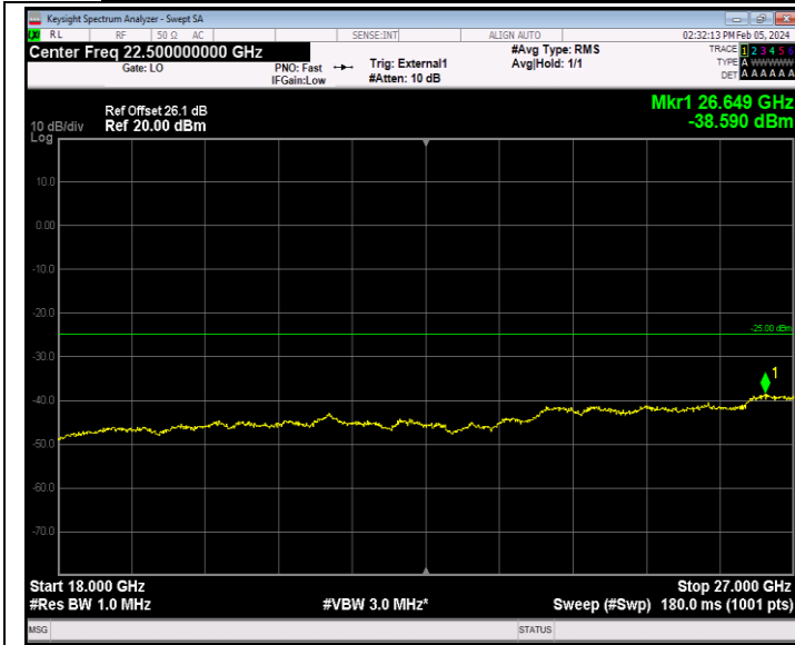
Band41_20MHz_64QAM_40640_1RB#0_18000~27000_18000~27000
