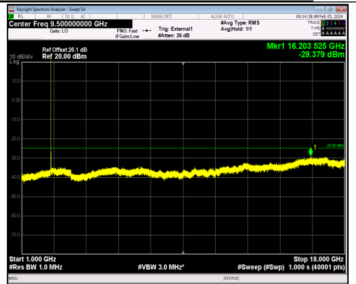
Band41_5MHz_64QAM_40065_1RB#0_1000~18000_1000~18000
