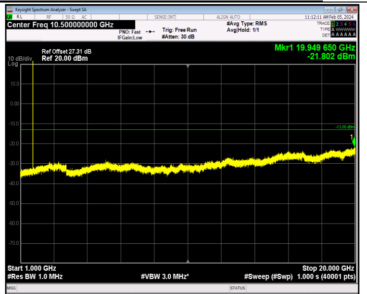
Band66_1.4MHz_QPSK_131979_1RB#0_1000~20000_1000~20000
