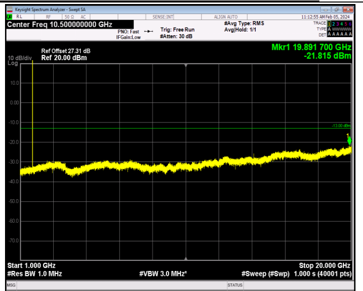
Band66_1.4MHz_64QAM_131979_1RB#0_1000~20000_1000~20000
