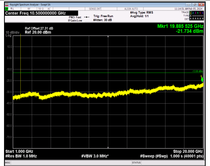
Band66_1.4MHz_16QAM_132665_1RB#0_1000~20000_1000~20000
