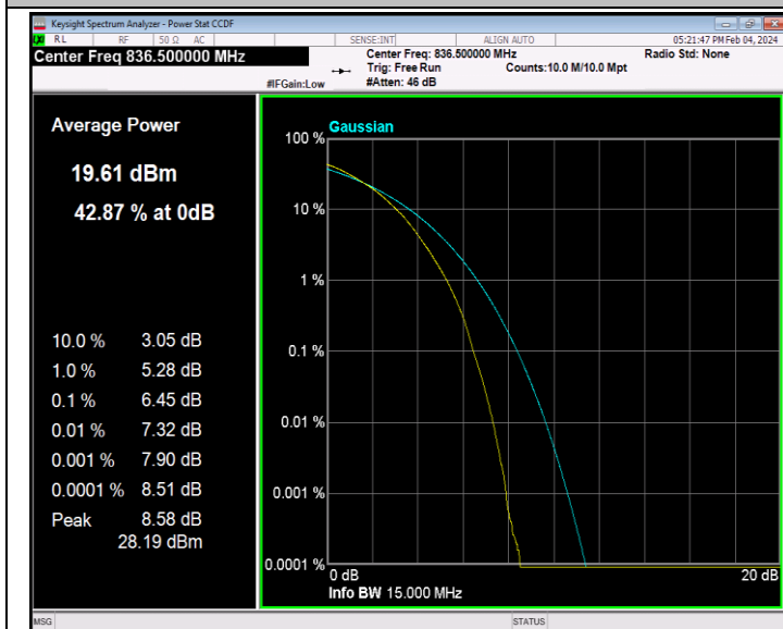
26(824-849)-15MHz-64QAM-26915-75RB#0-PASS
