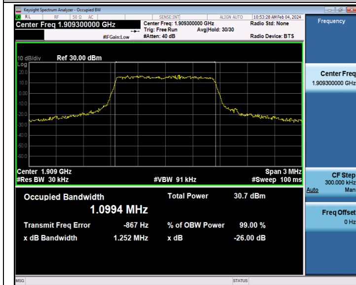
Band2-1.4MHz-QPSK-19193-6RB#0-PASS
