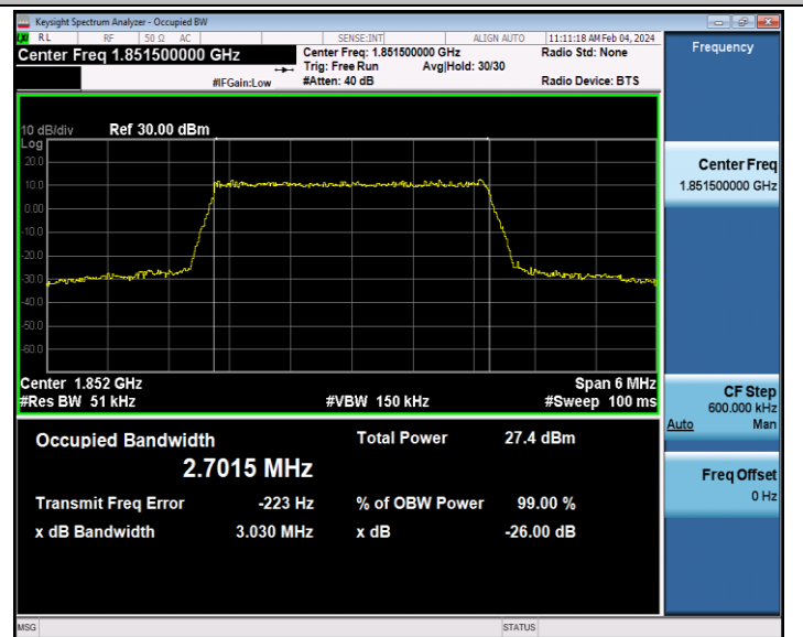
Band2-3MHz-64QAM-18615-15RB#0-PASS
