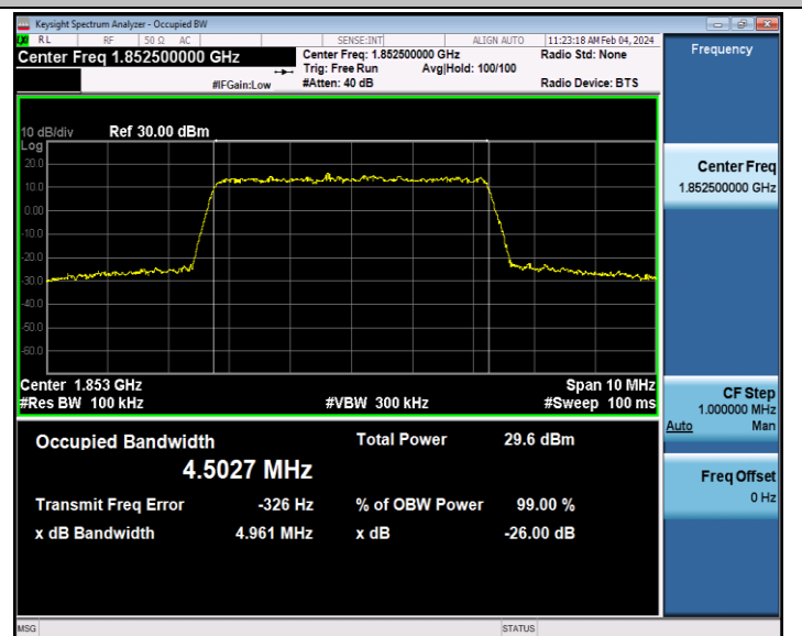
Band2-5MHz-16QAM-18625-25RB#0-PASS
