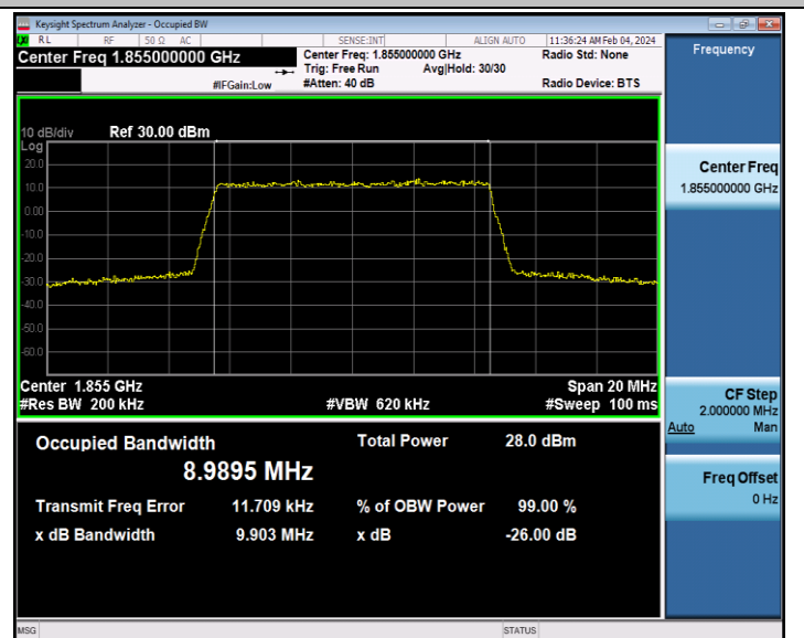
Band2-10MHz-64QAM-18650-50RB#0-PASS
