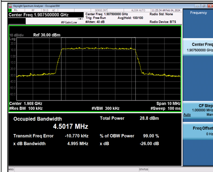
Band2-5MHz-64QAM-19175-25RB#0-PASS
