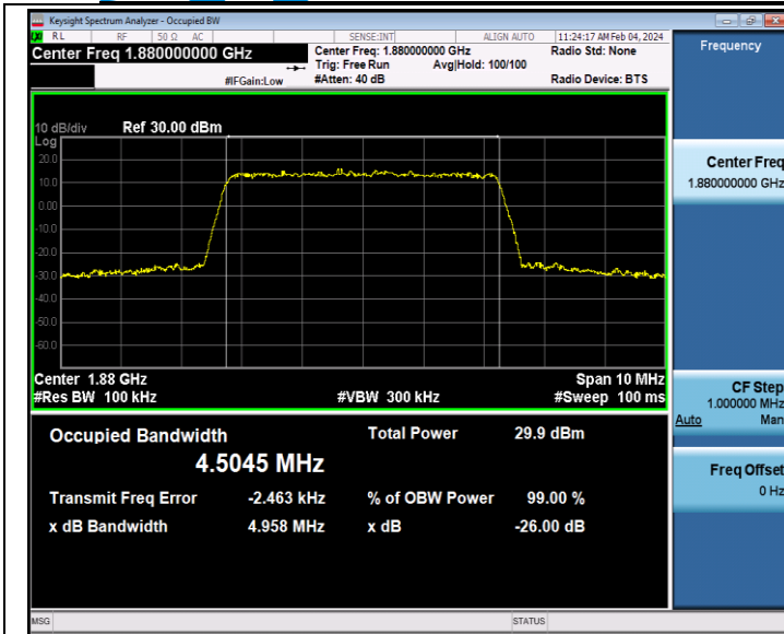
Band2-5MHz-16QAM-18900-25RB#0-PASS
