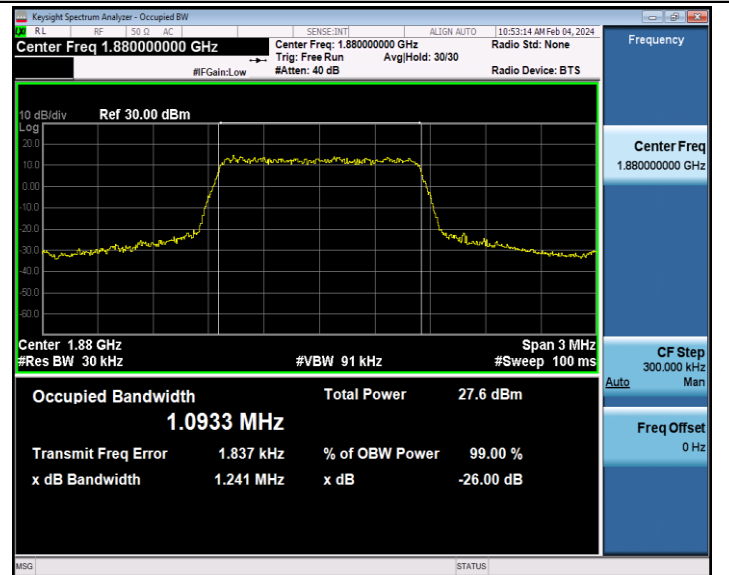
Band2-1.4MHz-16QAM-18800-6RB#0-PASS
