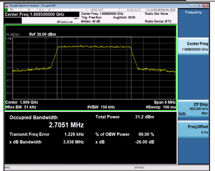
Band2-3MHz-QPSK-19185-15RB#0-PASS
