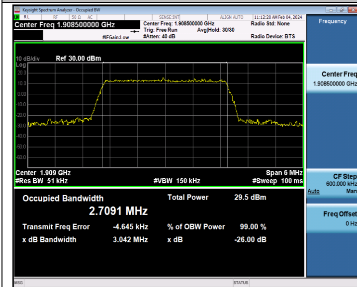
Band2-3MHz-16QAM-19185-15RB#0-PASS
