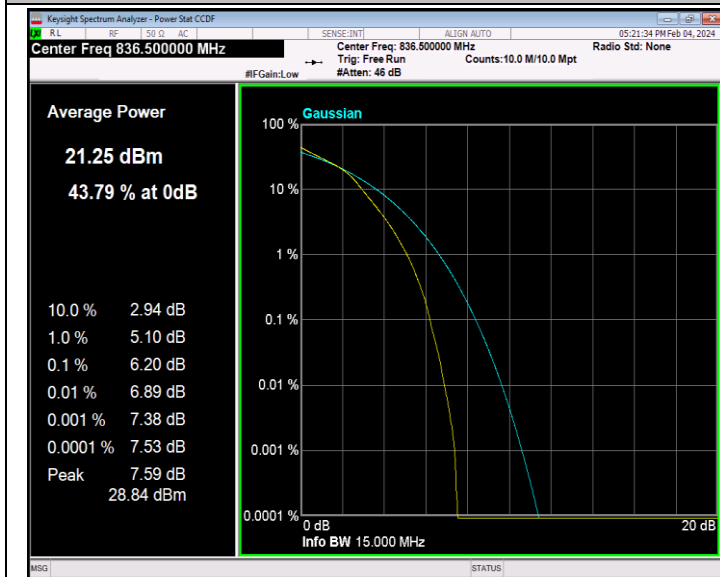
26(824-849)-15MHz-16QAM-26915-75RB#0-PASS
