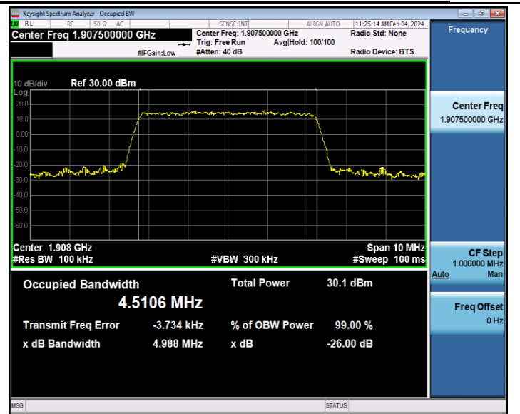
Band2-5MHz-16QAM-19175-25RB#0-PASS
