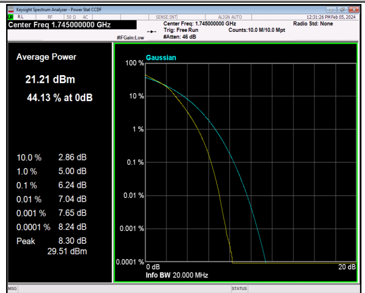
Band66-20MHz-16QAM-132322-100RB#0-PASS
