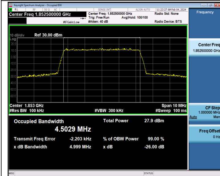
Band2-5MHz-64QAM-18625-25RB#0-PASS
