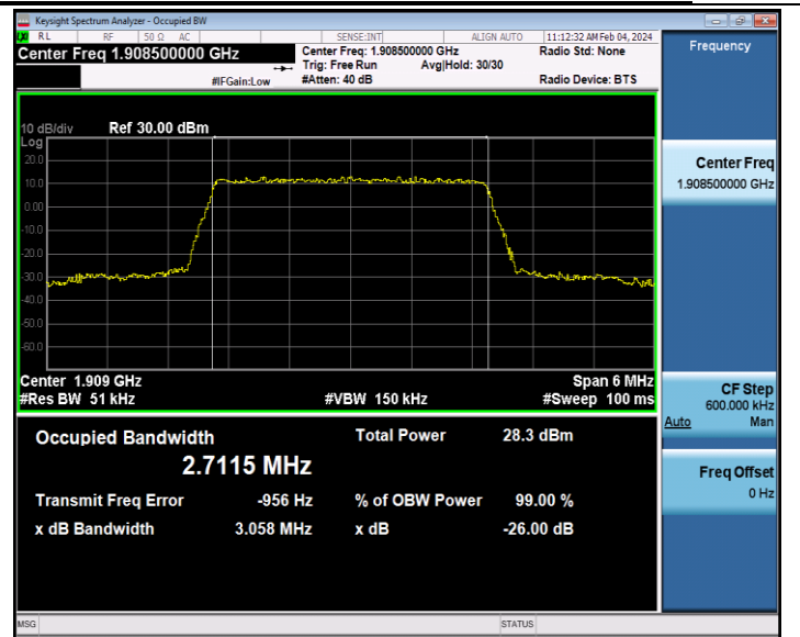
Band2-3MHz-64QAM-19185-15RB#0-PASS
