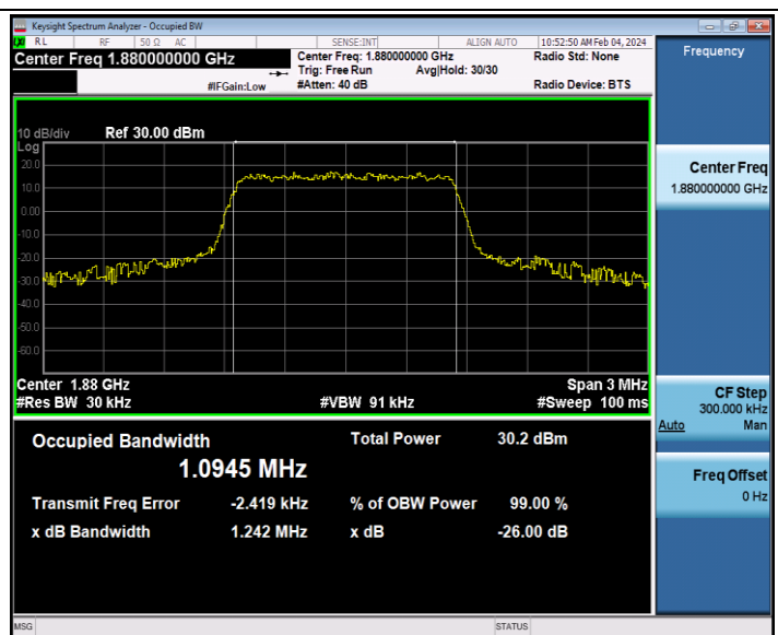
Band2-1.4MHz-QPSK-18900-6RB#0-PASS
