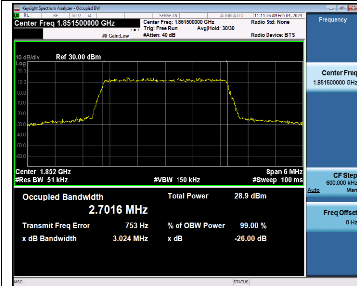
Band2-3MHz-16QAM-18615-15RB#0-PASS
