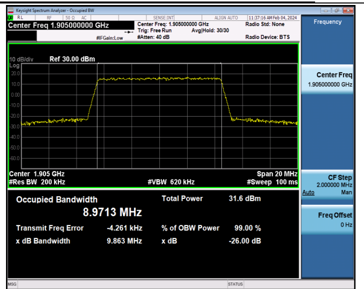
Band2-10MHz-QPSK-19150-50RB#0-PASS
