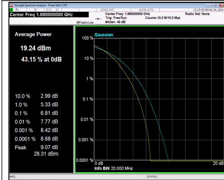
Band2-20MHz-64QAM-18900-100RB#0-PASS
