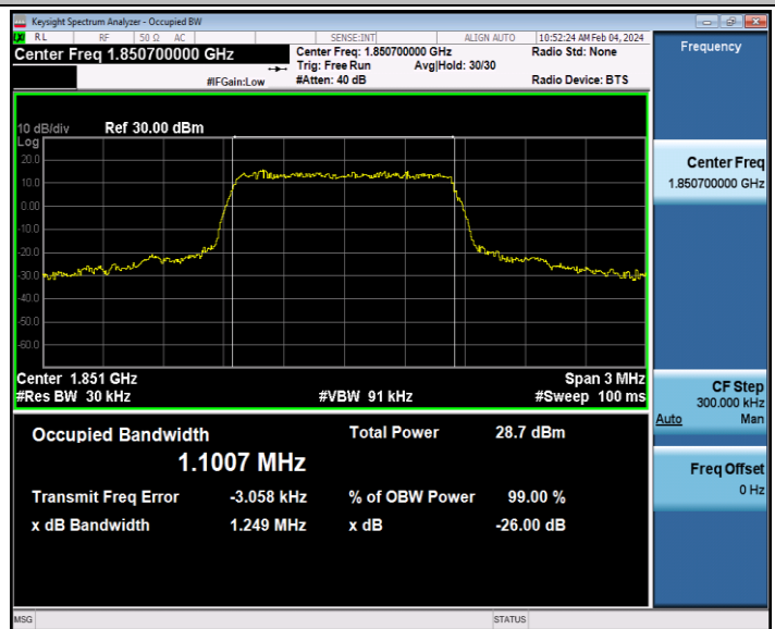
Band2-1.4MHz-16QAM-18607-6RB#0-PASS
