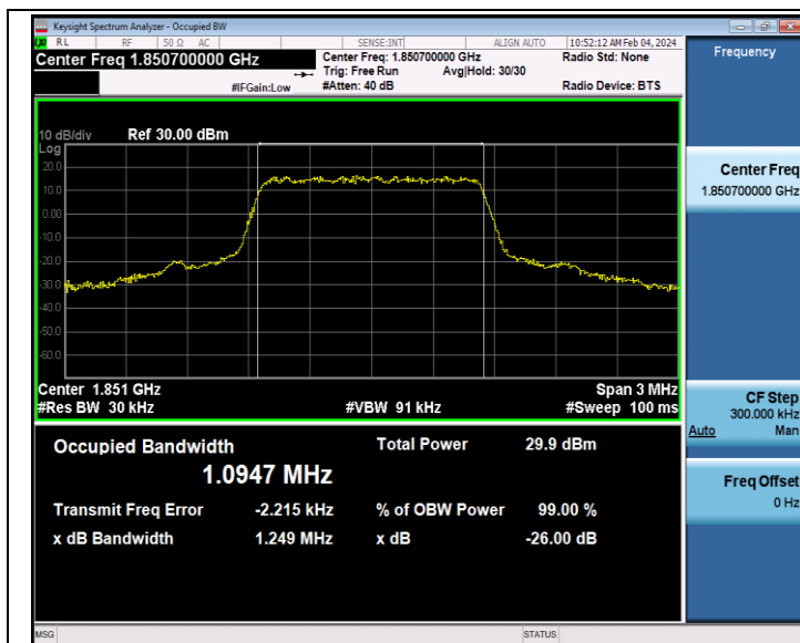
Band2-1.4MHz-QPSK-18607-6RB#0-PASS
