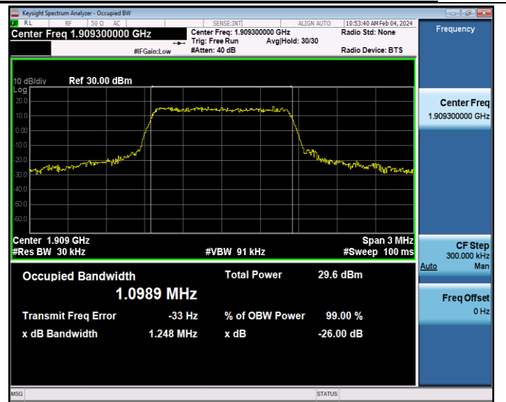
Band2-1.4MHz-16QAM-19193-6RB#0-PASS
