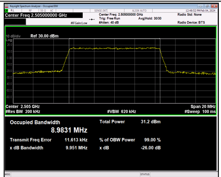
Band7-10MHz-QPSK-20800-50RB#0-PASS
