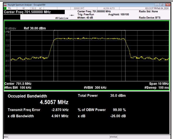
Band12-5MHz-16QAM-23035-25RB#0-PASS
