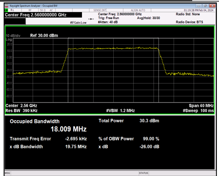
Band7-20MHz-64QAM-21350-100RB#0-PASS
