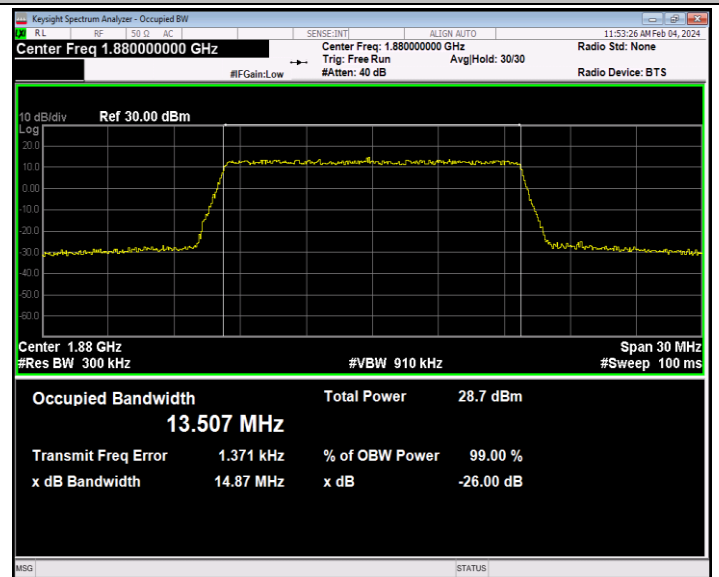
Band2-15MHz-64QAM-18900-75RB#0-PASS
