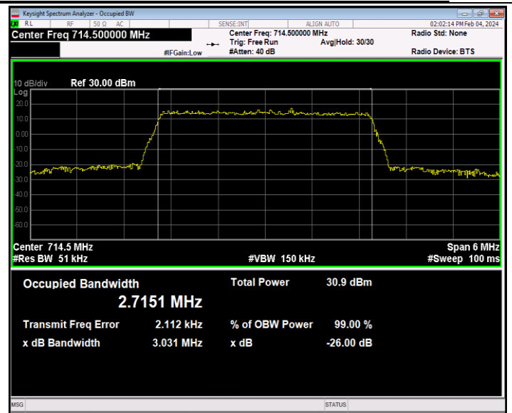
Band12-3MHz-QPSK-23165-15RB#0-PASS
