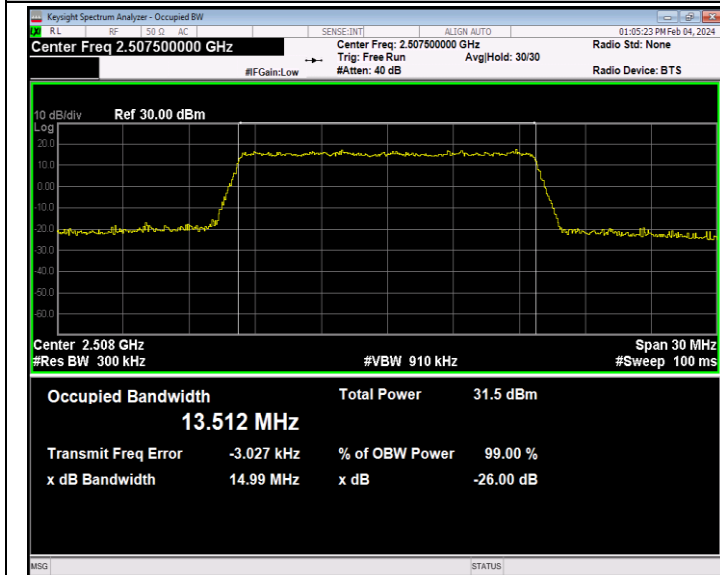
Band7-15MHz-QPSK-20825-75RB#0-PASS
