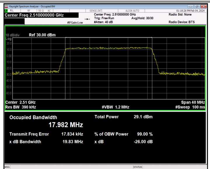
Band7-20MHz-64QAM-20850-100RB#0-PASS
