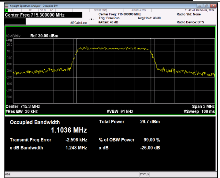
Band12-1.4MHz-16QAM-23173-6RB#0-PASS
