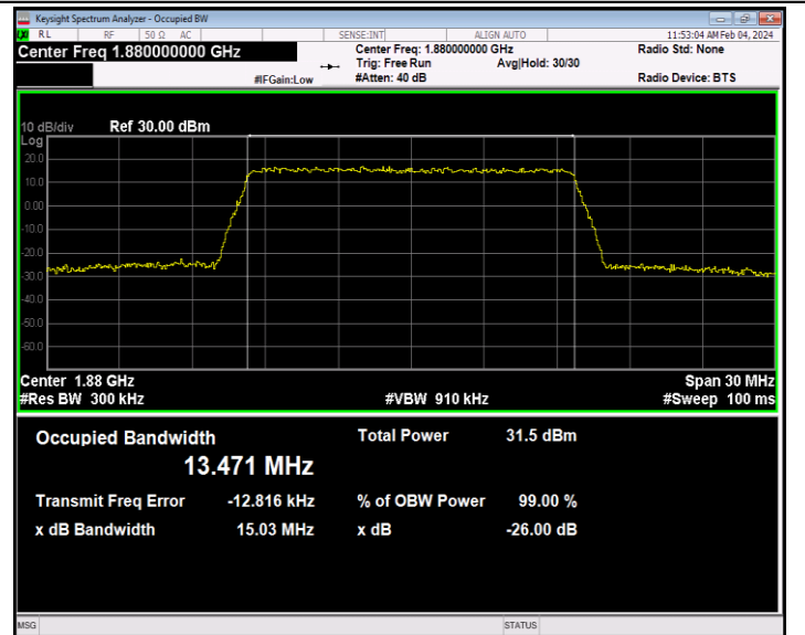
Band2-15MHz-QPSK-18900-75RB#0-PASS
