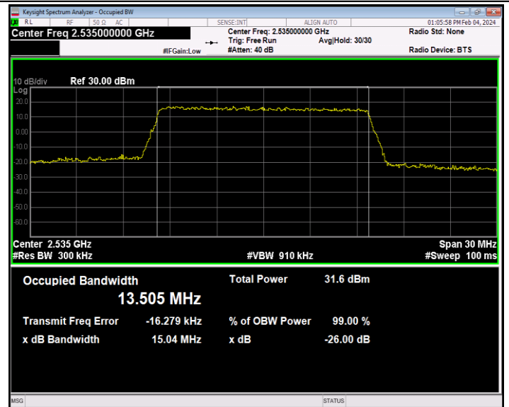
Band7-15MHz-QPSK-21100-75RB#0-PASS
