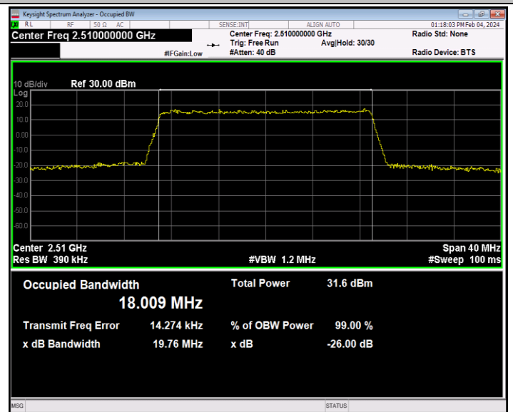
Band7-20MHz-QPSK-20850-100RB#0-PASS
