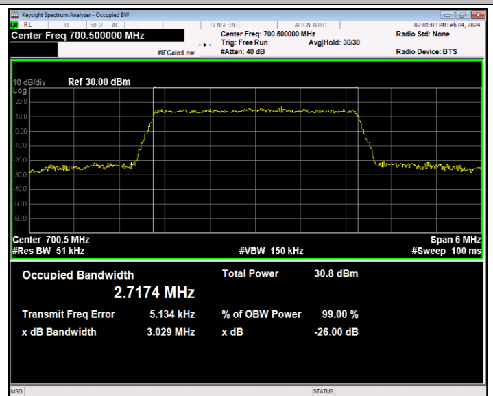
Band12-3MHz-QPSK-23025-15RB#0-PASS
