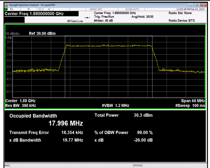
Band2-20MHz-16QAM-18900-100RB#0-PASS
