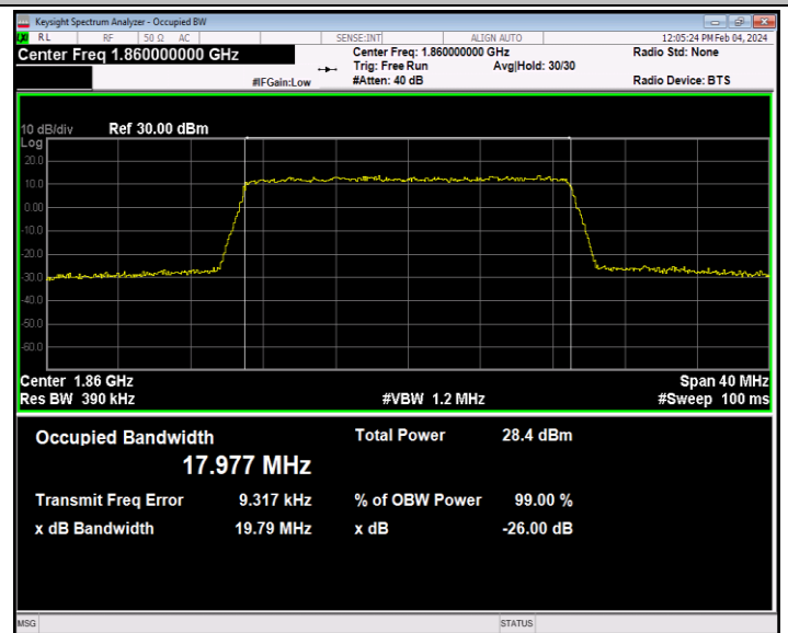
Band2-20MHz-64QAM-18700-100RB#0-PASS
