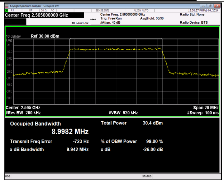
Band7-10MHz-64QAM-21400-50RB#0-PASS
