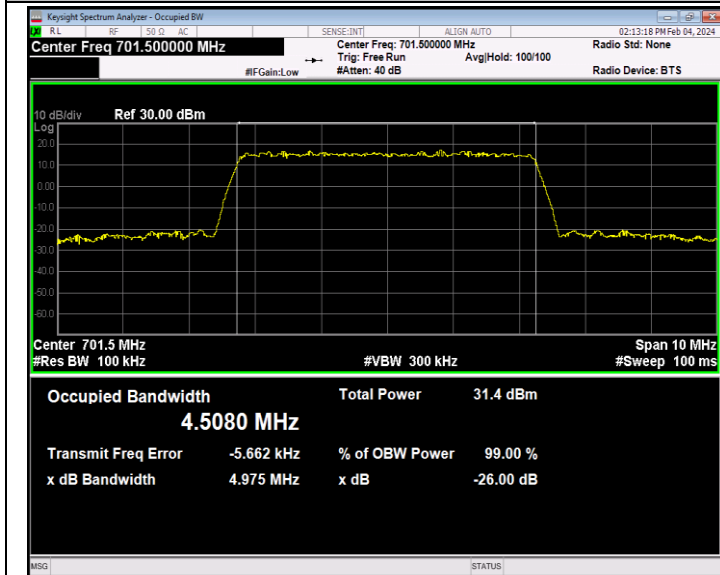
Band12-5MHz-QPSK-23035-25RB#0-PASS
