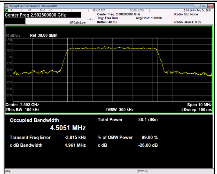
Band7-5MHz-16QAM-20775-25RB#0-PASS
