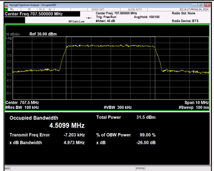
Band12-5MHz-QPSK-23095-25RB#0-PASS
