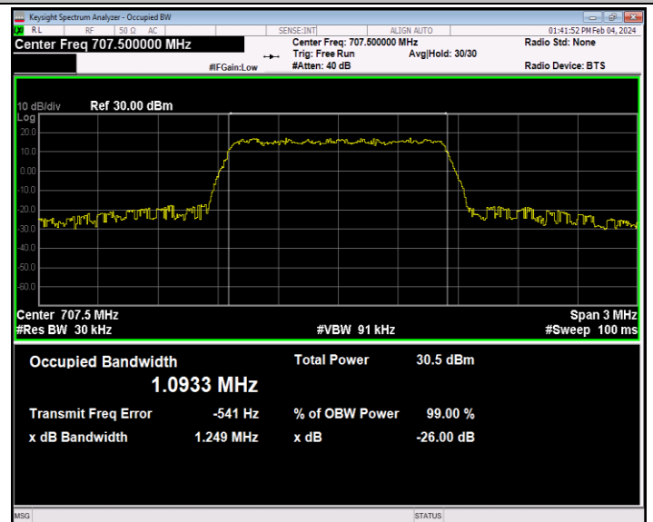
Band12-1.4MHz-QPSK-23095-6RB#0-PASS
