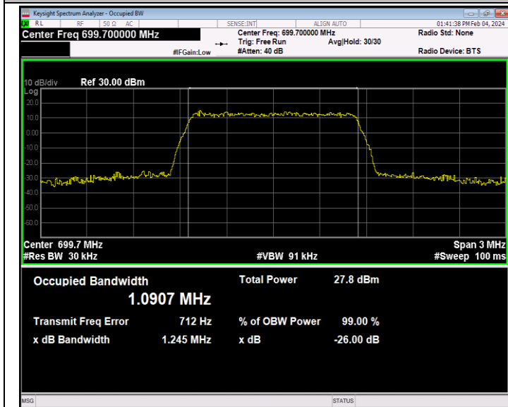
Band12-1.4MHz-64QAM-23017-6RB#0-PASS
