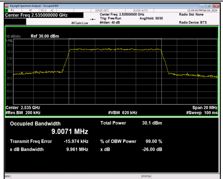
Band7-10MHz-16QAM-21100-50RB#0-PASS
