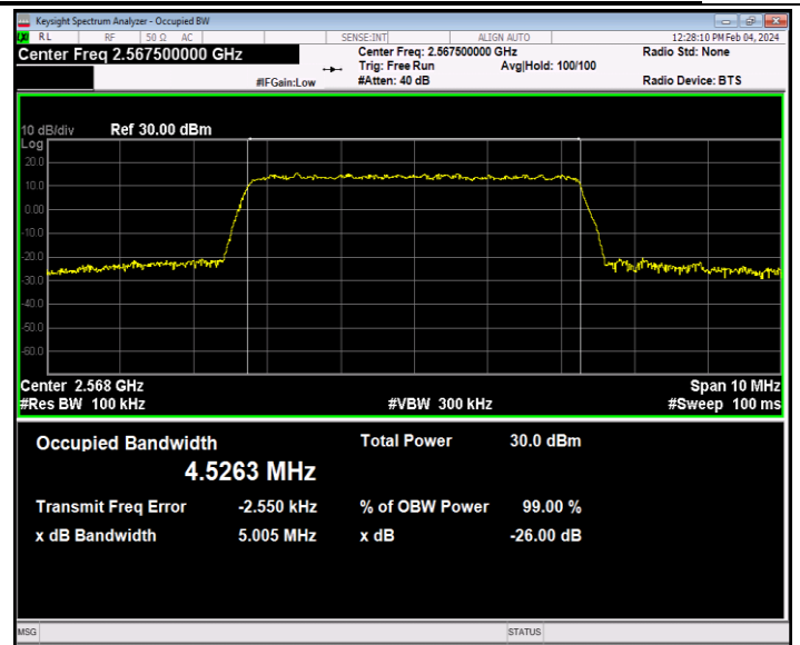
Band7-5MHz-16QAM-21425-25RB#0-PASS
