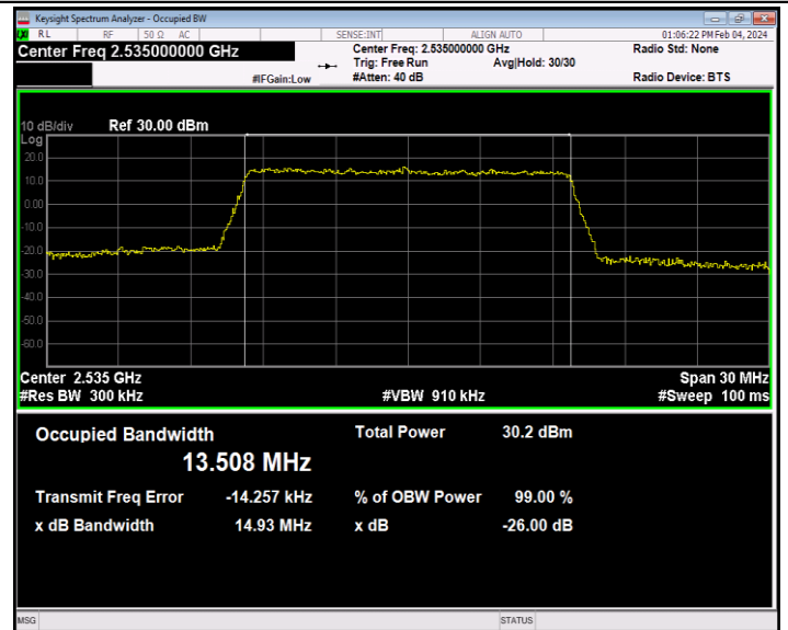
Band7-15MHz-64QAM-21100-75RB#0-PASS
