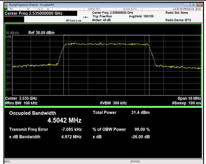
Band7-5MHz-QPSK-21100-25RB#0-PASS
