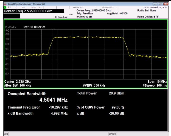
Band7-5MHz-64QAM-21100-25RB#0-PASS
