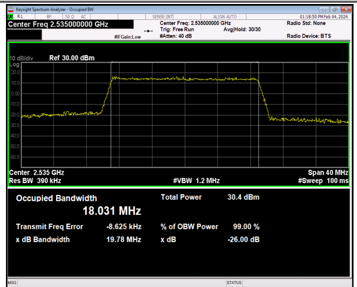
Band7-20MHz-16QAM-21100-100RB#0-PASS
