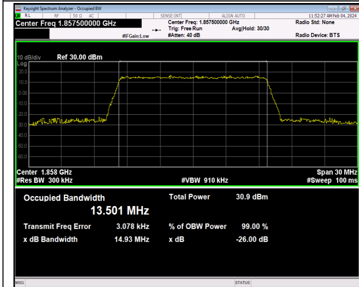
Band2-15MHz-QPSK-18675-75RB#0-PASS
