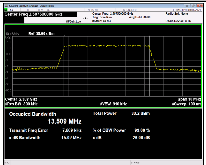
Band7-15MHz-16QAM-20825-75RB#0-PASS
