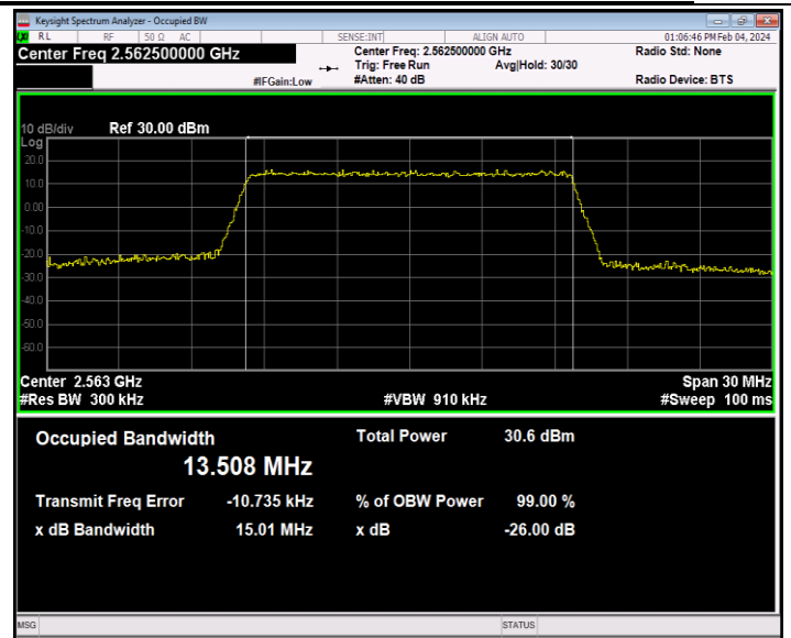
Band7-15MHz-16QAM-21375-75RB#0-PASS
