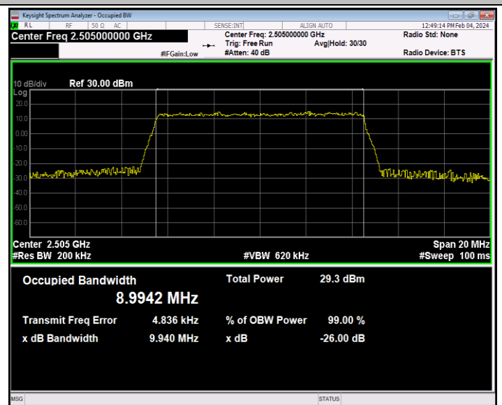
Band7-10MHz-64QAM-20800-50RB#0-PASS
