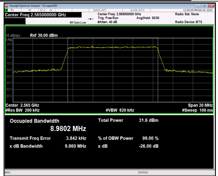
Band7-10MHz-QPSK-21400-50RB#0-PASS
