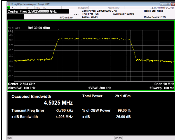
Band7-5MHz-64QAM-20775-25RB#0-PASS
