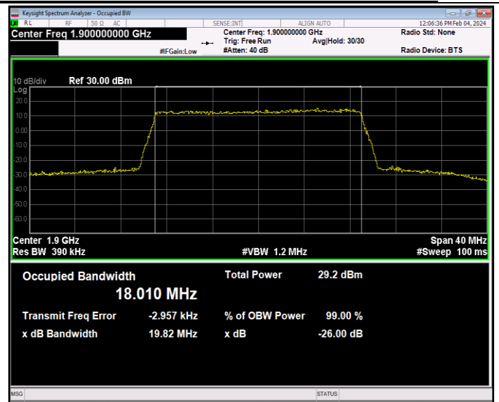
Band2-20MHz-64QAM-19100-100RB#0-PASS
