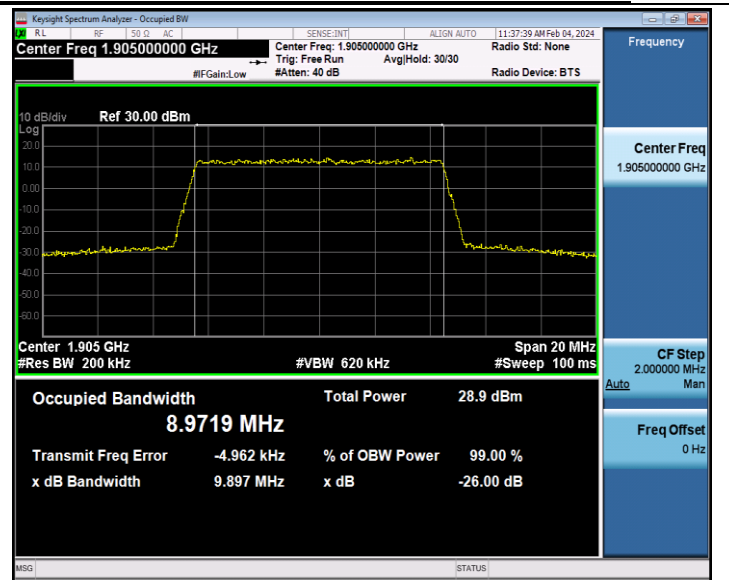
Band2-10MHz-64QAM-19150-50RB#0-PASS
