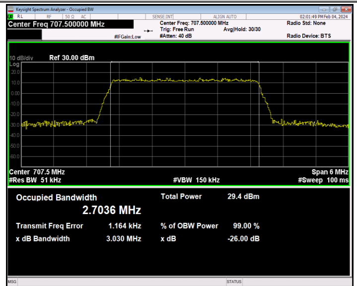
Band12-3MHz-16QAM-23095-15RB#0-PASS
