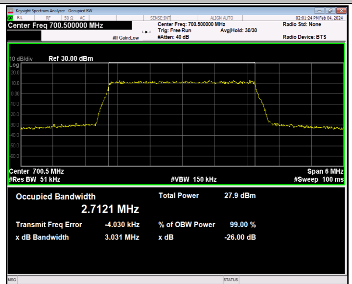
Band12-3MHz-64QAM-23025-15RB#0-PASS
