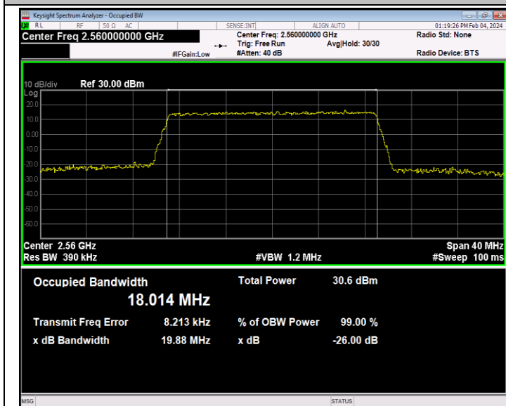
Band7-20MHz-16QAM-21350-100RB#0-PASS
