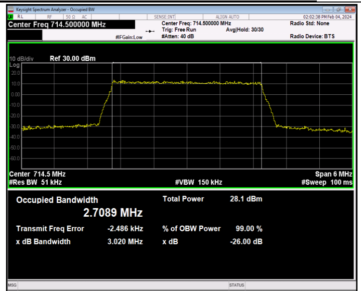
Band12-3MHz-64QAM-23165-15RB#0-PASS
