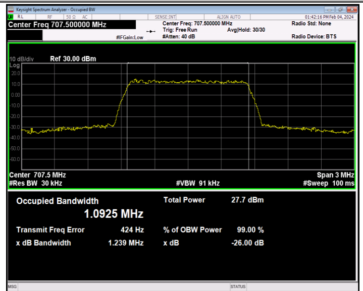
Band12-1.4MHz-64QAM-23095-6RB#0-PASS
