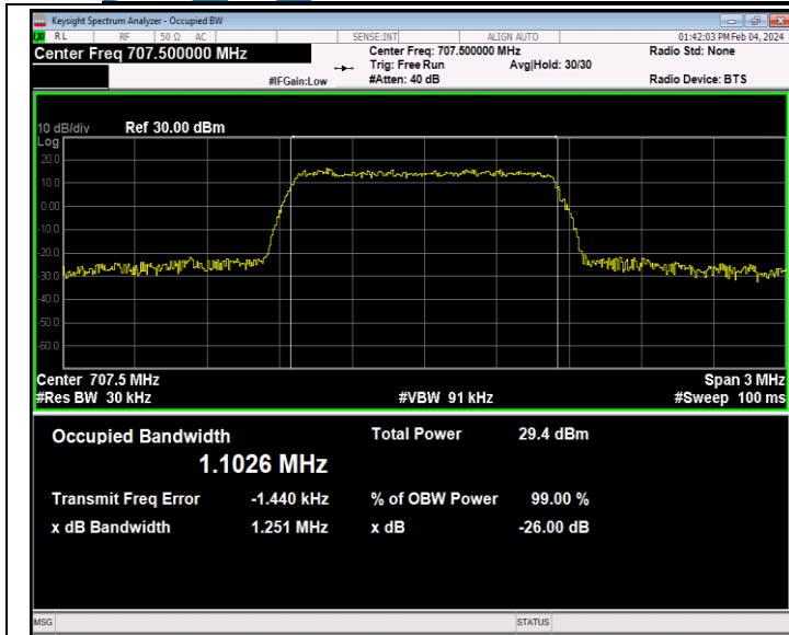
Band12-1.4MHz-16QAM-23095-6RB#0-PASS
