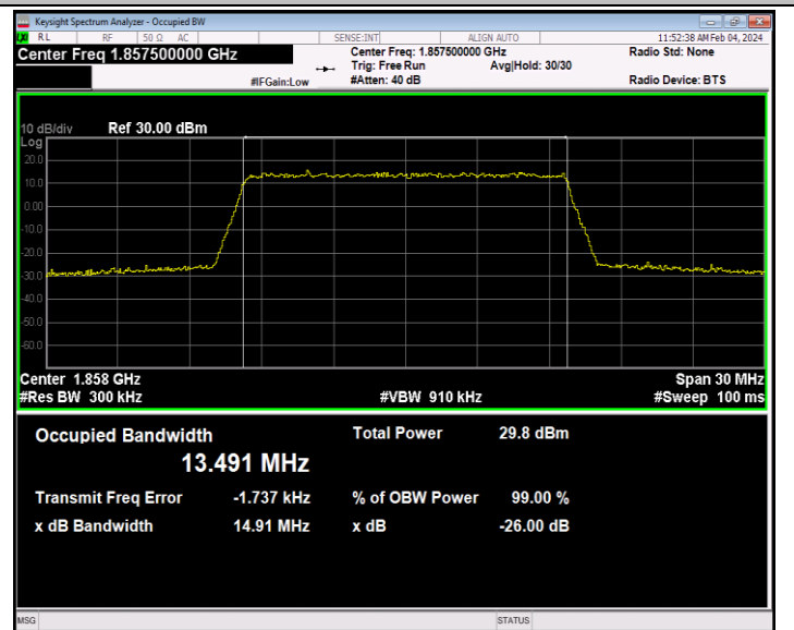
Band2-15MHz-16QAM-18675-75RB#0-PASS
