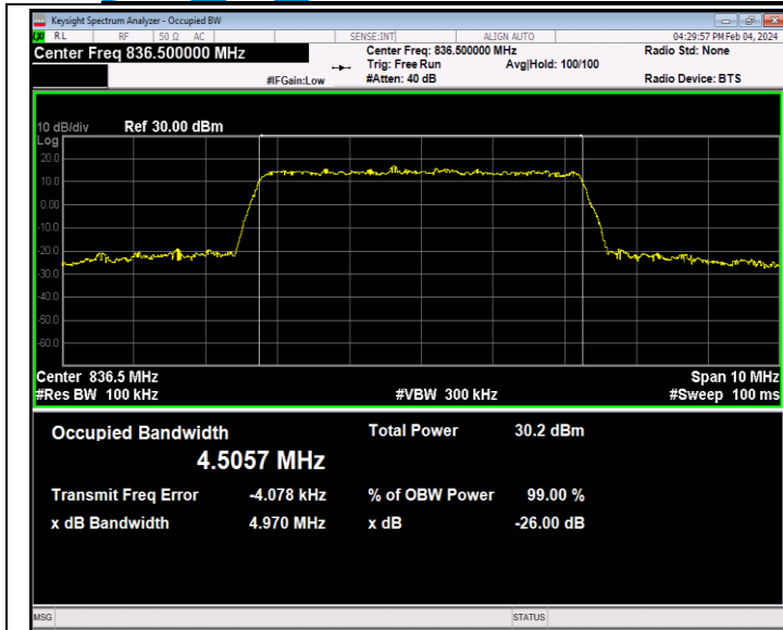
26(824-849)-5MHz-16QAM-26915-25RB#0-PASS
