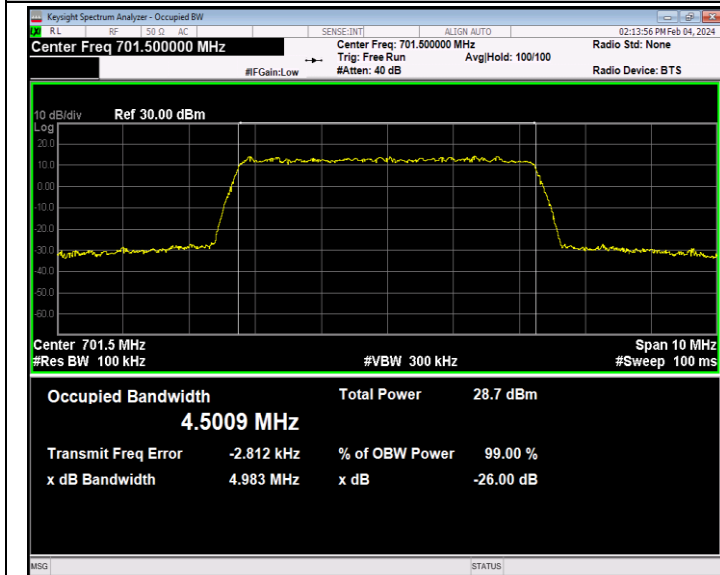
Band12-5MHz-64QAM-23035-25RB#0-PASS
