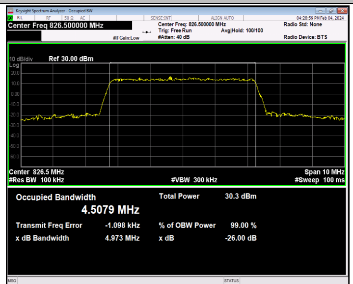
26(824-849)-5MHz-16QAM-26815-25RB#0-PASS
