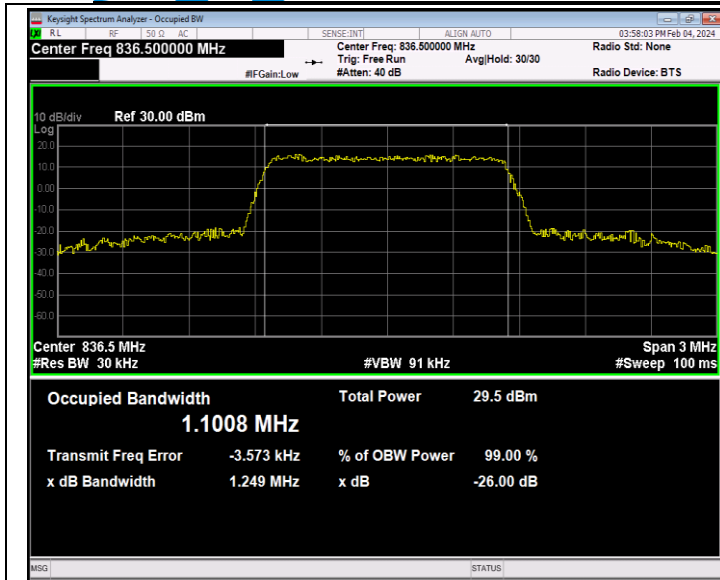
26(824-849)-1.4MHz-16QAM-26915-6RB#0-PASS
