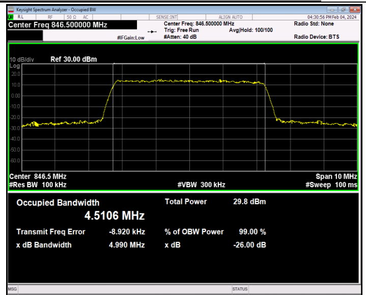
26(824-849)-5MHz-16QAM-27015-25RB#0-PASS
