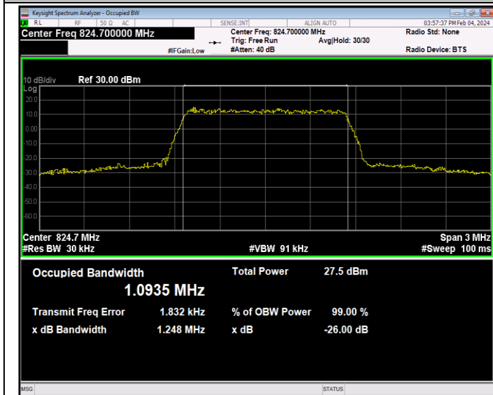
26(824-849)-1.4MHz-64QAM-26797-6RB#0-PASS
