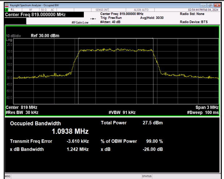
26(814-824)-1.4MHz-64QAM-26740-6RB#0-PASS
