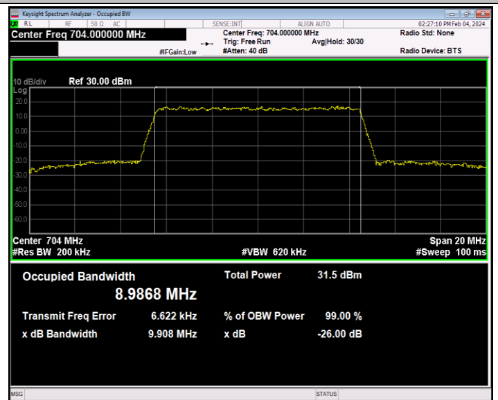
Band12-10MHz-QPSK-23060-50RB#0-PASS
