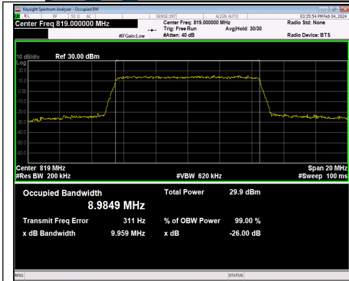
26(814-824)-10MHz-16QAM-26740-50RB#0-PASS
