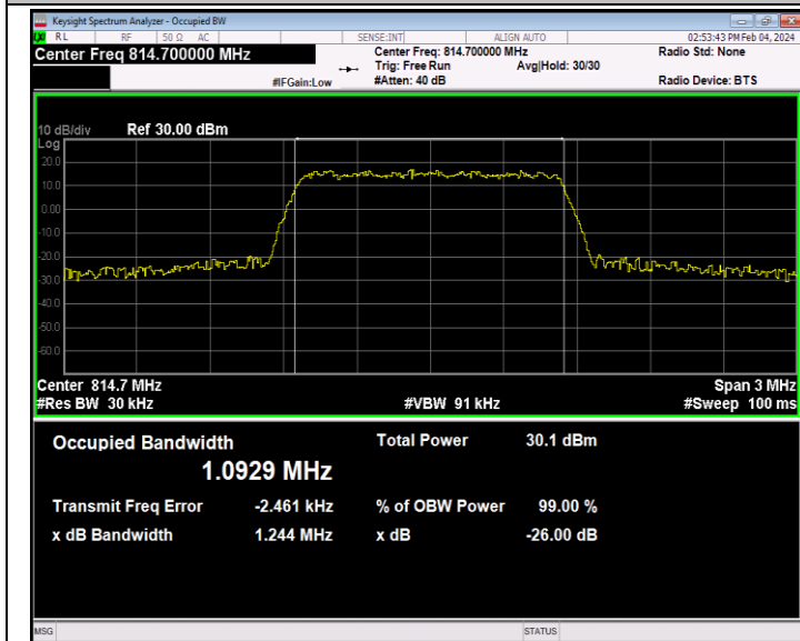
26(814-824)-1.4MHz-QPSK-26697-6RB#0-PASS
