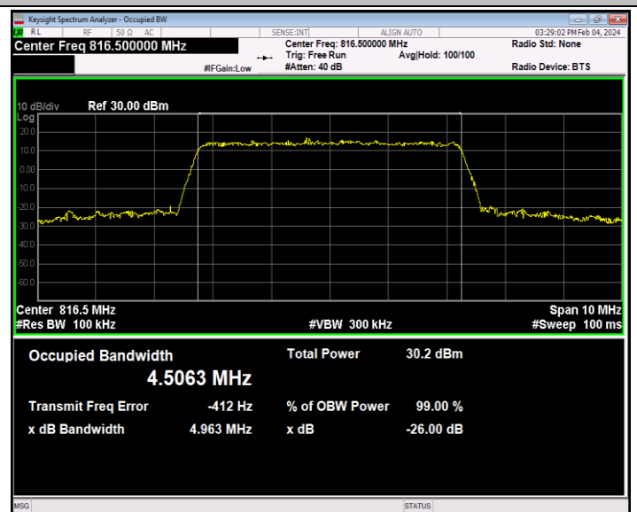
26(814-824)-5MHz-16QAM-26715-25RB#0-PASS
