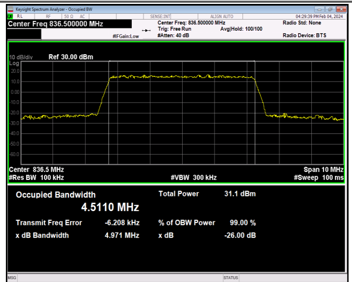
26(824-849)-5MHz-QPSK-26915-25RB#0-PASS
