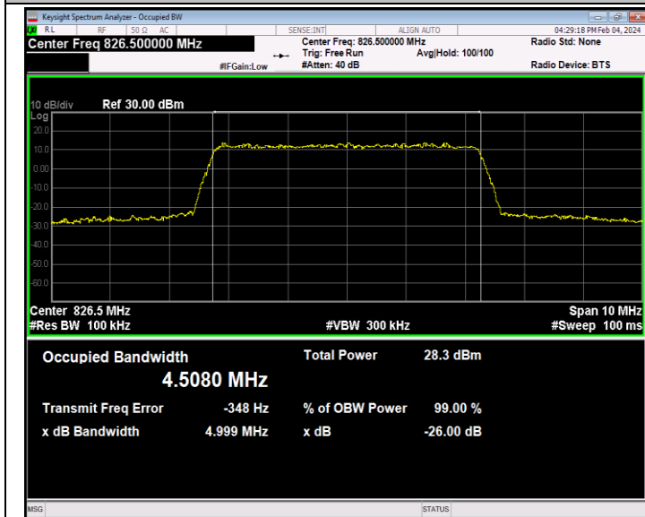
26(824-849)-5MHz-64QAM-26815-25RB#0-PASS
