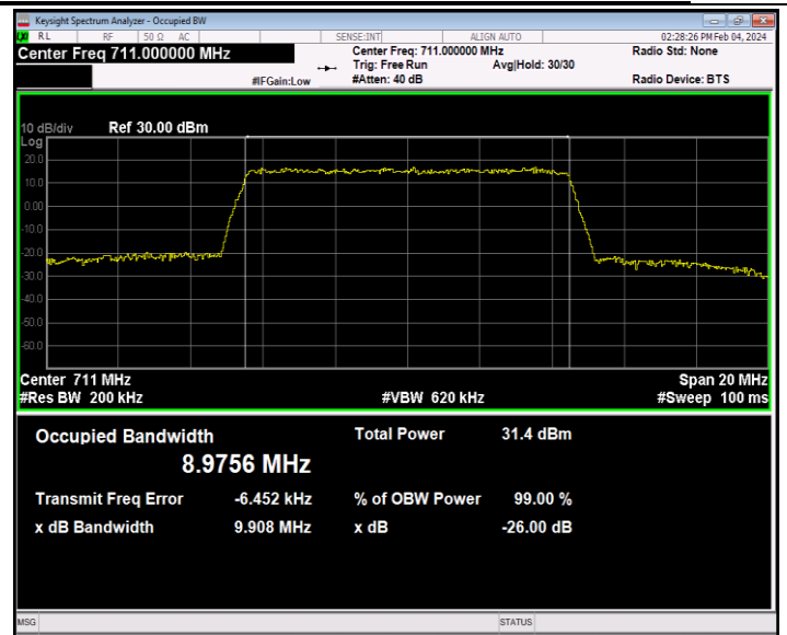
Band12-10MHz-QPSK-23130-50RB#0-PASS
