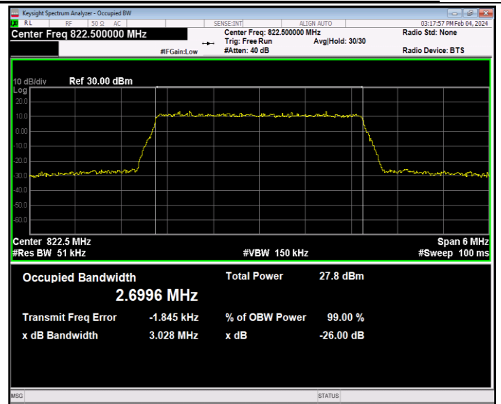
26(814-824)-3MHz-64QAM-26775-15RB#0-PASS
