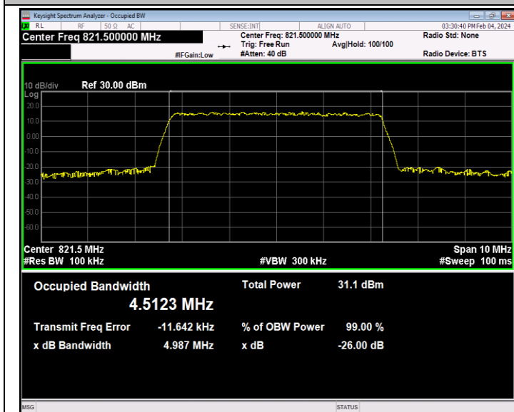
26(814-824)-5MHz-QPSK-26765-25RB#0-PASS
