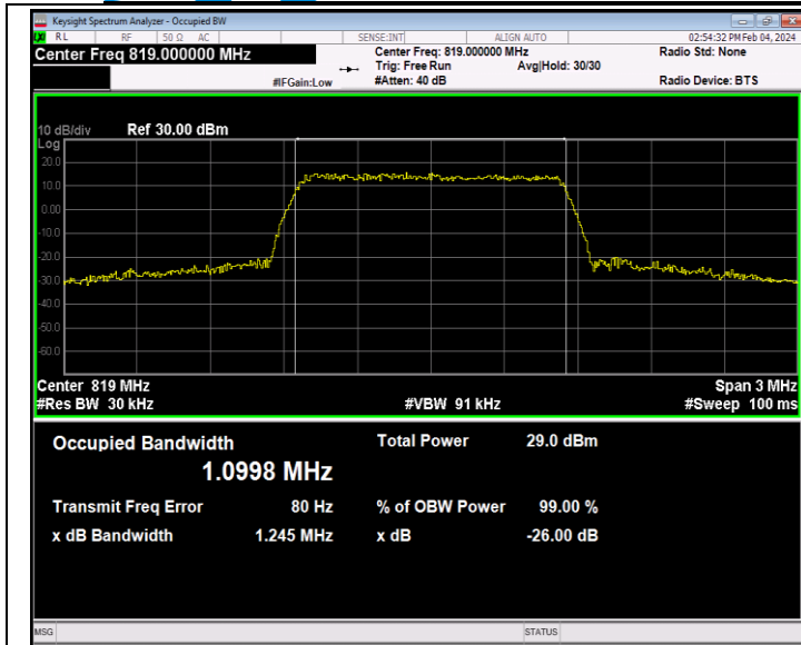
26(814-824)-1.4MHz-16QAM-26740-6RB#0-PASS
