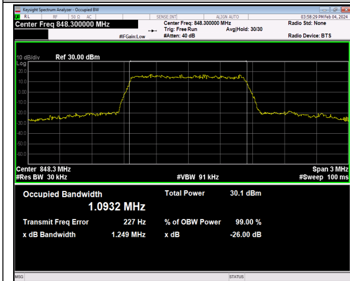
26(824-849)-1.4MHz-QPSK-27033-6RB#0-PASS
