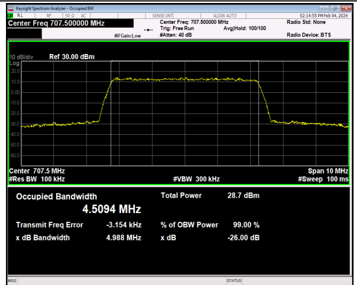
Band12-5MHz-64QAM-23095-25RB#0-PASS
