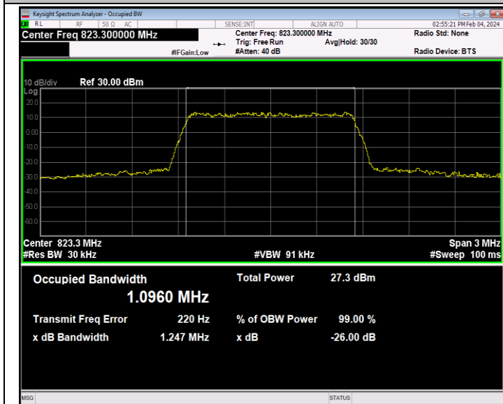
26(814-824)-1.4MHz-64QAM-26783-6RB#0-PASS
