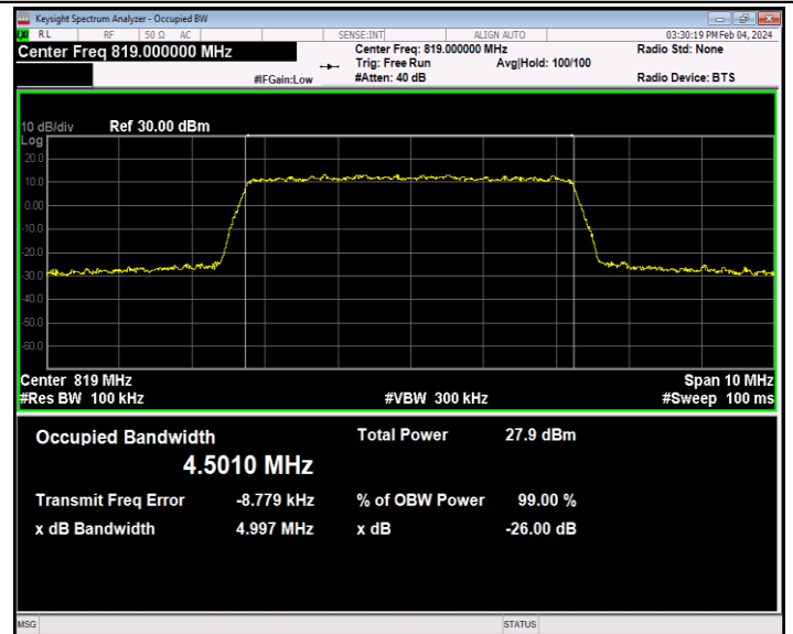
26(814-824)-5MHz-64QAM-26740-25RB#0-PASS
