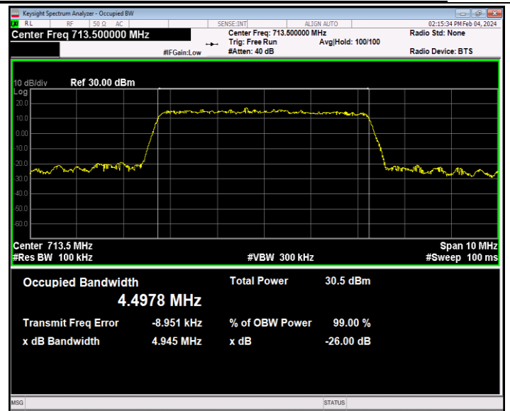
Band12-5MHz-16QAM-23155-25RB#0-PASS
