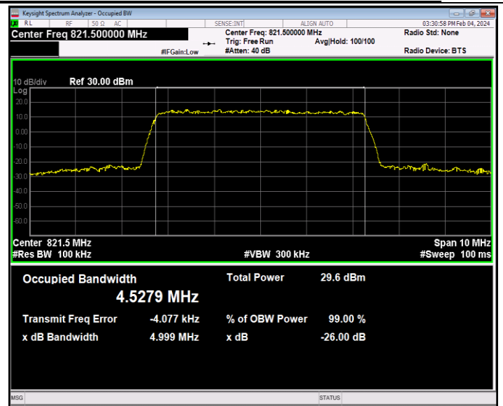
26(814-824)-5MHz-16QAM-26765-25RB#0-PASS
