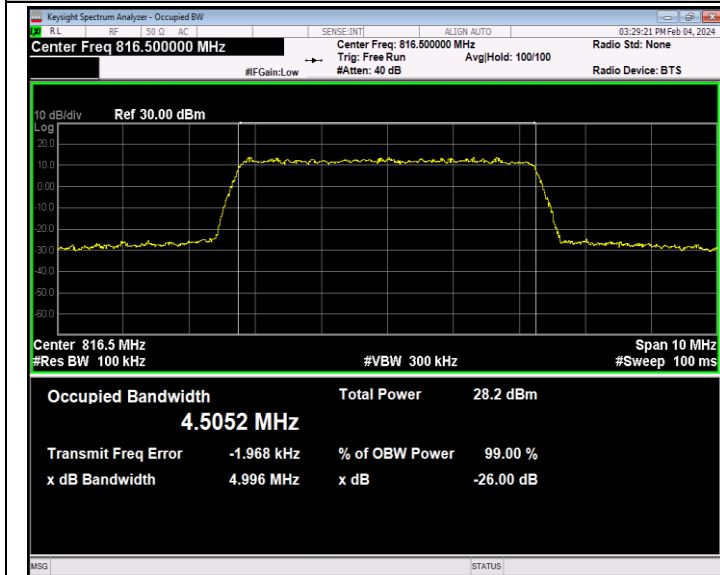
26(814-824)-5MHz-64QAM-26715-25RB#0-PASS
