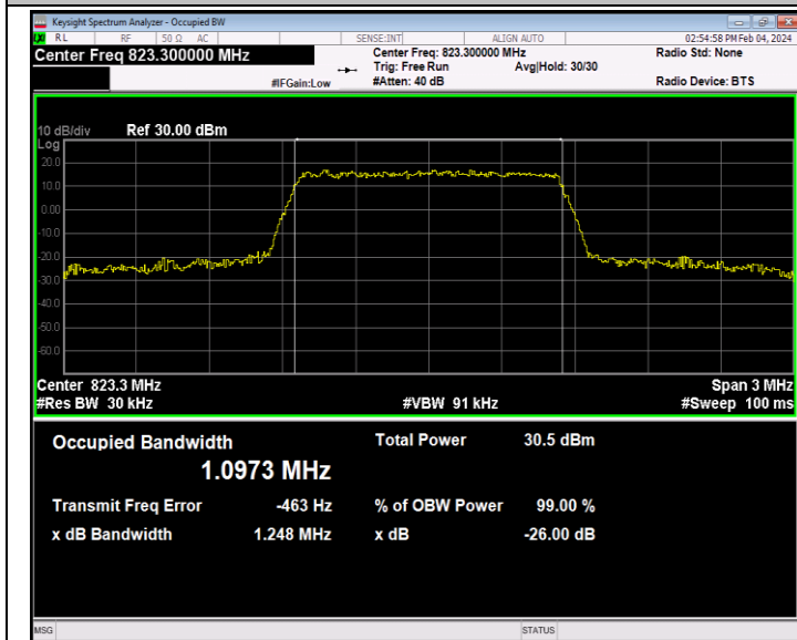
26(814-824)-1.4MHz-QPSK-26783-6RB#0-PASS
