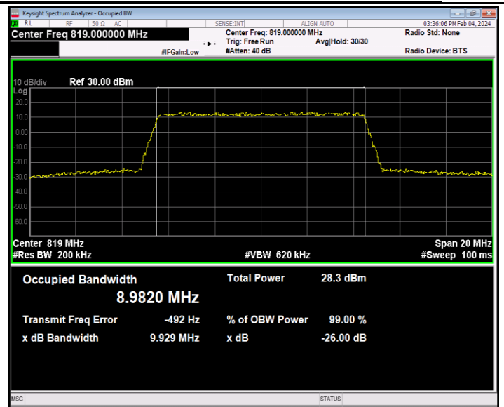
26(814-824)-10MHz-64QAM-26740-50RB#0-PASS
