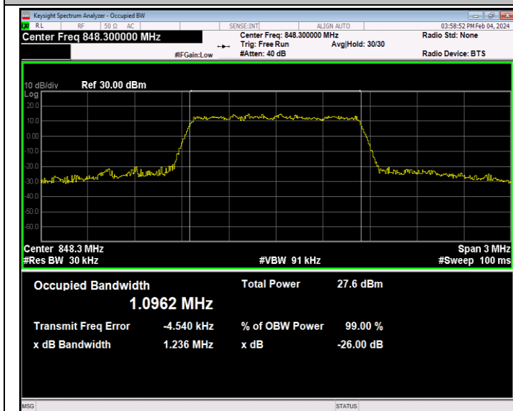
26(824-849)-1.4MHz-64QAM-27033-6RB#0-PASS
