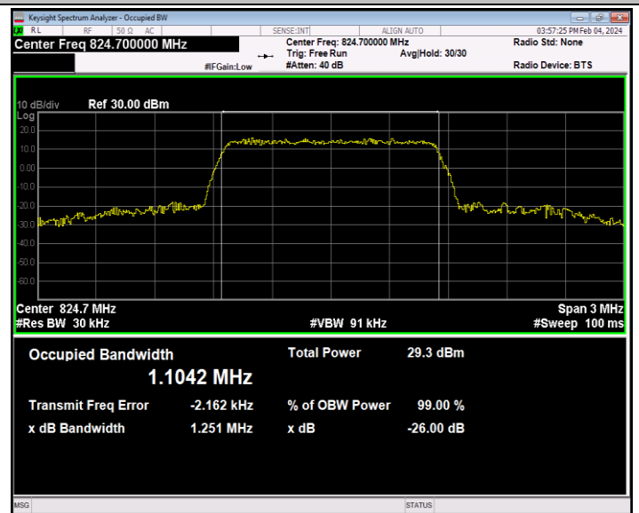
26(824-849)-1.4MHz-16QAM-26797-6RB#0-PASS
