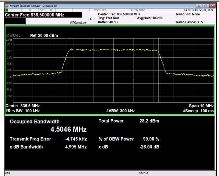
26(824-849)-5MHz-64QAM-26915-25RB#0-PASS
