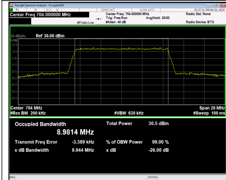
Band12-10MHz-16QAM-23060-50RB#0-PASS
