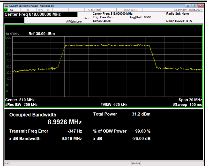
26(814-824)-10MHz-QPSK-26740-50RB#0-PASS
