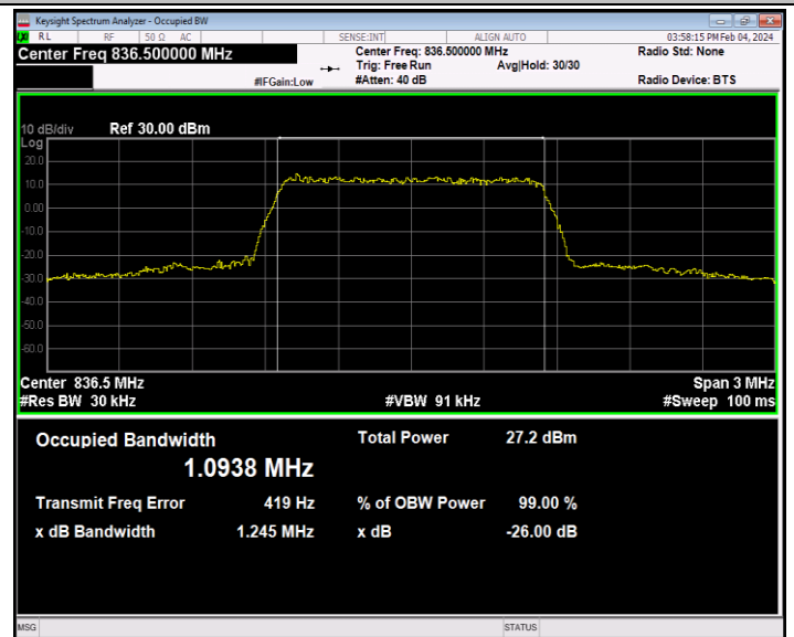
26(824-849)-1.4MHz-64QAM-26915-6RB#0-PASS
