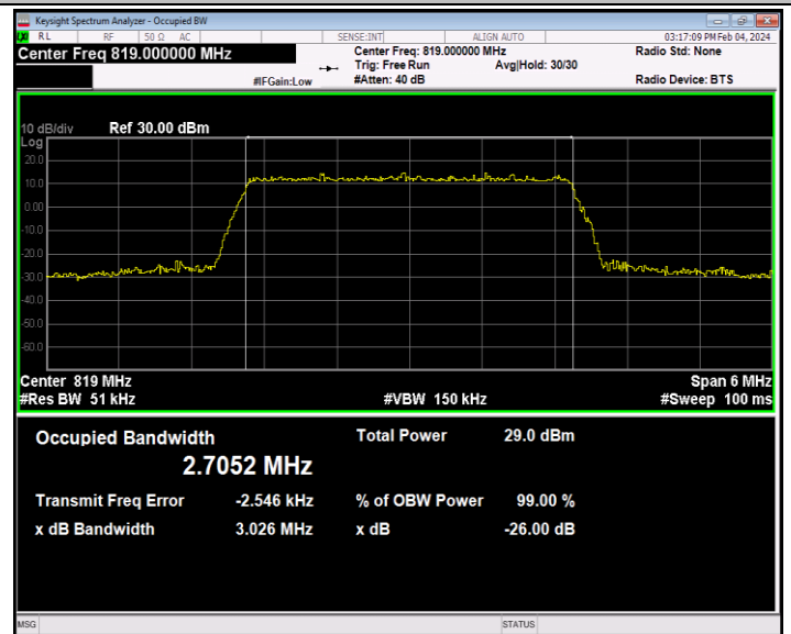
26(814-824)-3MHz-16QAM-26740-15RB#0-PASS
