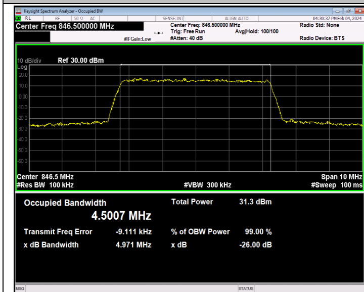
26(824-849)-5MHz-QPSK-27015-25RB#0-PASS
