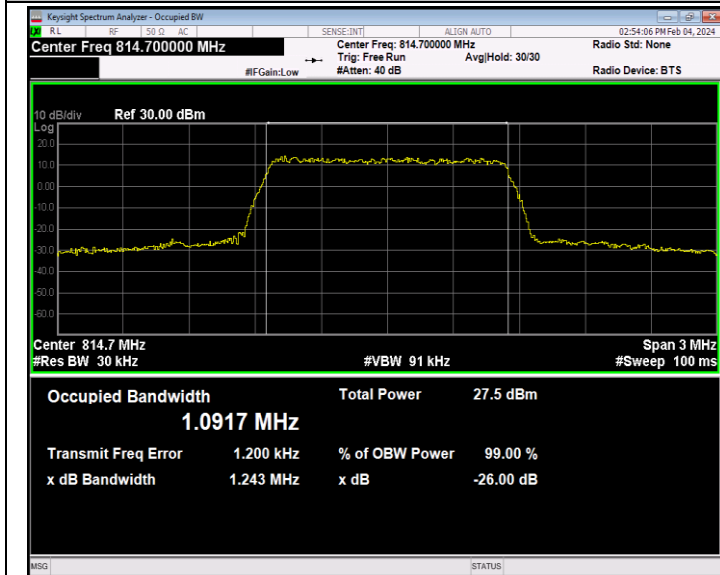
26(814-824)-1.4MHz-64QAM-26697-6RB#0-PASS
