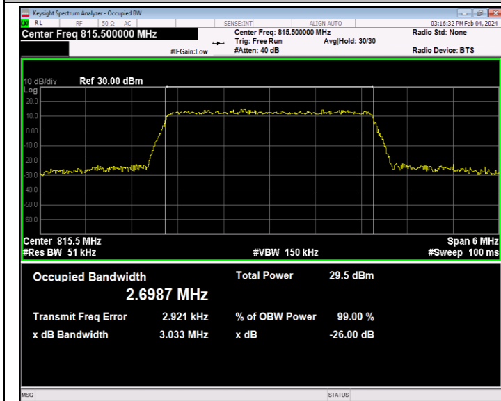
26(814-824)-3MHz-16QAM-26705-15RB#0-PASS
