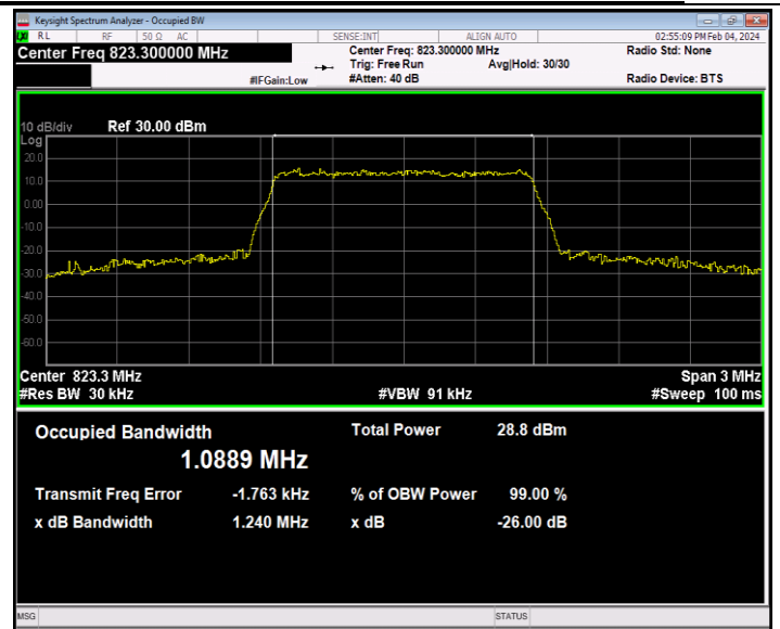
26(814-824)-1.4MHz-16QAM-26783-6RB#0-PASS
