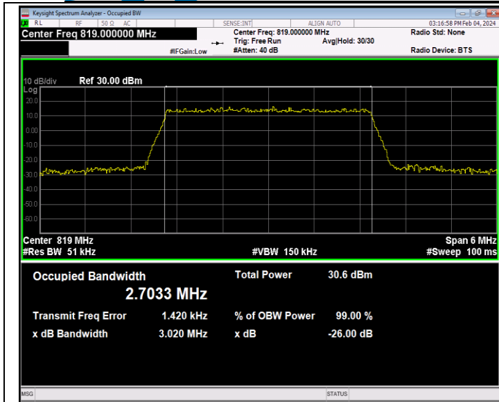
26(814-824)-3MHz-QPSK-26740-15RB#0-PASS
