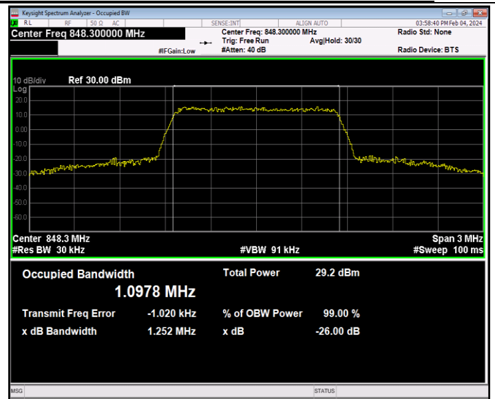
26(824-849)-1.4MHz-16QAM-27033-6RB#0-PASS
