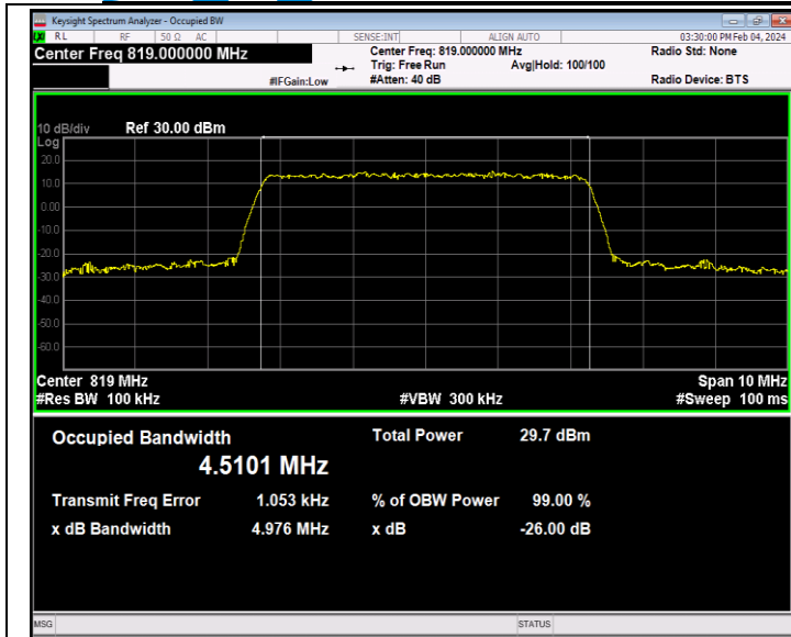
26(814-824)-5MHz-16QAM-26740-25RB#0-PASS
