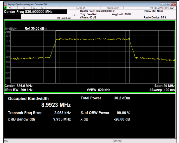
26(824-849)-10MHz-16QAM-26915-50RB#0-PASS
