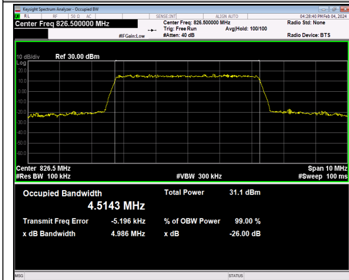
26(824-849)-5MHz-QPSK-26815-25RB#0-PASS
