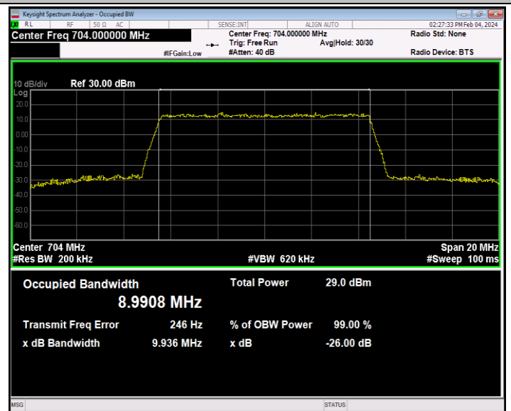
Band12-10MHz-64QAM-23060-50RB#0-PASS
