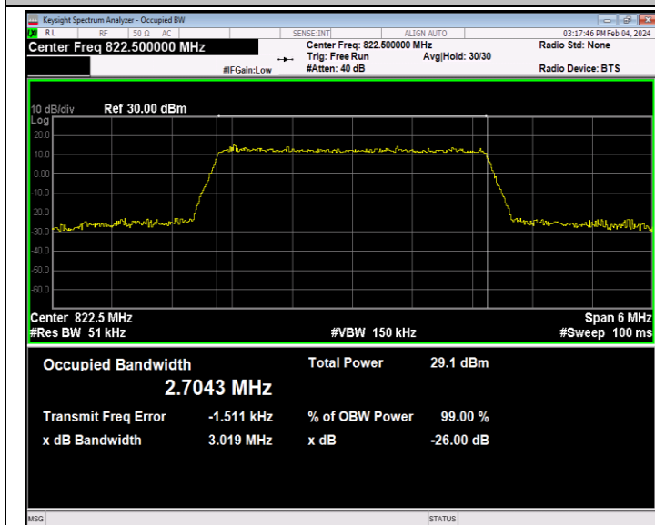
26(814-824)-3MHz-16QAM-26775-15RB#0-PASS
