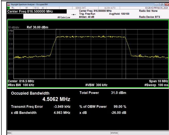
26(814-824)-5MHz-QPSK-26715-25RB#0-PASS
