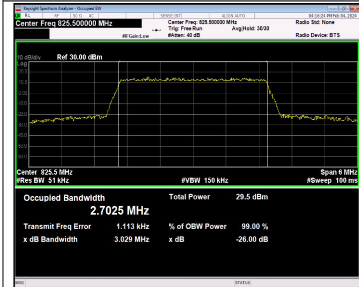
26(824-849)-3MHz-16QAM-26805-15RB#0-PASS
