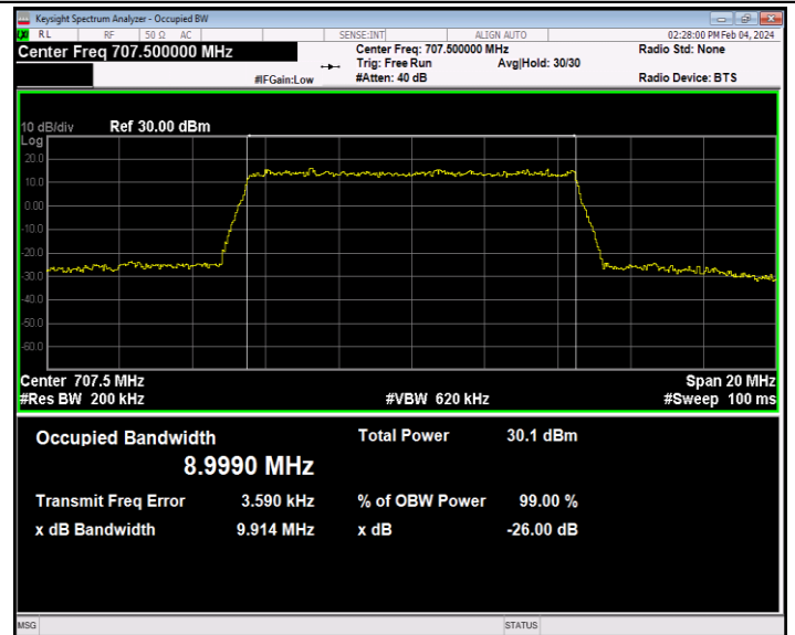
Band12-10MHz-16QAM-23095-50RB#0-PASS
