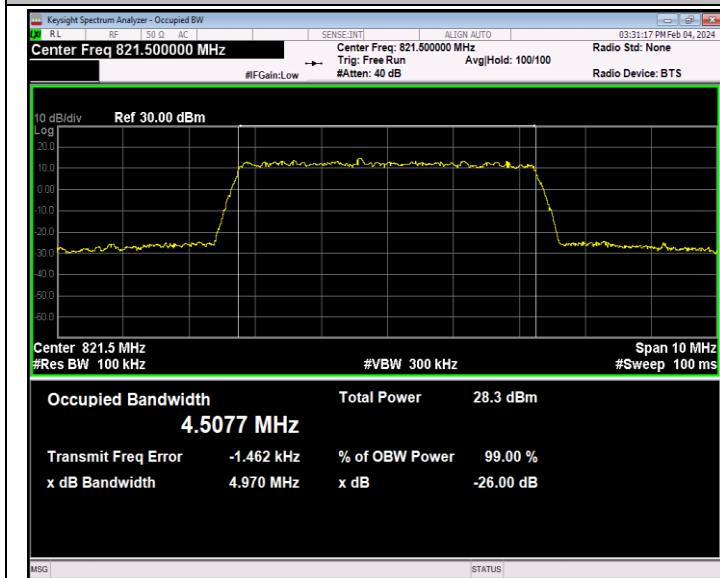
26(814-824)-5MHz-64QAM-26765-25RB#0-PASS
