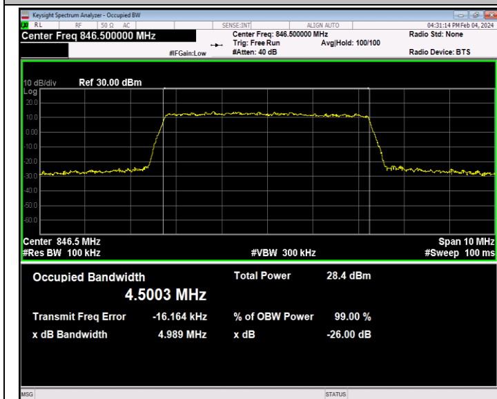
26(824-849)-5MHz-64QAM-27015-25RB#0-PASS
