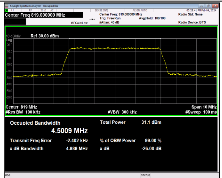
26(814-824)-5MHz-QPSK-26740-25RB#0-PASS
