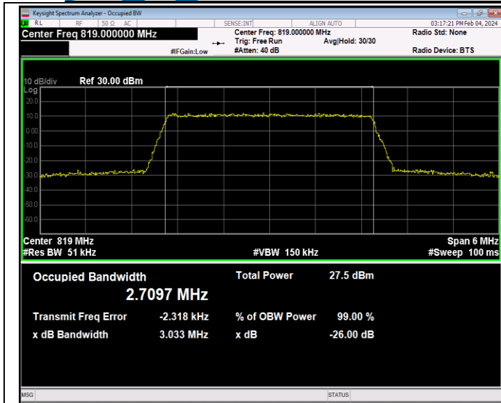
26(814-824)-3MHz-64QAM-26740-15RB#0-PASS
