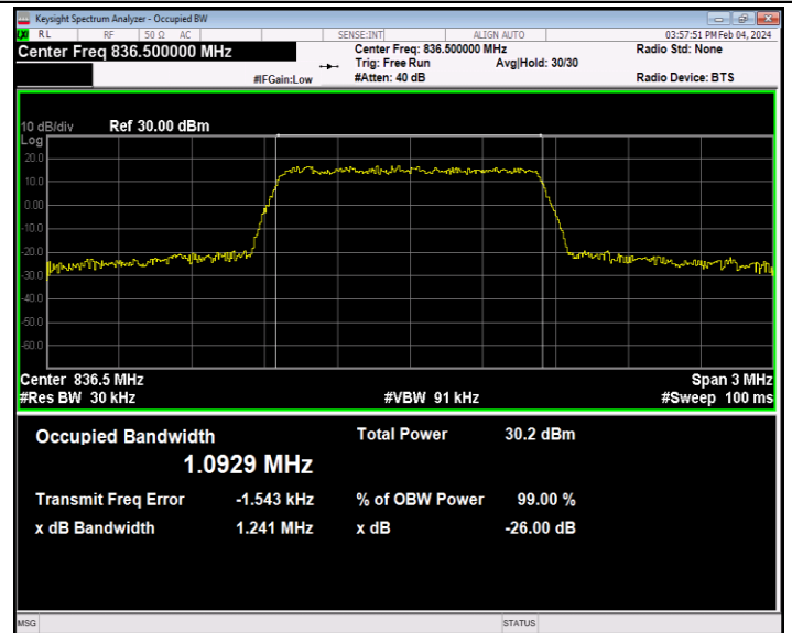
26(824-849)-1.4MHz-QPSK-26915-6RB#0-PASS
