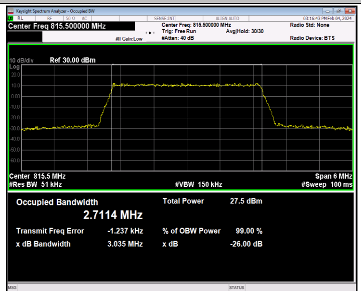
26(814-824)-3MHz-64QAM-26705-15RB#0-PASS
