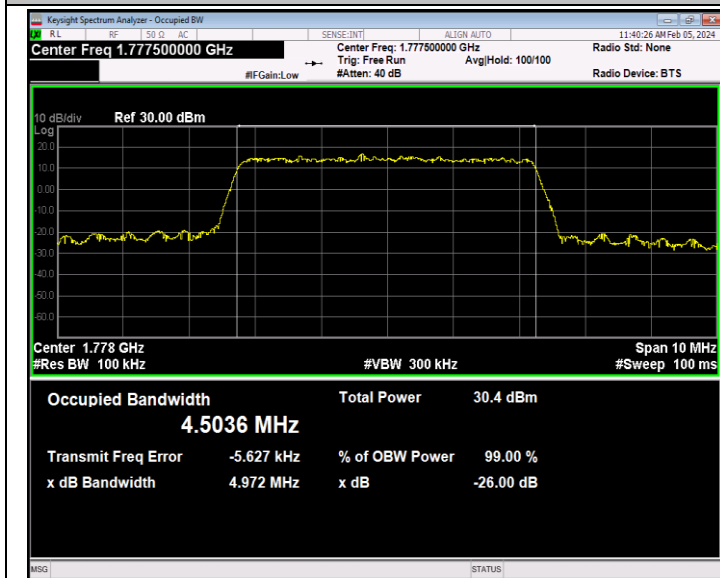
Band66-5MHz-16QAM-132647-25RB#0-PASS
