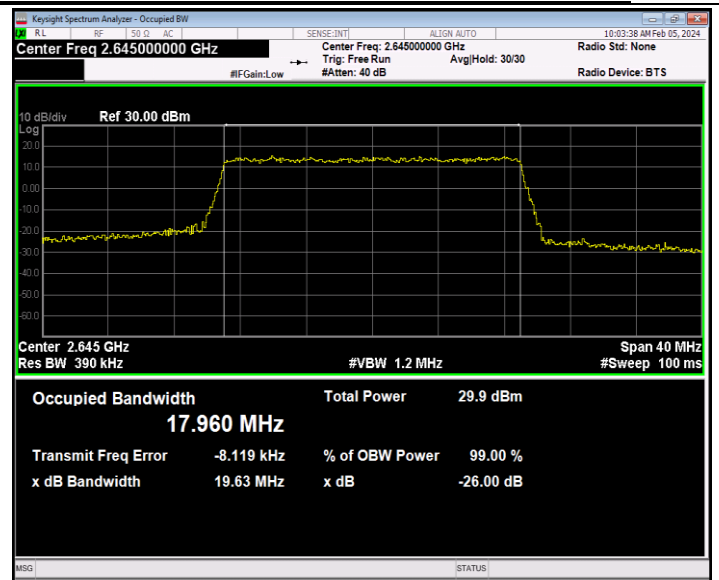
41(2535-2655)-20MHz-16QAM-41140-100RB#0-PASS
