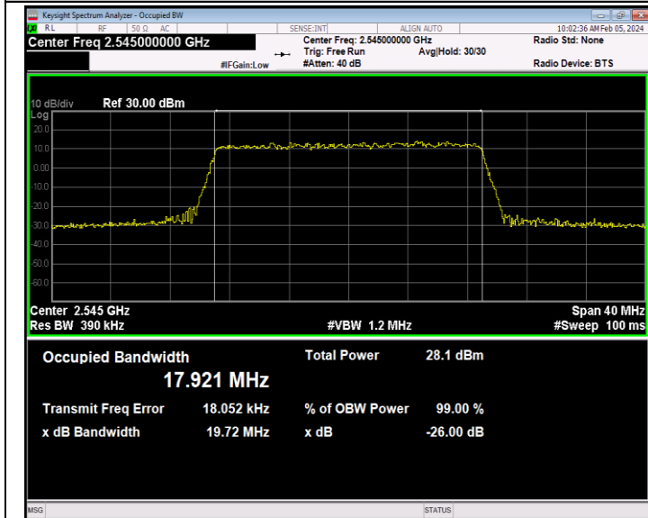
41(2535-2655)-20MHz-64QAM-40140-100RB#0-PASS
