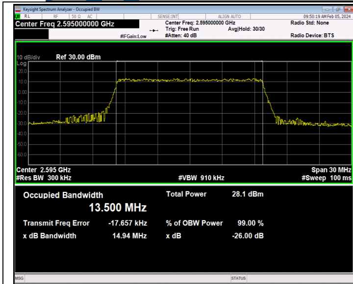
41(2535-2655)-15MHz-64QAM-40640-75RB#0-PASS
