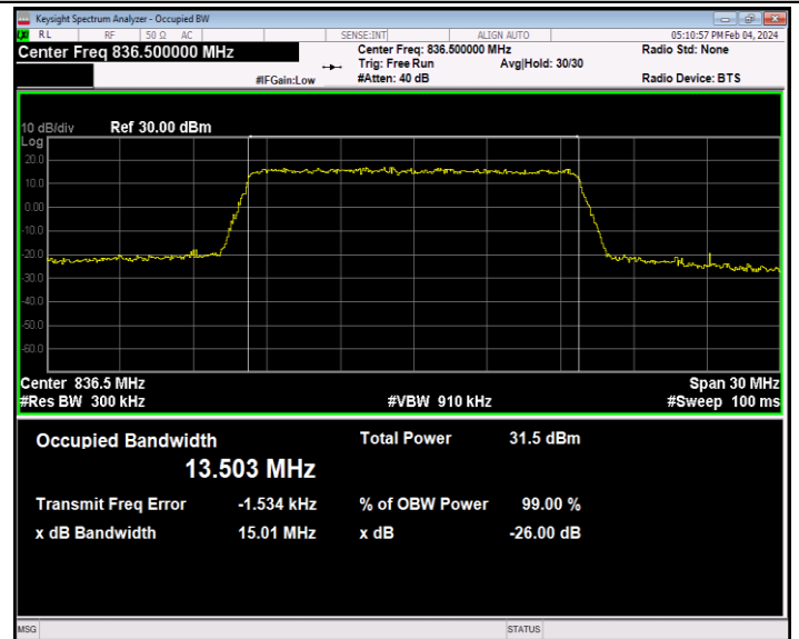
26(824-849)-15MHz-QPSK-26915-75RB#0-PASS
