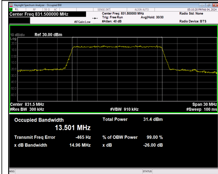
26(824-849)-15MHz-QPSK-26865-75RB#0-PASS
