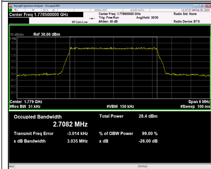
Band66-3MHz-64QAM-132657-15RB#0-PASS
