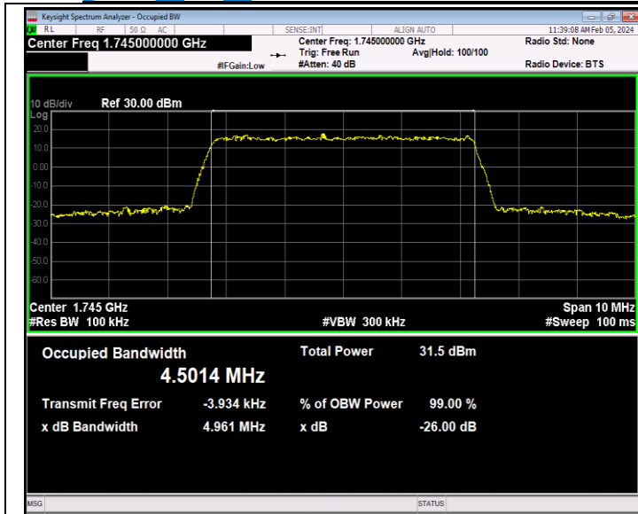
Band66-5MHz-QPSK-132322-25RB#0-PASS
