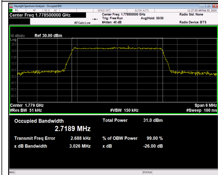
Band66-3MHz-QPSK-132657-15RB#0-PASS
