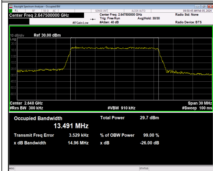
41(2535-2655)-15MHz-16QAM-41165-75RB#0-PASS
