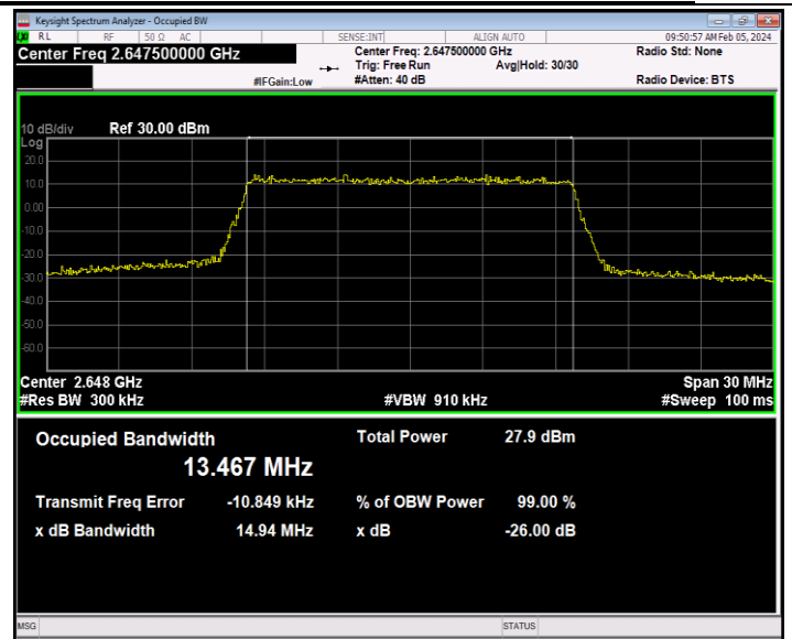
41(2535-2655)-15MHz-64QAM-41165-75RB#0-PASS
