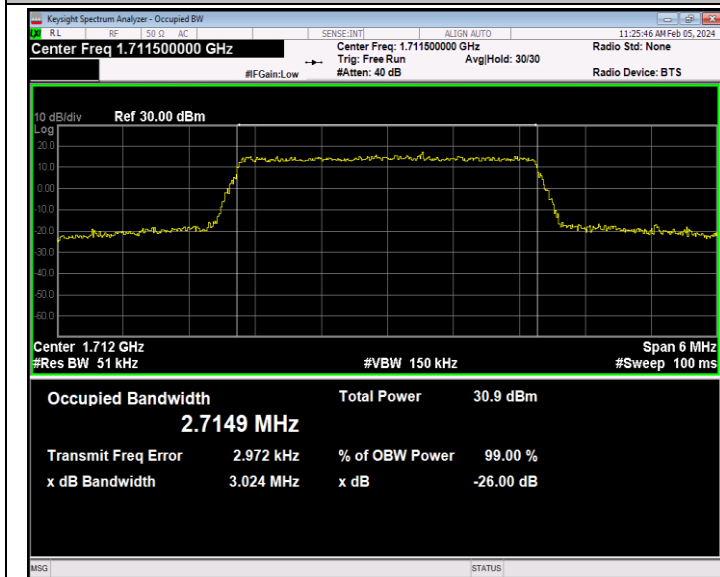
Band66-3MHz-QPSK-131987-15RB#0-PASS
