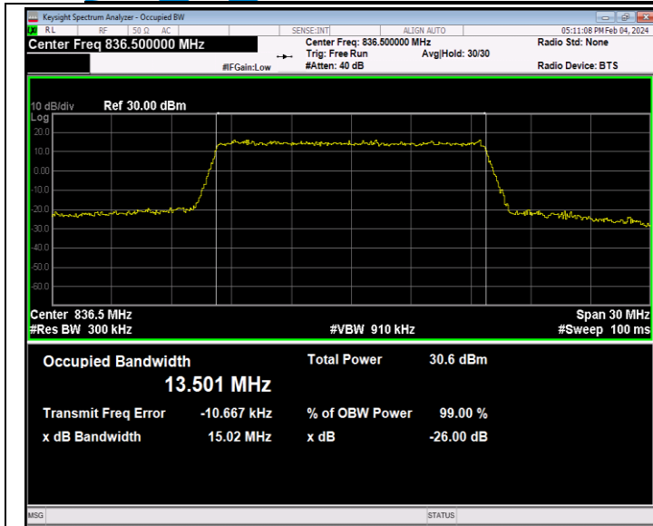
26(824-849)-15MHz-16QAM-26915-75RB#0-PASS
