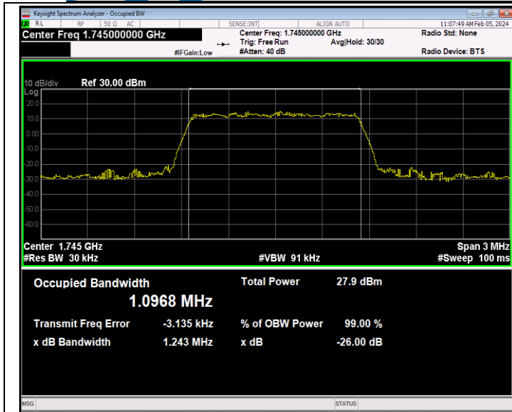
Band66-1.4MHz-64QAM-132322-6RB#0-PASS
