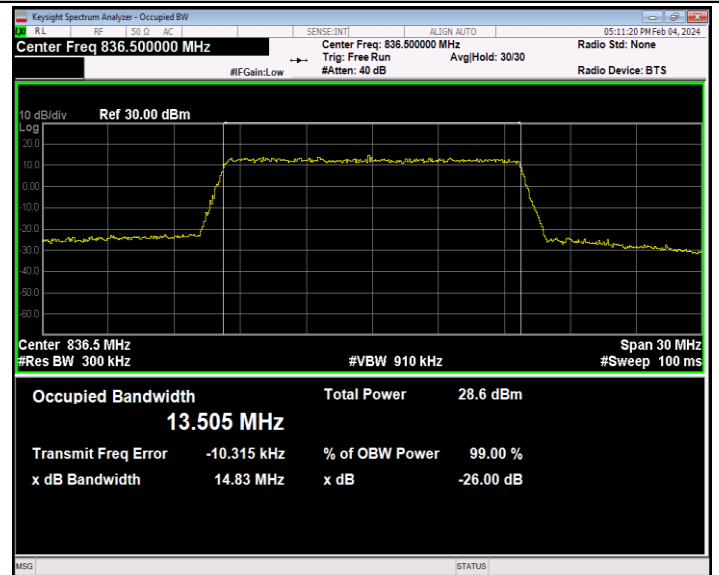
26(824-849)-15MHz-64QAM-26915-75RB#0-PASS
