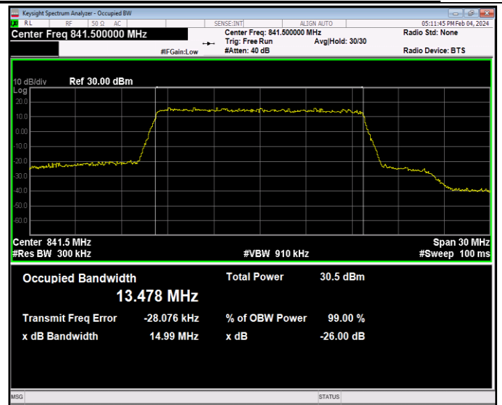
26(824-849)-15MHz-16QAM-26965-75RB#0-PASS
