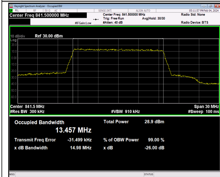
26(824-849)-15MHz-64QAM-26965-75RB#0-PASS
