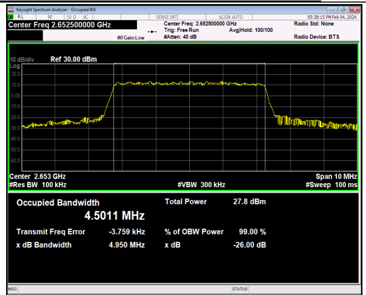
41(2535-2655)-5MHz-64QAM-41215-25RB#0-PASS
