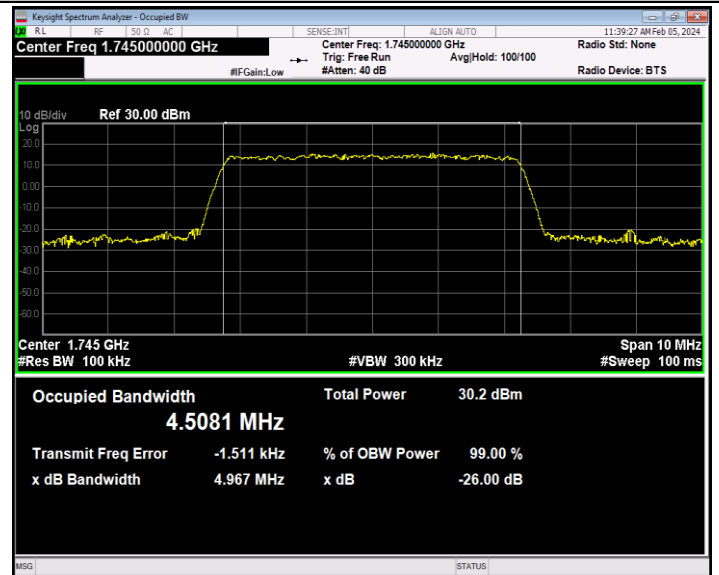
Band66-5MHz-16QAM-132322-25RB#0-PASS
