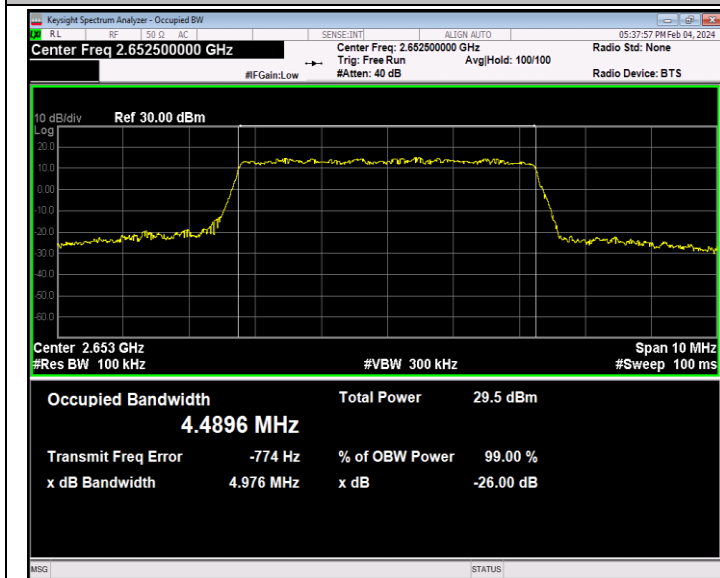
41(2535-2655)-5MHz-16QAM-41215-25RB#0-PASS
