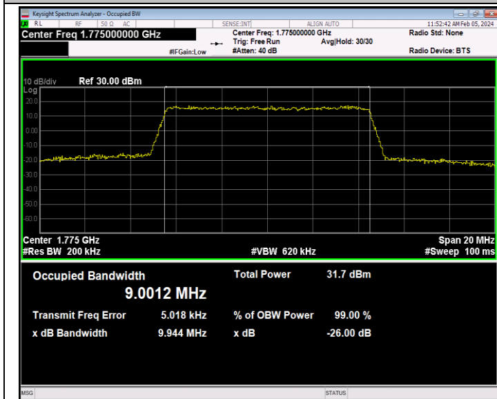
Band66-10MHz-QPSK-132622-50RB#0-PASS
