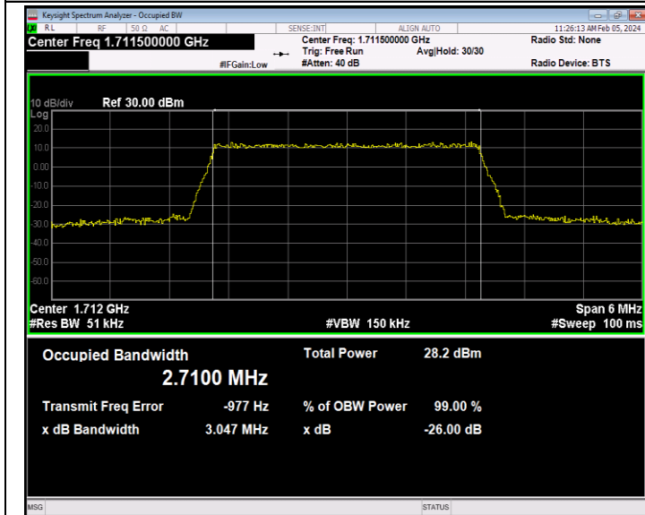
Band66-3MHz-64QAM-131987-15RB#0-PASS
