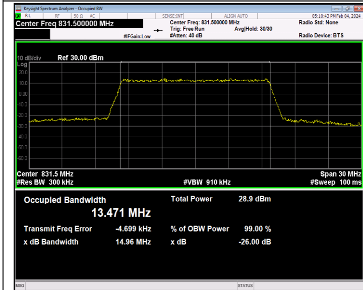
26(824-849)-15MHz-64QAM-26865-75RB#0-PASS
