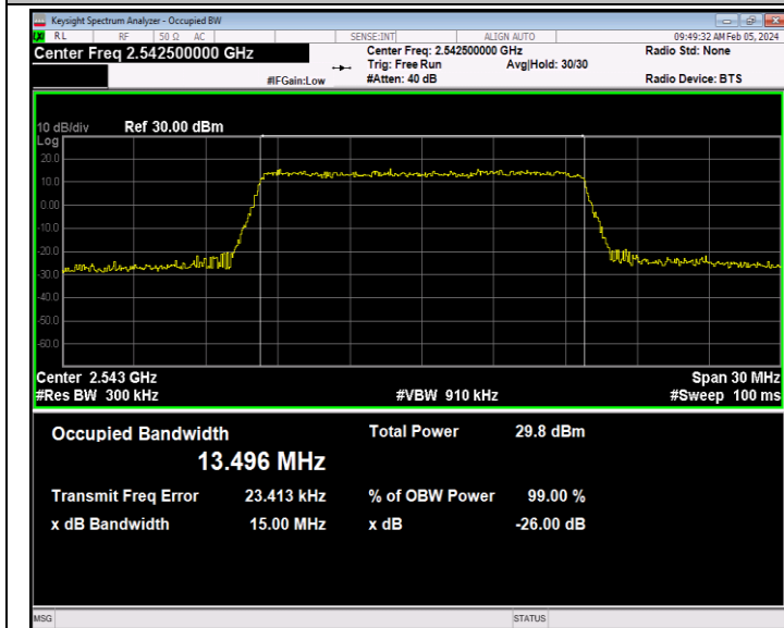
41(2535-2655)-15MHz-16QAM-40115-75RB#0-PASS
