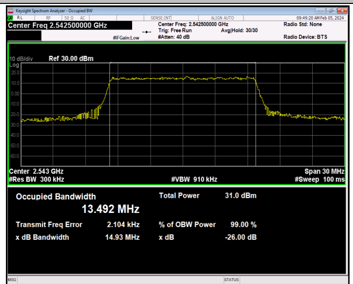
41(2535-2655)-15MHz-QPSK-40115-75RB#0-PASS
