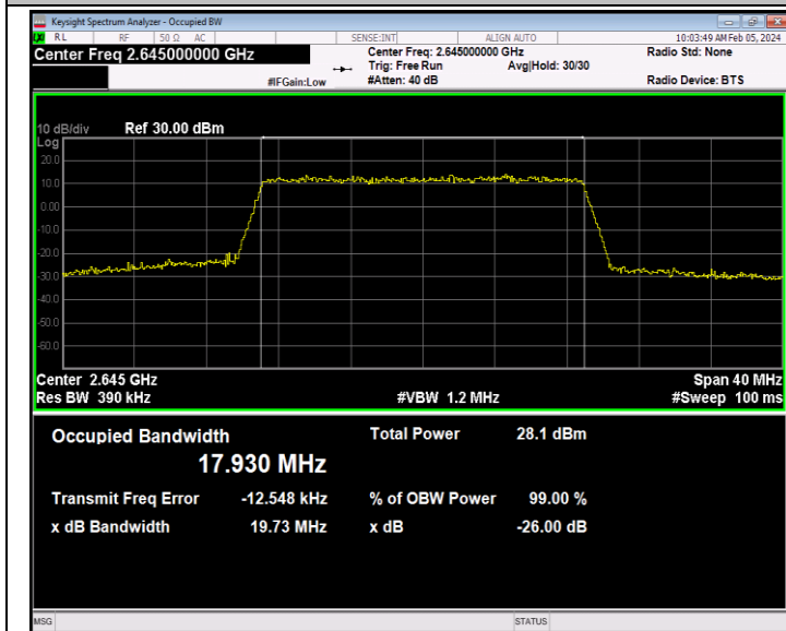
41(2535-2655)-20MHz-64QAM-41140-100RB#0-PASS
