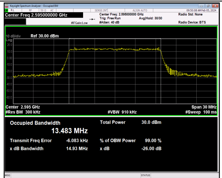
41(2535-2655)-15MHz-16QAM-40640-75RB#0-PASS
