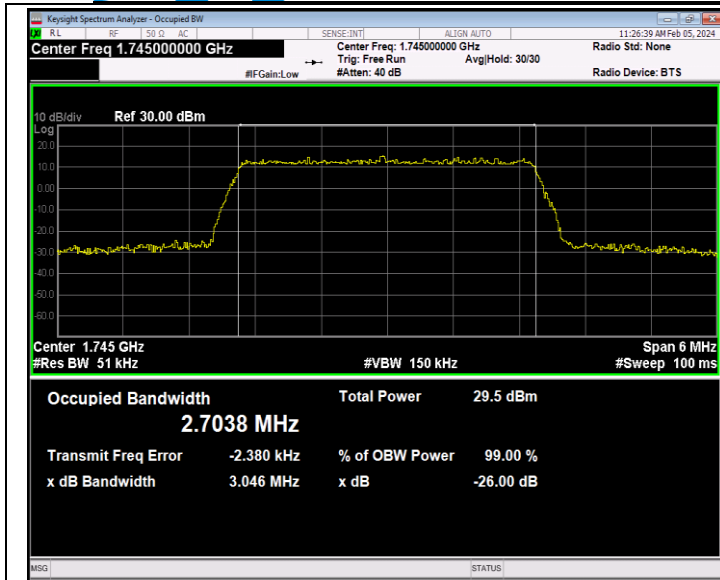
Band66-3MHz-16QAM-132322-15RB#0-PASS
