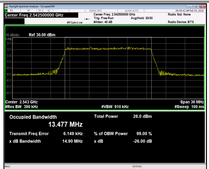
41(2535-2655)-15MHz-64QAM-40115-75RB#0-PASS
