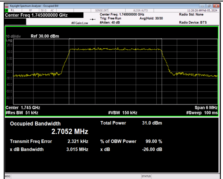
Band66-3MHz-QPSK-132322-15RB#0-PASS
