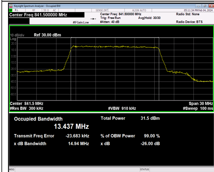
26(824-849)-15MHz-QPSK-26965-75RB#0-PASS
