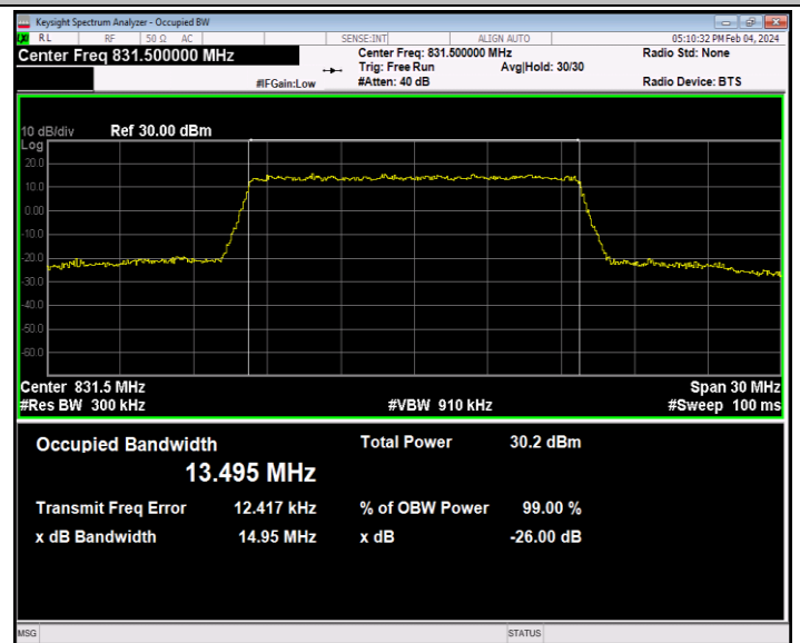
26(824-849)-15MHz-16QAM-26865-75RB#0-PASS
