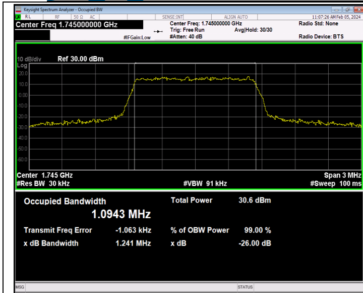
Band66-1.4MHz-QPSK-132322-6RB#0-PASS
