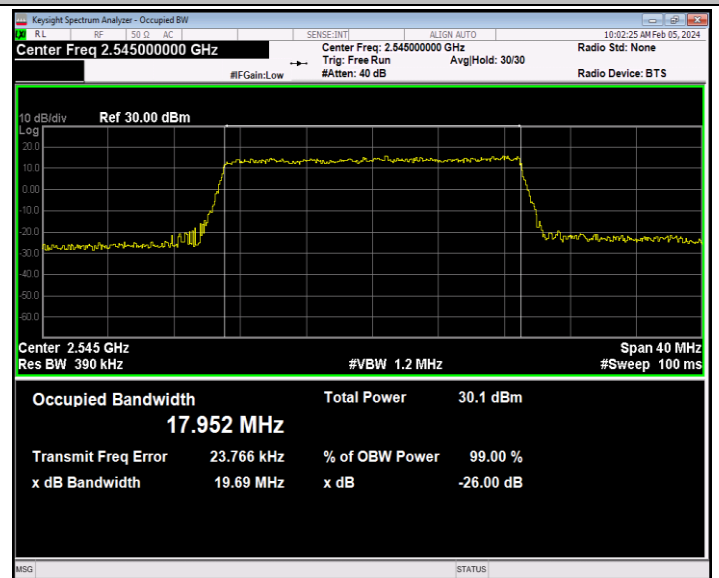
41(2535-2655)-20MHz-16QAM-40140-100RB#0-PASS
