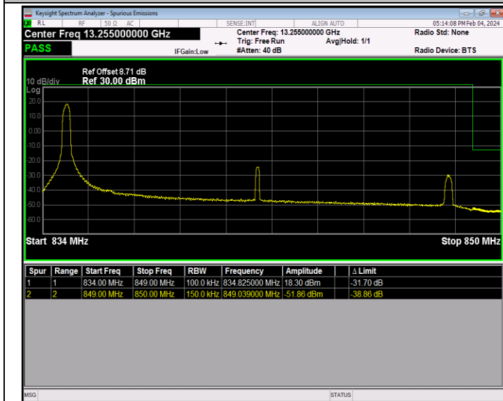
Band26_15MHz_QPSK_26965_1RB#0
