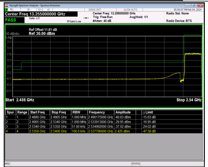
Band41_5MHz_16QAM_40065_25RB#0
