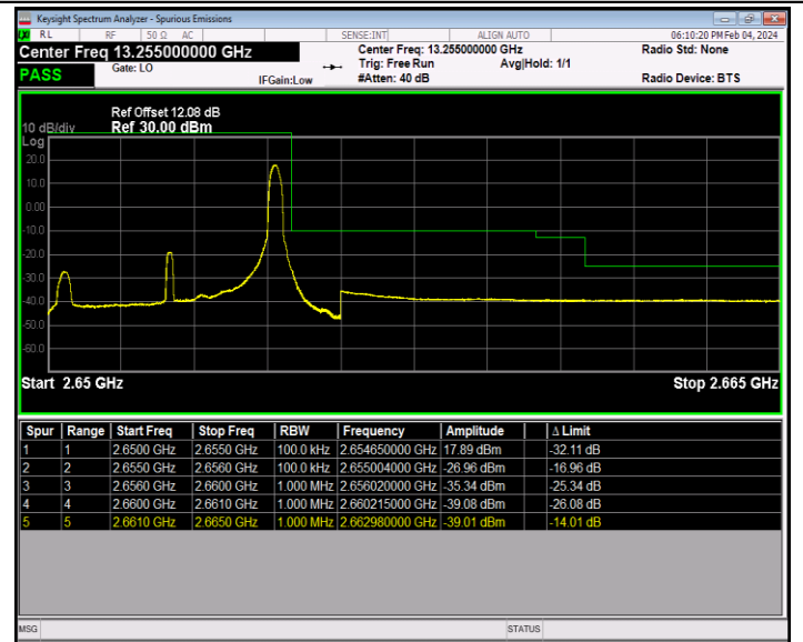
Band41_5MHz_64QAM_41215_1RB#24
