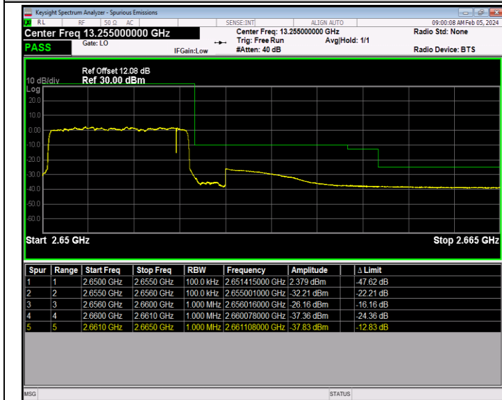
Band41_5MHz_16QAM_41215_25RB#0
