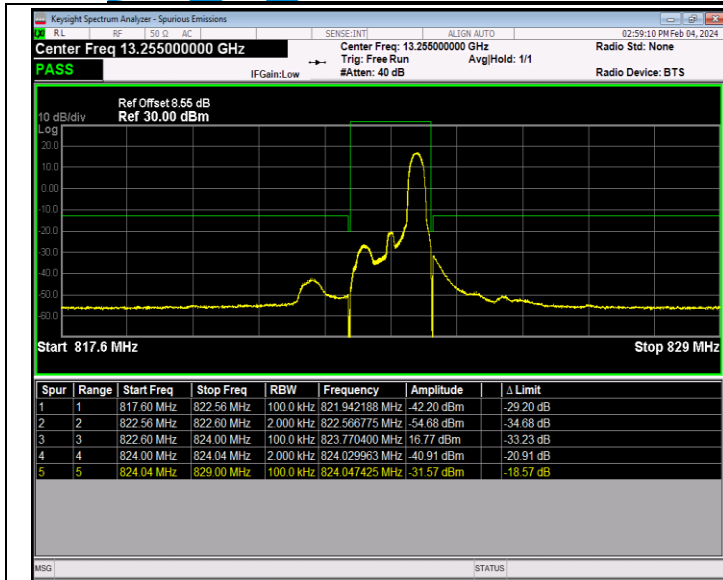
Band26_1.4MHz_64QAM_26783_1RB#5
