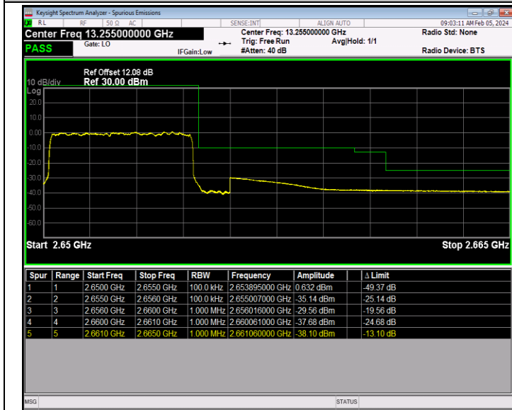
Band41_5MHz_64QAM_41215_25RB#0
