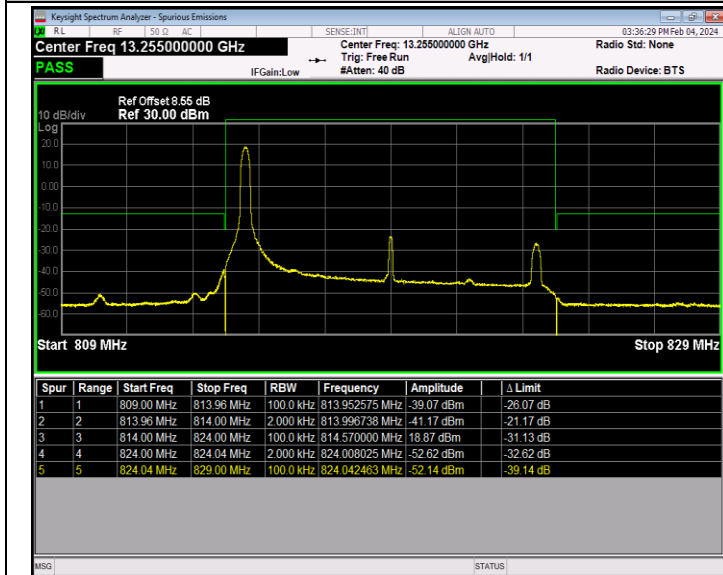
Band26_10MHz_QPSK_26740_1RB#0
