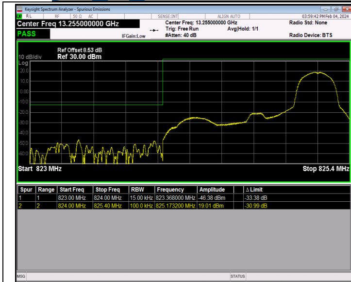
Band26_1.4MHz_QPSK_26797_1RB#5
