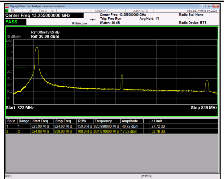
Band26_15MHz_16QAM_26865_1RB#0
