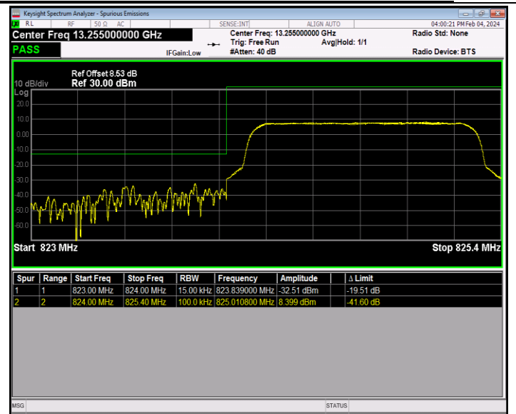
Band26_1.4MHz_16QAM_26797_6RB#0
