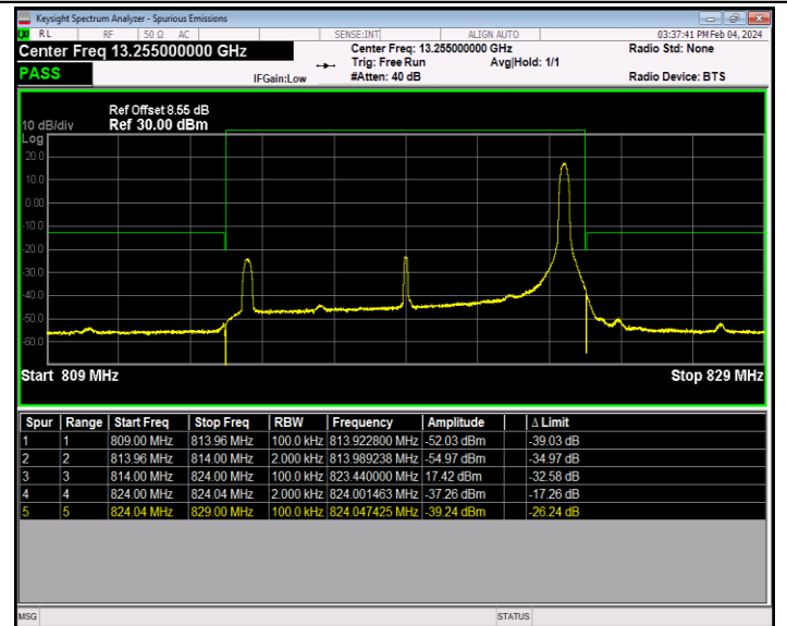
Band26_10MHz_64QAM_26740_1RB#49
