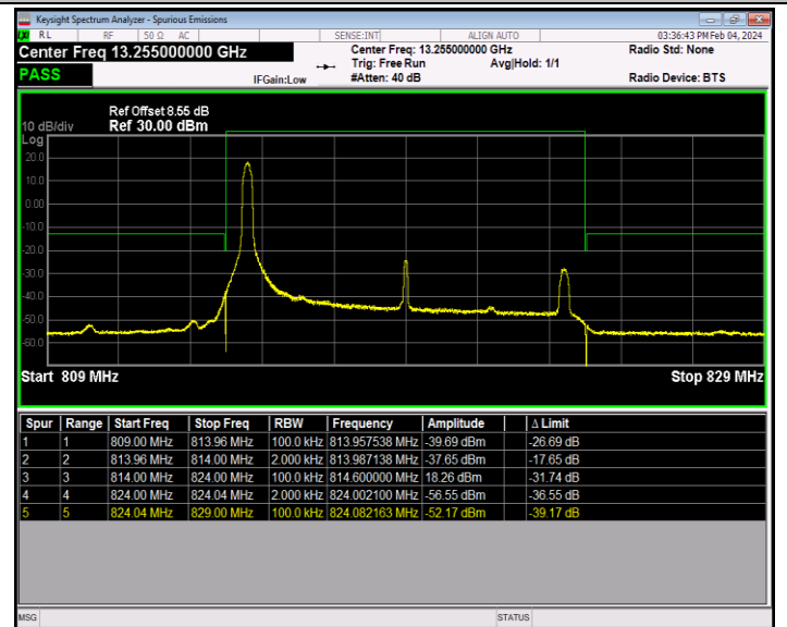
Band26_10MHz_16QAM_26740_1RB#0
