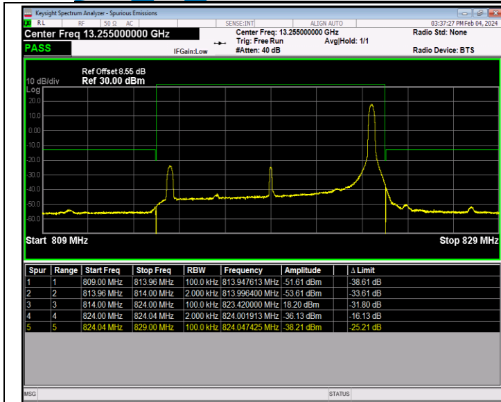
Band26_10MHz_16QAM_26740_1RB#49
