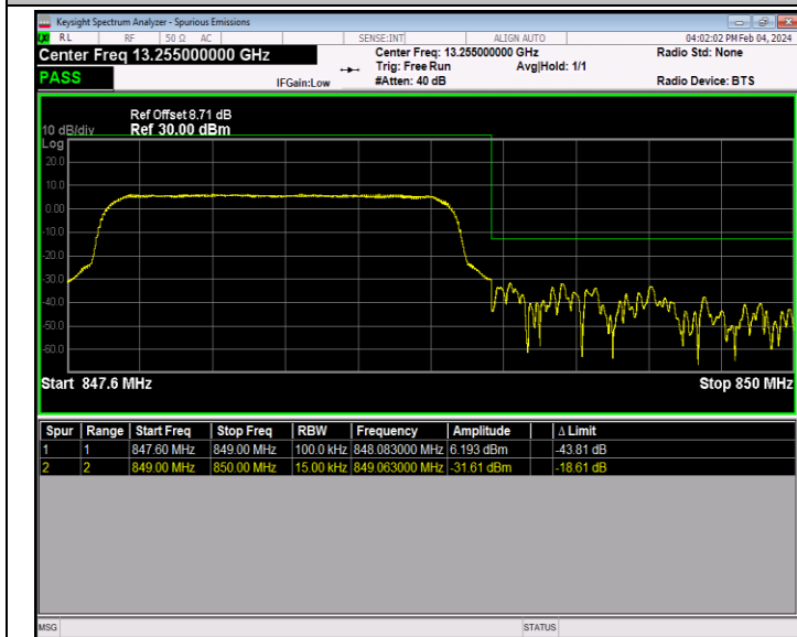
Band26_1.4MHz_64QAM_27033_6RB#0
