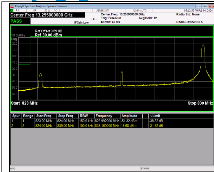
Band26_15MHz_QPSK_26865_1RB#74
