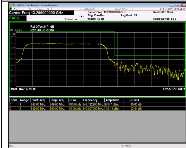
Band26_1.4MHz_QPSK_27033_6RB#0
