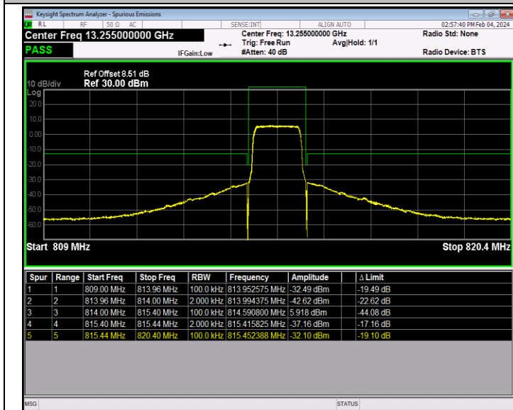
Band26_1.4MHz_64QAM_26697_6RB#0
