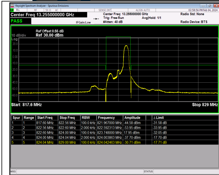
Band26_1.4MHz_16QAM_26783_1RB#5
