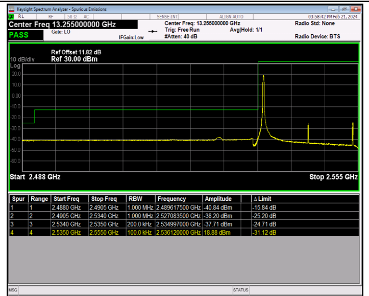
Band41_20MHz_QPSK_40140_1RB#0
