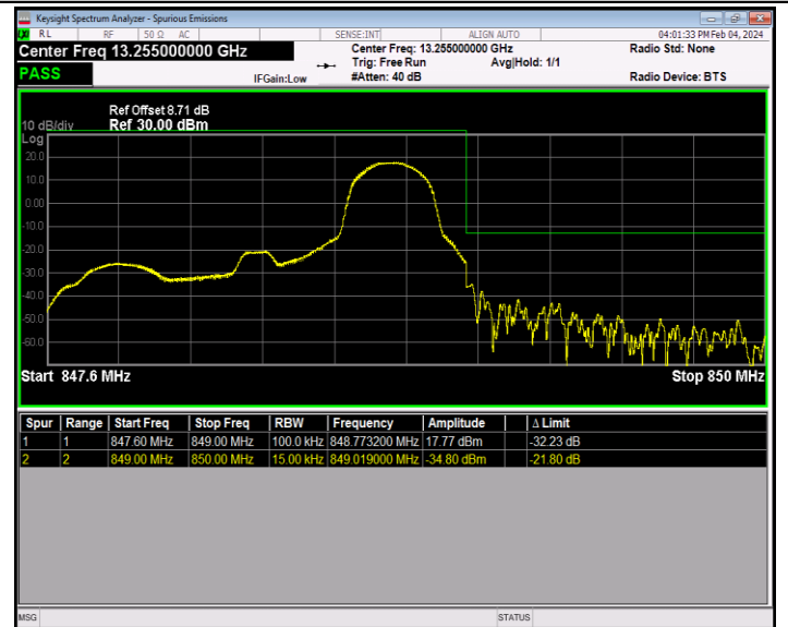
Band26_1.4MHz_64QAM_27033_1RB#5
