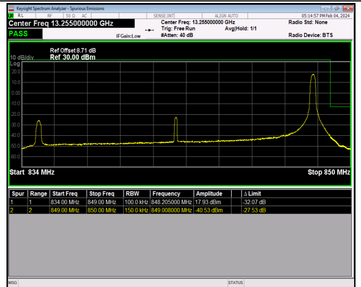
Band26_15MHz_16QAM_26965_1RB#74
