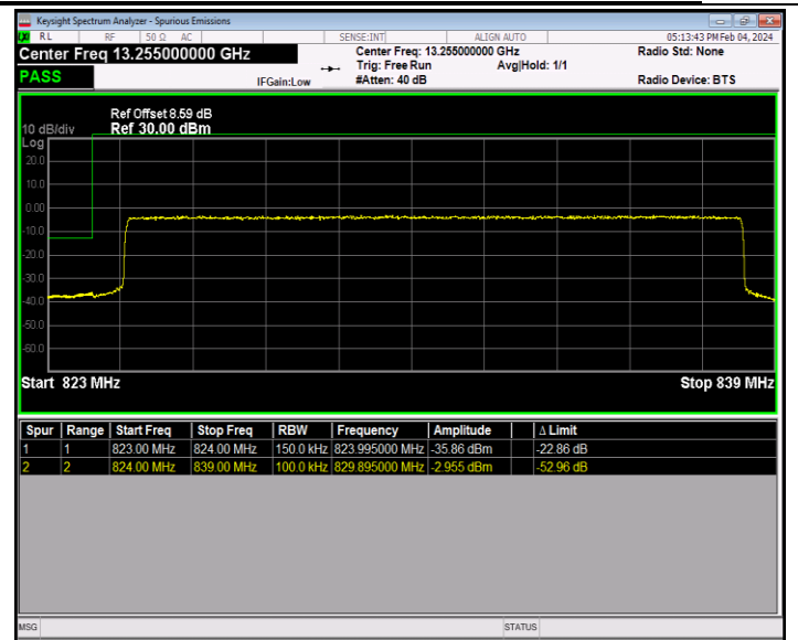
Band26_15MHz_16QAM_26865_75RB#0
