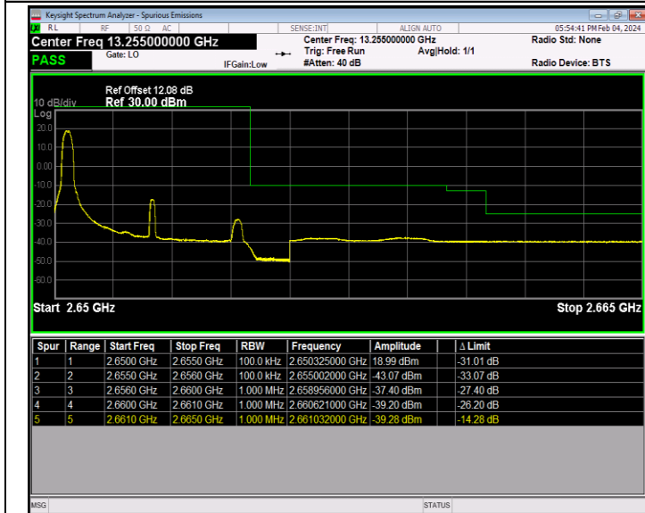
Band41_5MHz_QPSK_41215_1RB#0
