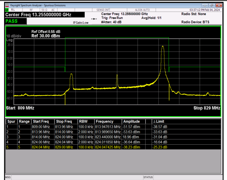
Band26_10MHz_QPSK_26740_1RB#49
