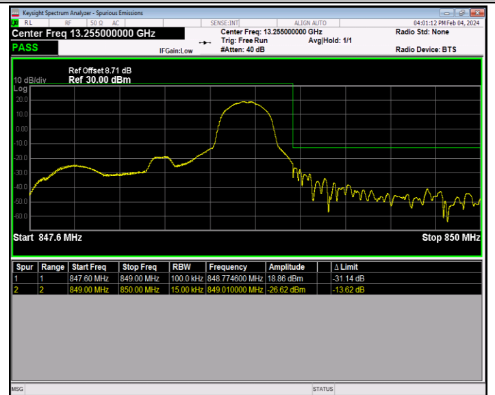
Band26_1.4MHz_QPSK_27033_1RB#5
