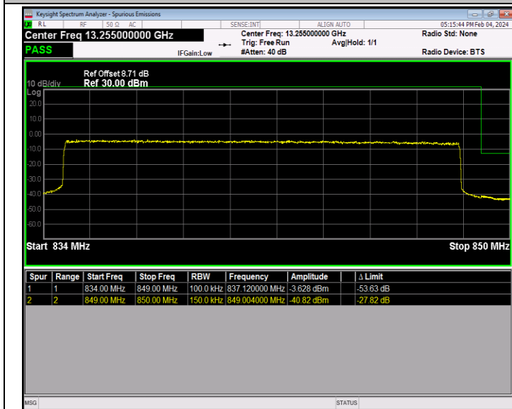
Band26_15MHz_64QAM_26965_75RB#0
