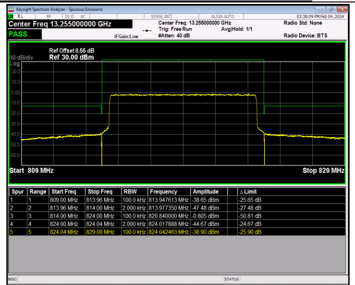
Band26_10MHz_16QAM_26740_50RB#0
