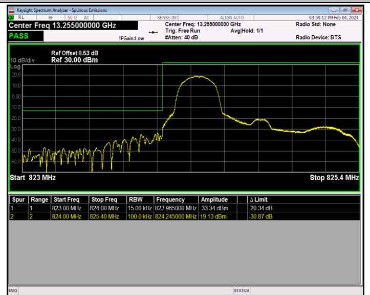
Band26_1.4MHz_QPSK_26797_1RB#0
