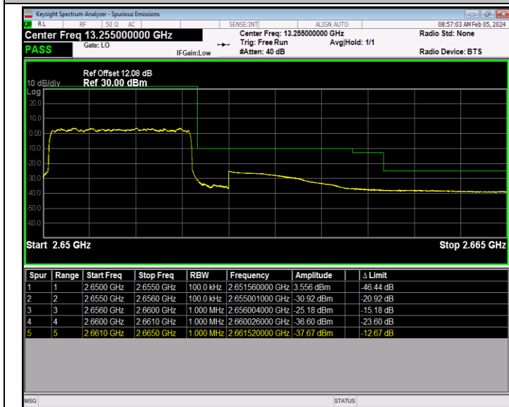
Band41_5MHz_QPSK_41215_25RB#0
