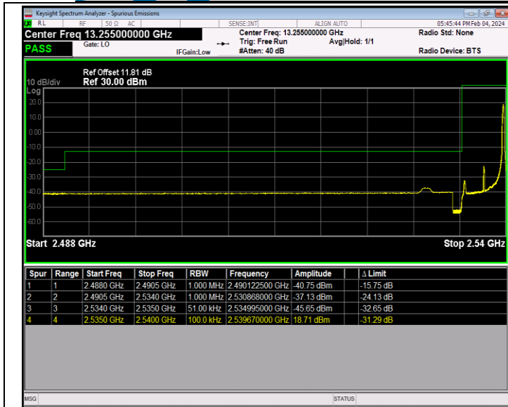
Band41_5MHz_16QAM_40065_1RB#24
