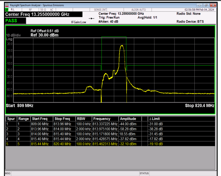
Band26_1.4MHz_64QAM_26697_1RB#5
