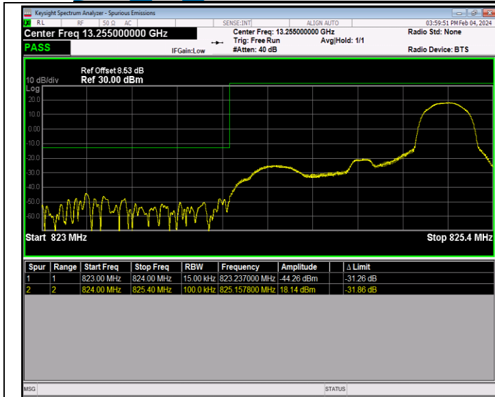
Band26_1.4MHz_16QAM_26797_1RB#5
