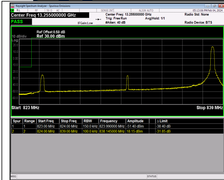
Band26_15MHz_16QAM_26865_1RB#74
