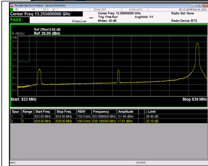
Band26_15MHz_64QAM_26865_1RB#74
