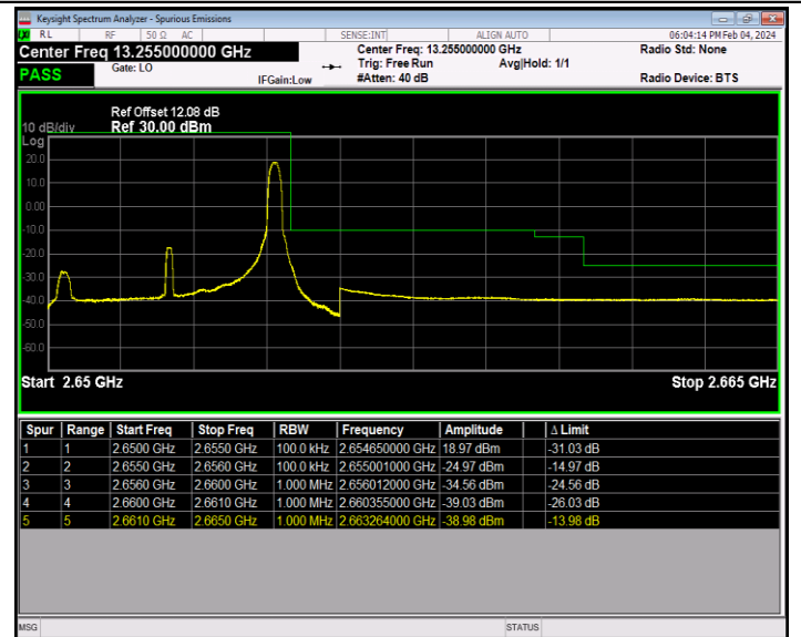
Band41_5MHz_QPSK_41215_1RB#24
