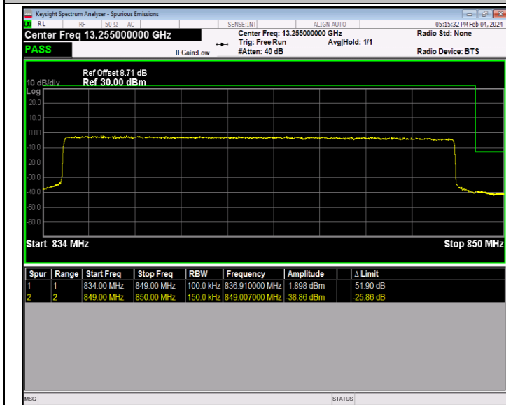
Band26_15MHz_16QAM_26965_75RB#0
