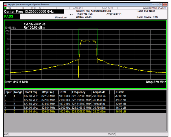
Band26_1.4MHz_16QAM_26783_6RB#0
