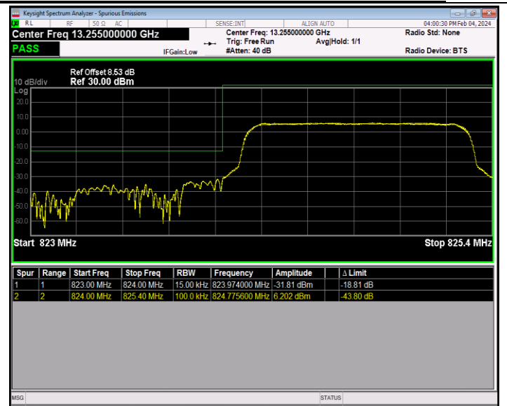
Band26_1.4MHz_64QAM_26797_6RB#0
