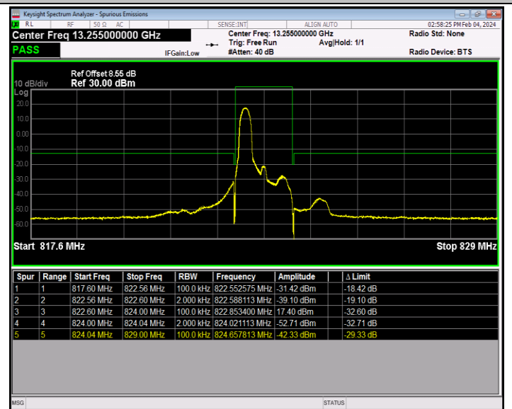
Band26_1.4MHz_64QAM_26783_1RB#0
