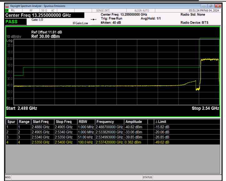
Band41_5MHz_64QAM_40065_25RB#0
