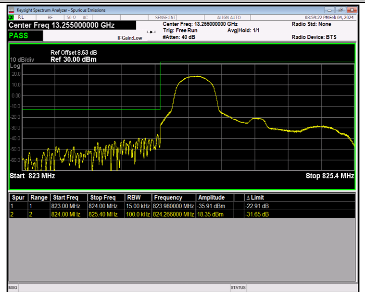
Band26_1.4MHz_16QAM_26797_1RB#0
