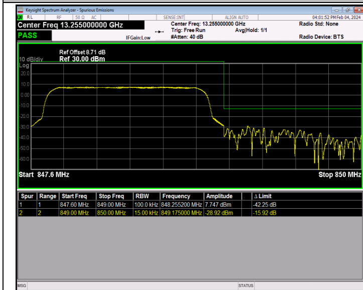
Band26_1.4MHz_16QAM_27033_6RB#0
