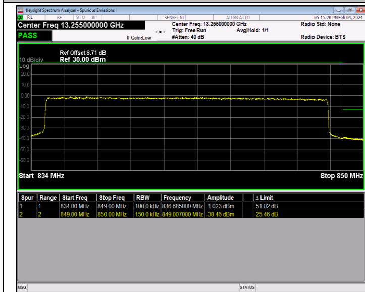
Band26_15MHz_QPSK_26965_75RB#0
