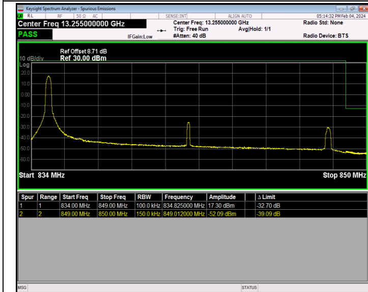
Band26_15MHz_64QAM_26965_1RB#0
