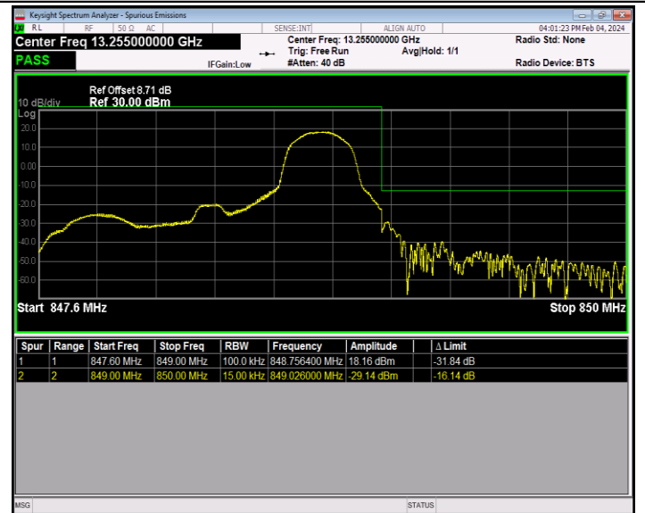
Band26_1.4MHz_16QAM_27033_1RB#5
