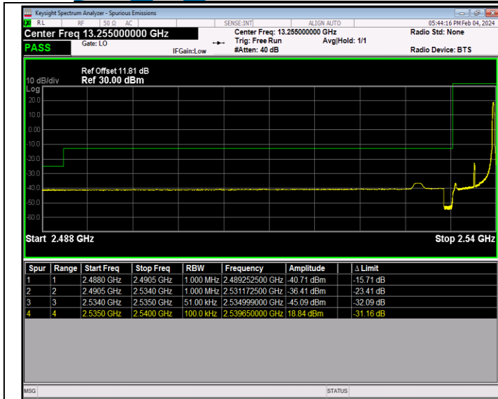
Band41_5MHz_QPSK_40065_1RB#24
