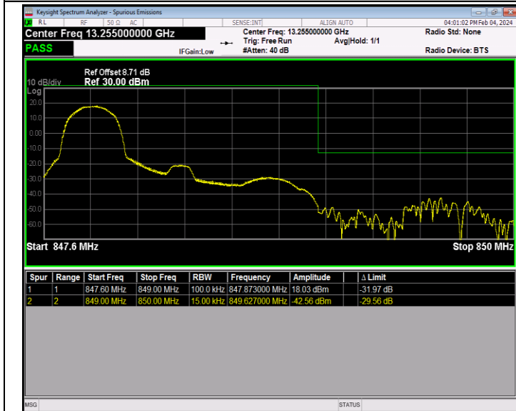
Band26_1.4MHz_64QAM_27033_1RB#0
