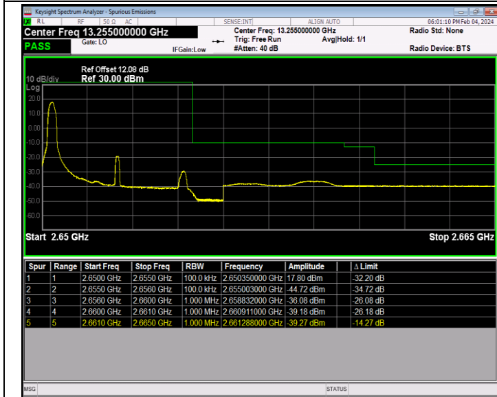
Band41_5MHz_64QAM_41215_1RB#0
