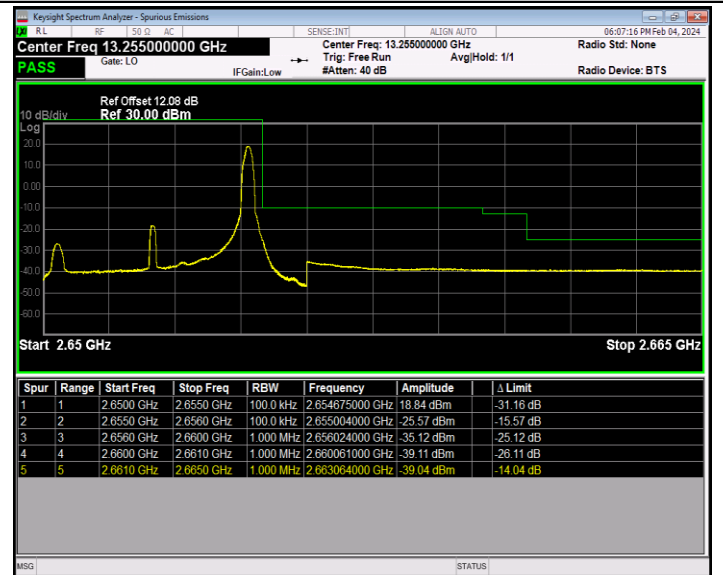
Band41_5MHz_16QAM_41215_1RB#24
