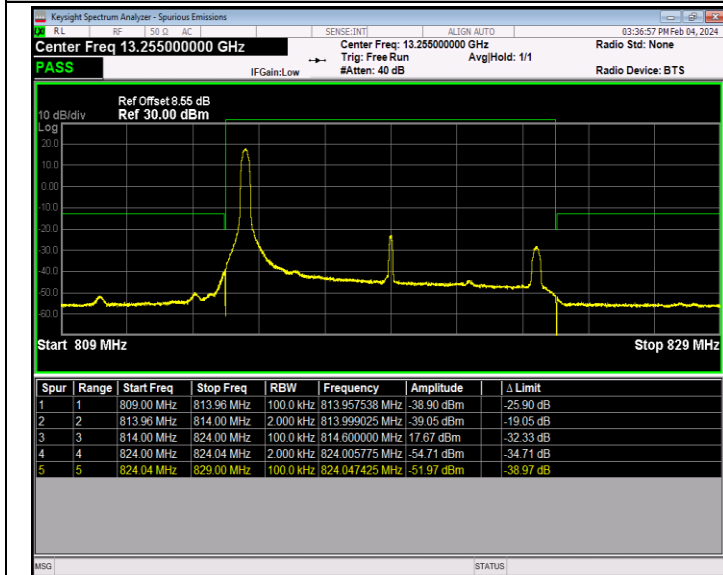
Band26_10MHz_64QAM_26740_1RB#0
