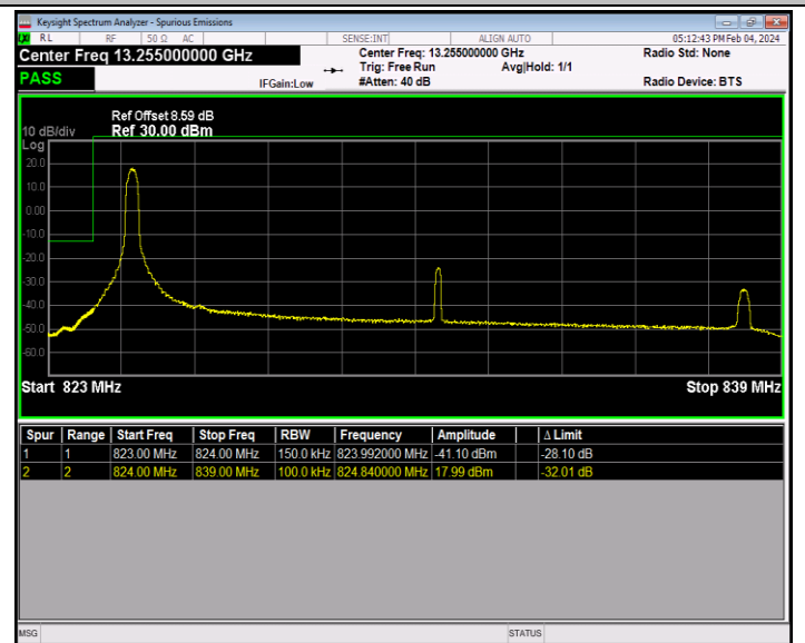
Band26_15MHz_64QAM_26865_1RB#0
