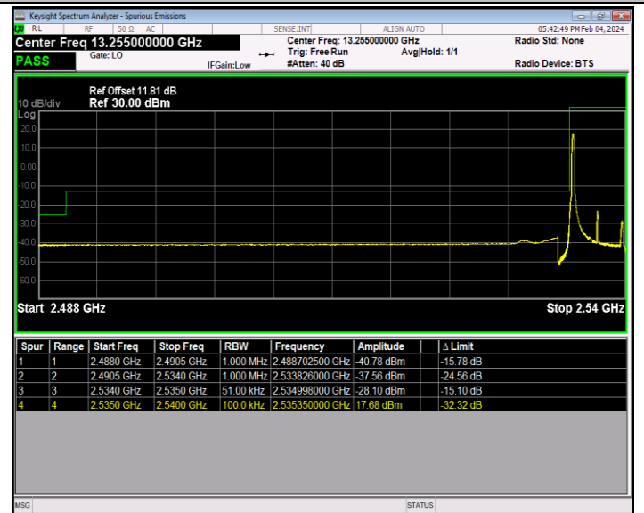
Band41_5MHz_64QAM_40065_1RB#0
