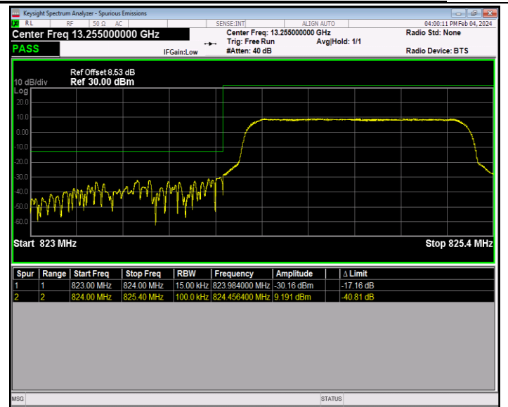
Band26_1.4MHz_QPSK_26797_6RB#0
