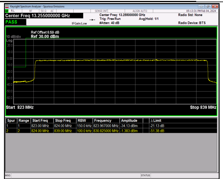
Band26_15MHz_QPSK_26865_75RB#0
