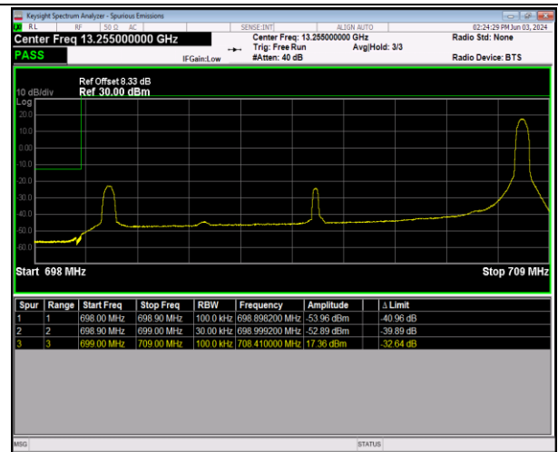
Band12_10MHz_64QAM_23060_1RB#49
