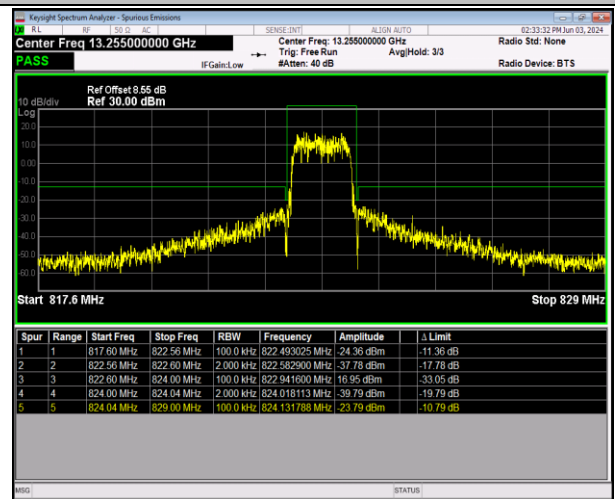
Band26_1.4MHz_16QAM_26783_6RB#0
