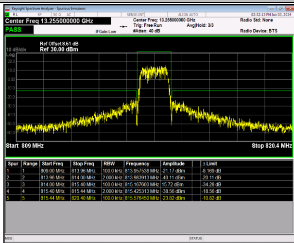
Band26_1.4MHz_16QAM_26697_6RB#0
