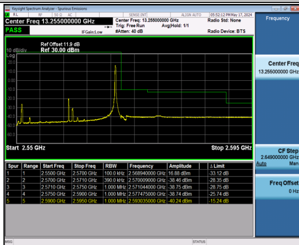
Band7_20MHz_64QAM_21350_1RB#99
