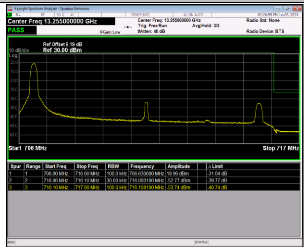
Band12_10MHz_QPSK_23130_1RB#0
