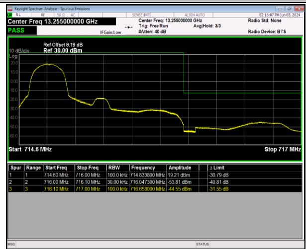
Band12_1.4MHz_QPSK_23173_1RB#0
