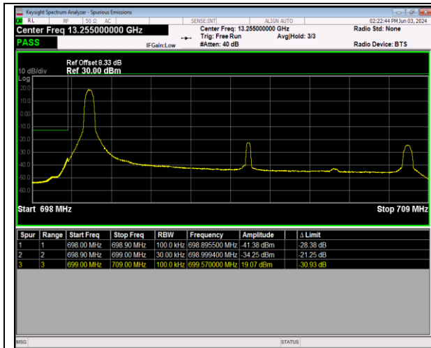
Band12_10MHz_16QAM_23060_1RB#0
