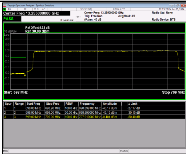
Band12_10MHz_16QAM_23060_50RB#0
