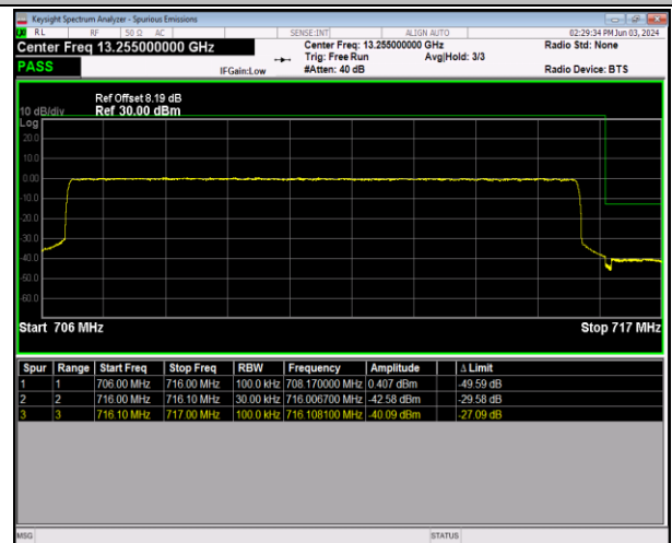
Band12_10MHz_QPSK_23130_50RB#0
