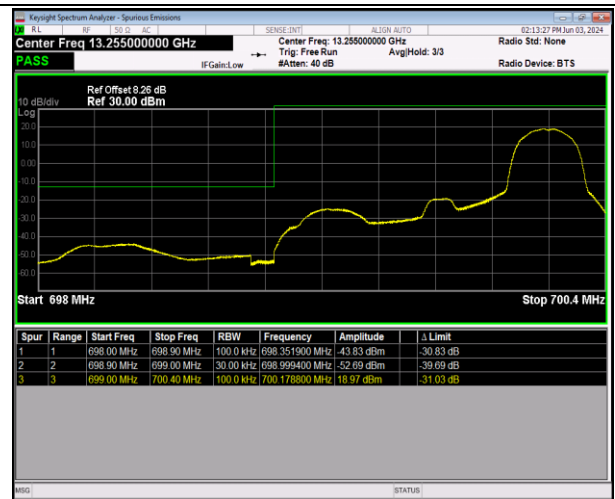
Band12_1.4MHz_QPSK_23017_1RB#5
