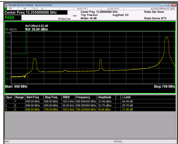
Band12_10MHz_16QAM_23060_1RB#49
