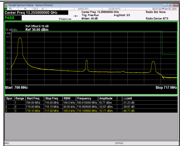
Band12_10MHz_16QAM_23130_1RB#0
