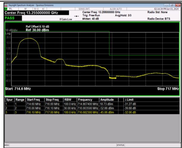
Band12_1.4MHz_16QAM_23173_1RB#0
