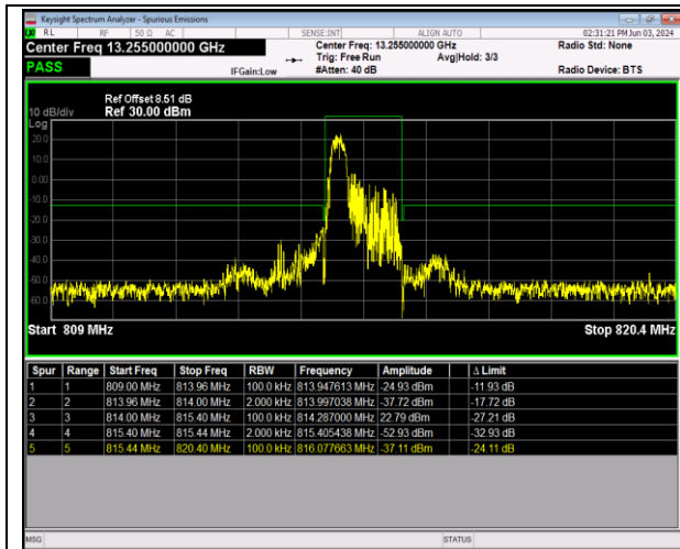
Band26_1.4MHz_16QAM_26697_1RB#0
