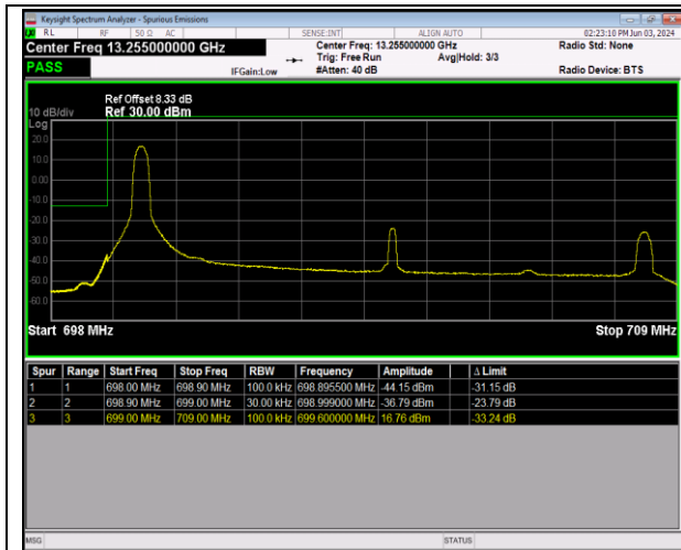
Band12_10MHz_64QAM_23060_1RB#0
