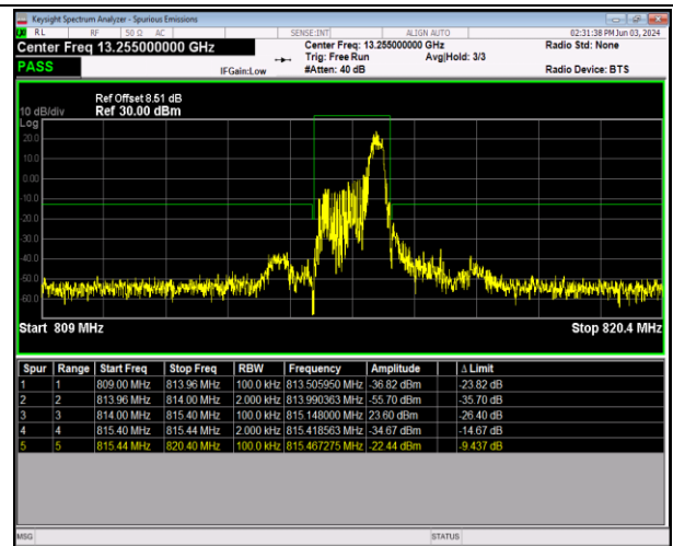
Band26_1.4MHz_QPSK_26697_1RB#5
