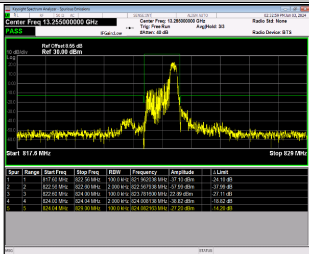
Band26_1.4MHz_QPSK_26783_1RB#5
