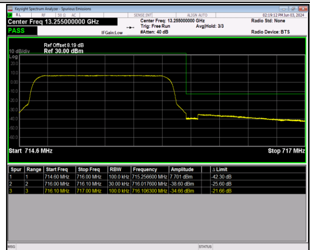
Band12_1.4MHz_16QAM_23173_6RB#0
