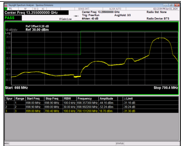
Band12_1.4MHz_16QAM_23017_1RB#5
