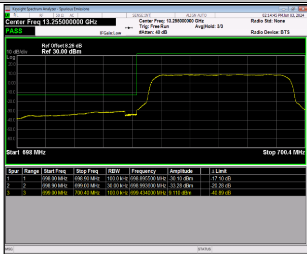
Band12_1.4MHz_QPSK_23017_6RB#0
