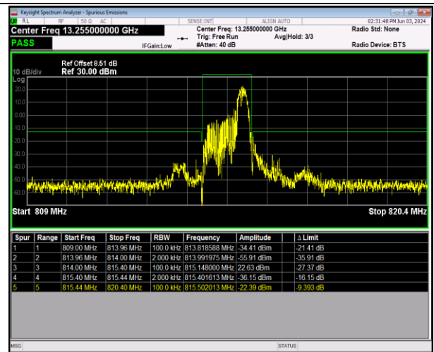
Band26_1.4MHz_16QAM_26697_1RB#5
