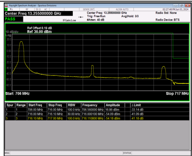
Band12_10MHz_64QAM_23130_1RB#0
