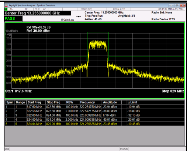
Band26_1.4MHz_QPSK_26783_6RB#0
