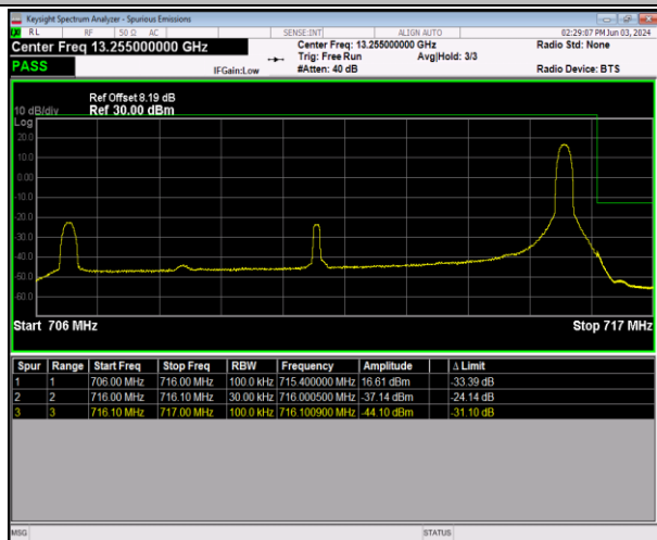
Band12_10MHz_64QAM_23130_1RB#49
