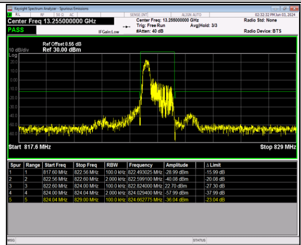
Band26_1.4MHz_QPSK_26783_1RB#0
