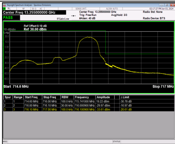
Band12_1.4MHz_QPSK_23173_1RB#5
