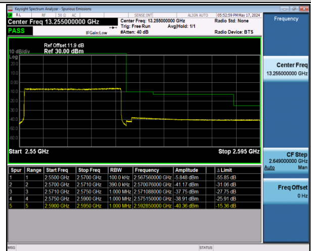
Band7_20MHz_64QAM_21350_100RB#0
