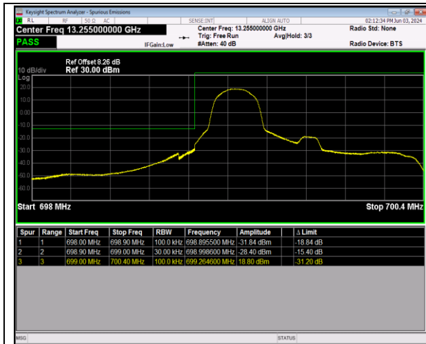
Band12_1.4MHz_16QAM_23017_1RB#0
