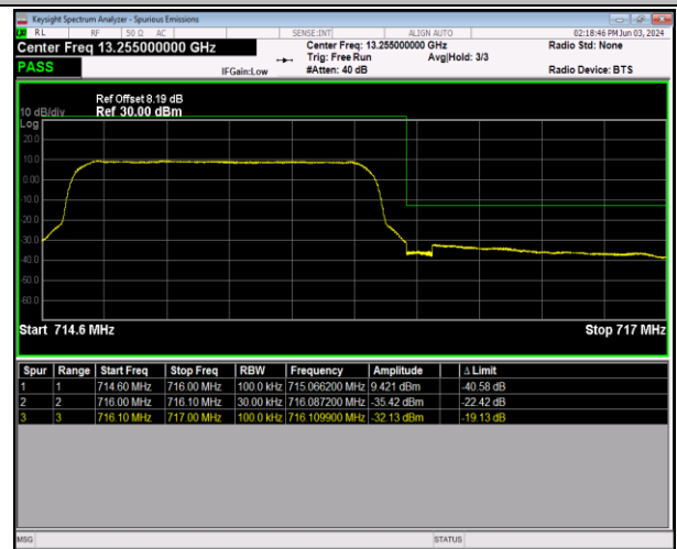
Band12_1.4MHz_QPSK_23173_6RB#0
