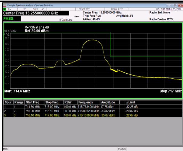
Band12_1.4MHz_64QAM_23173_1RB#5
