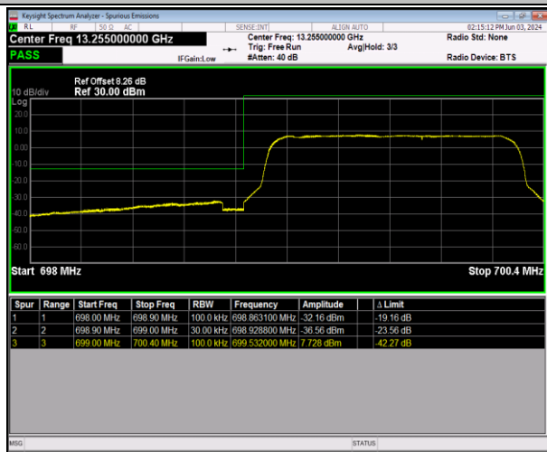
Band12_1.4MHz_16QAM_23017_6RB#0
