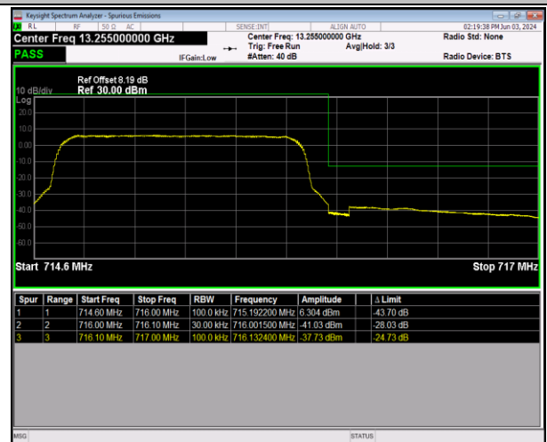
Band12_1.4MHz_64QAM_23173_6RB#0
