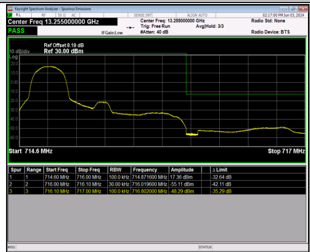
Band12_1.4MHz_64QAM_23173_1RB#0
