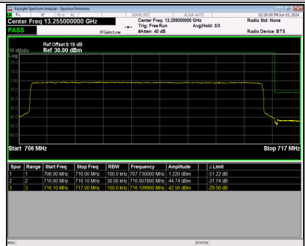
Band12_10MHz_16QAM_23130_50RB#0
