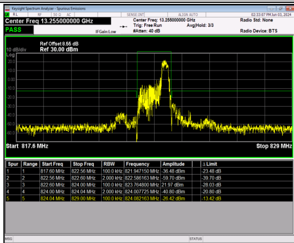
Band26_1.4MHz_16QAM_26783_1RB#5
