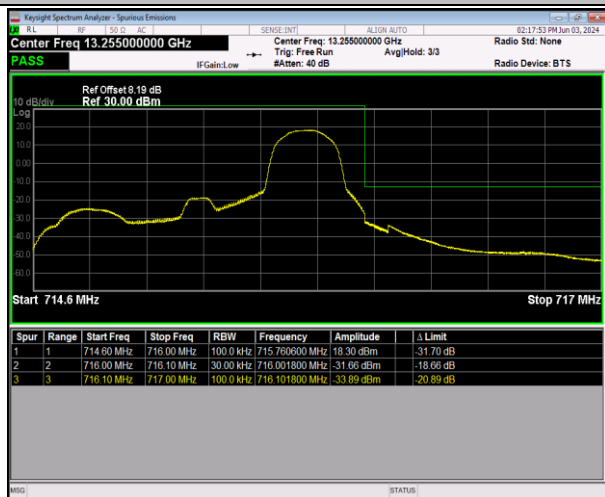
Band12_1.4MHz_16QAM_23173_1RB#5
