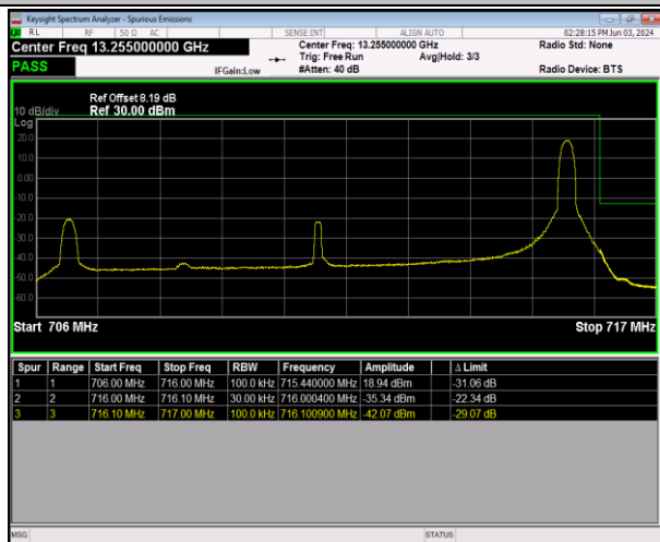
Band12_10MHz_QPSK_23130_1RB#49
