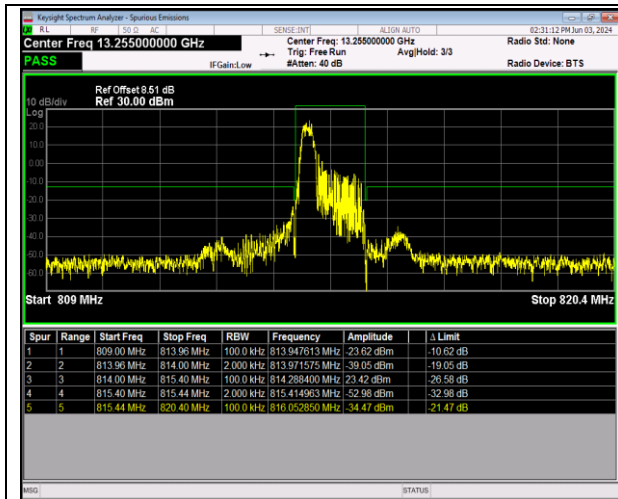
Band26_1.4MHz_QPSK_26697_1RB#0
