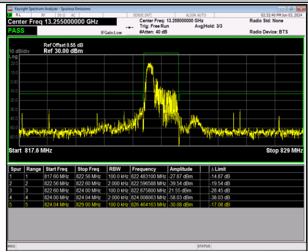
Band26_1.4MHz_16QAM_26783_1RB#0
