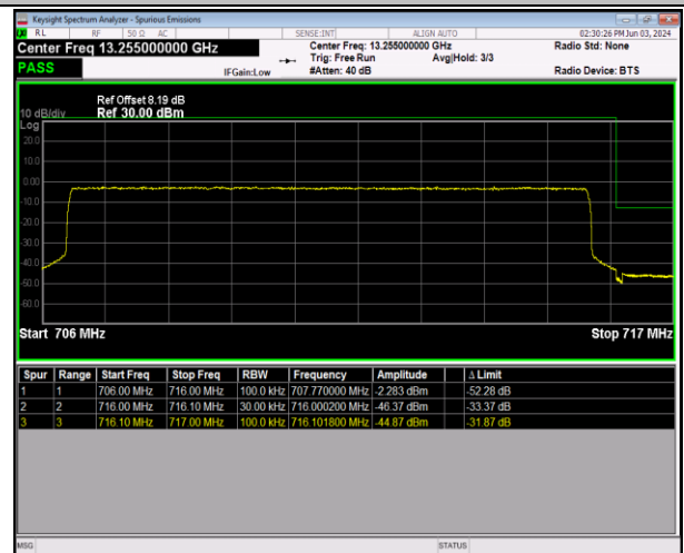
Band12_10MHz_64QAM_23130_50RB#0
