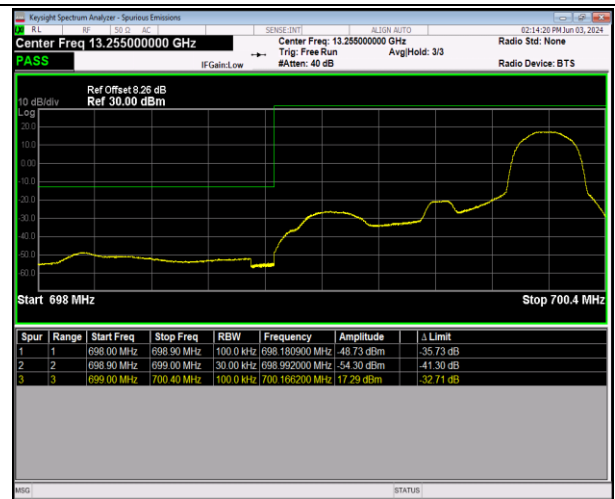
Band12_1.4MHz_64QAM_23017_1RB#5
