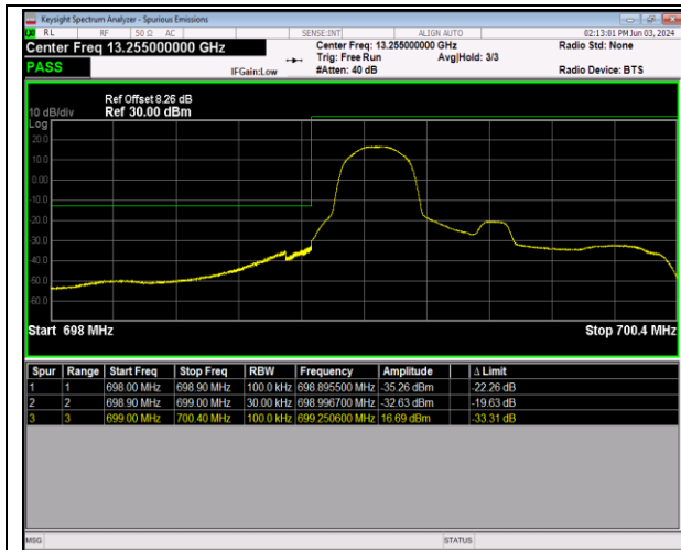
Band12_1.4MHz_64QAM_23017_1RB#0
