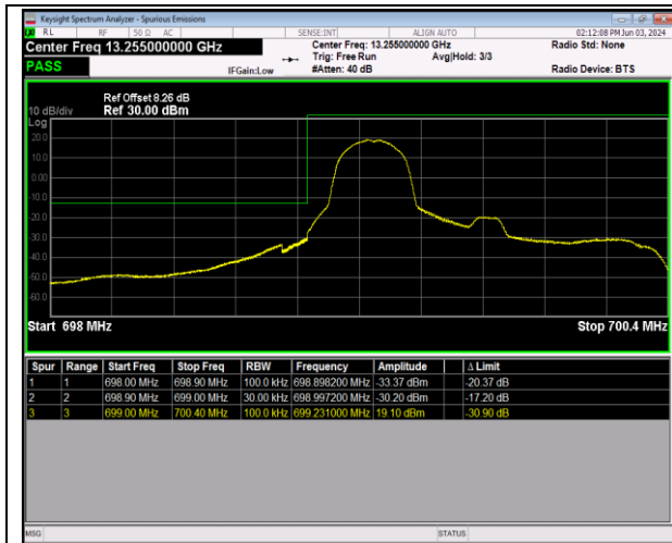
Band12_1.4MHz_QPSK_23017_1RB#0
