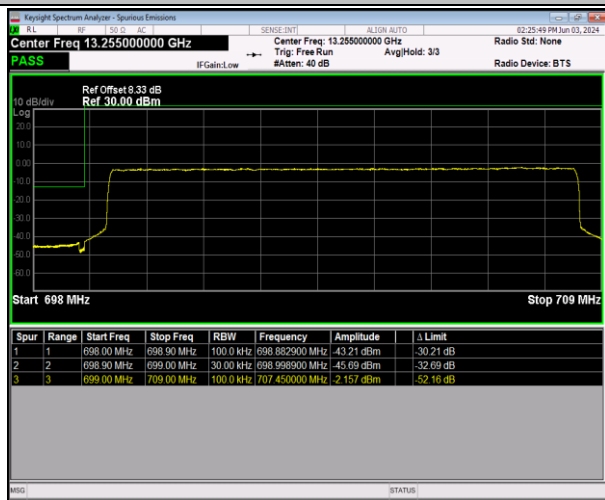
Band12_10MHz_64QAM_23060_50RB#0
