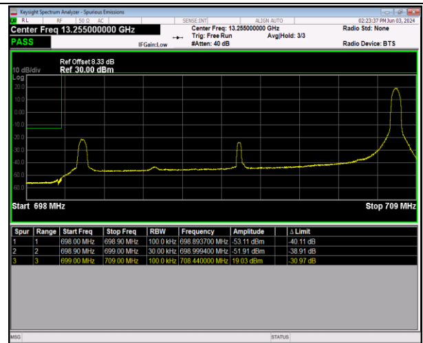
Band12_10MHz_QPSK_23060_1RB#49
