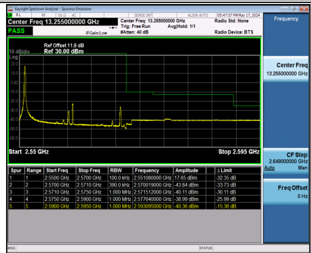
Band7_20MHz_64QAM_21350_1RB#0
