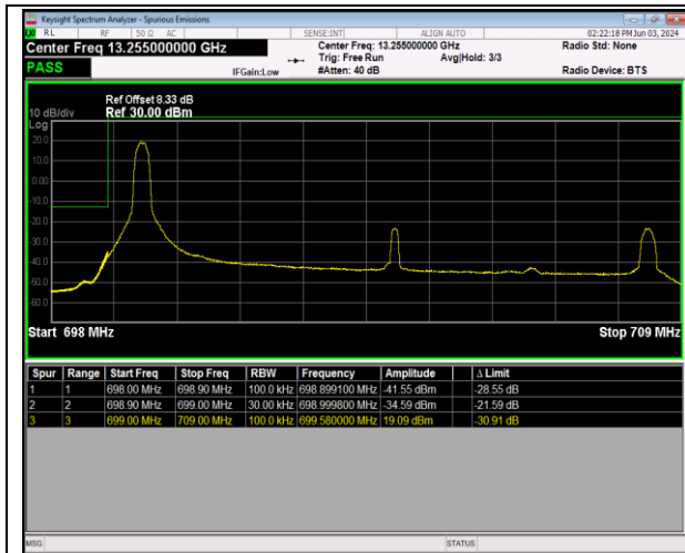
Band12_10MHz_QPSK_23060_1RB#0
